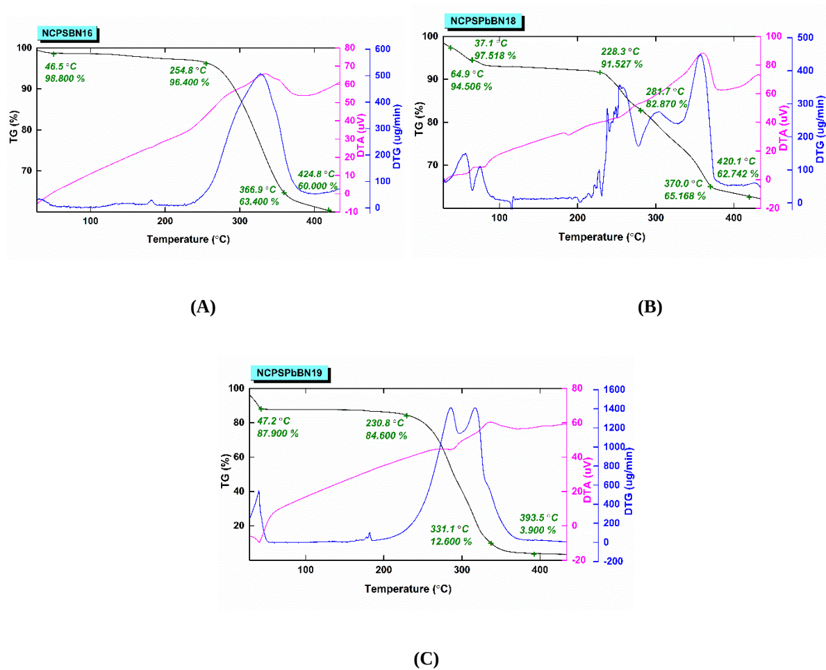
Figure S2. TGA thermograms of the PCM nanocomposites: (A) NCPSBN16, (B) NCPSPbBN18, (C) NCPSPbBN19.
