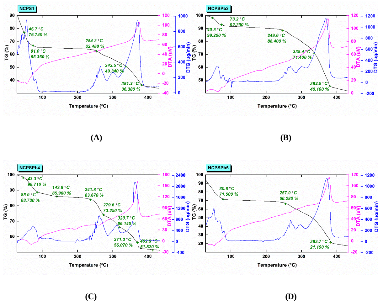
Figure S1. TGA thermograms of the PCM nanocomposites: (A) NCPS1, (B) NCPSPb2, (C) NCPSPb4, (D) NCPSPb5.
