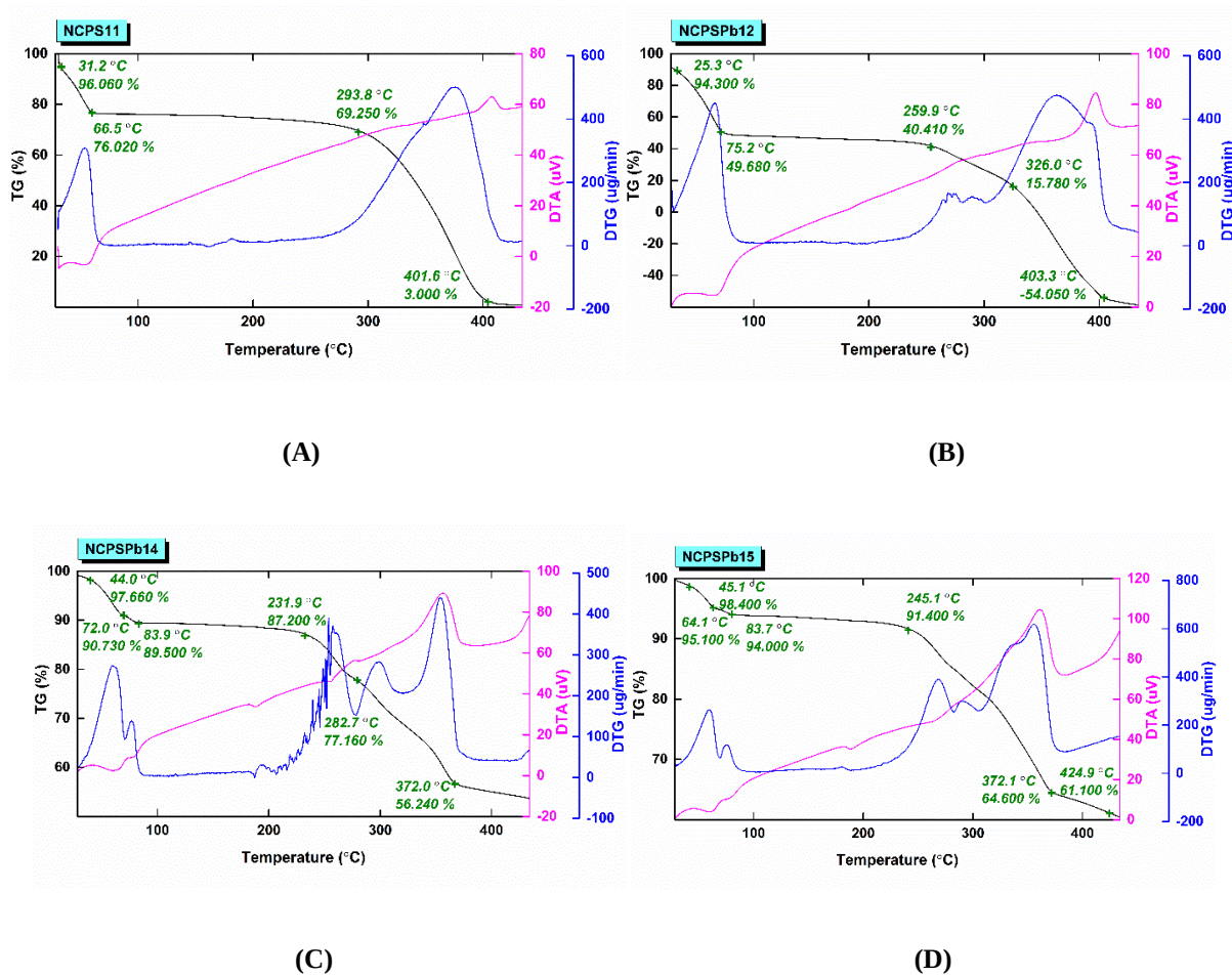
Figure S5. TGAs of researched PCMs: (A) NCPS11, (B) NCPSPb12, (C) NCPSPb14 (D) NCPSPb15.
