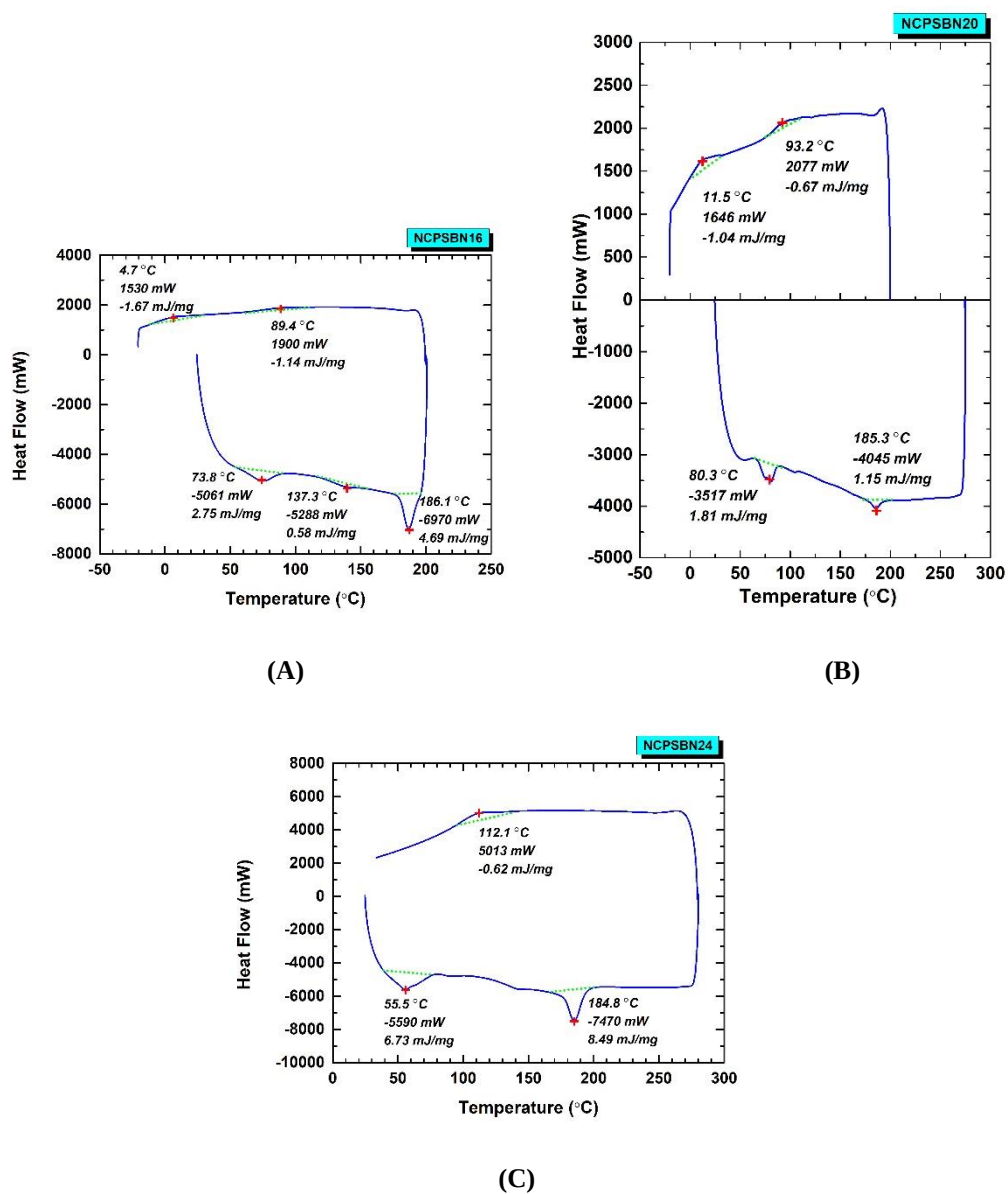
Figure S8. Thermal behavior of PS-PEG PCM Nanocomposites: (A) NCPSBN16, (B) NCPSBN20, (C) NCPSBN24
