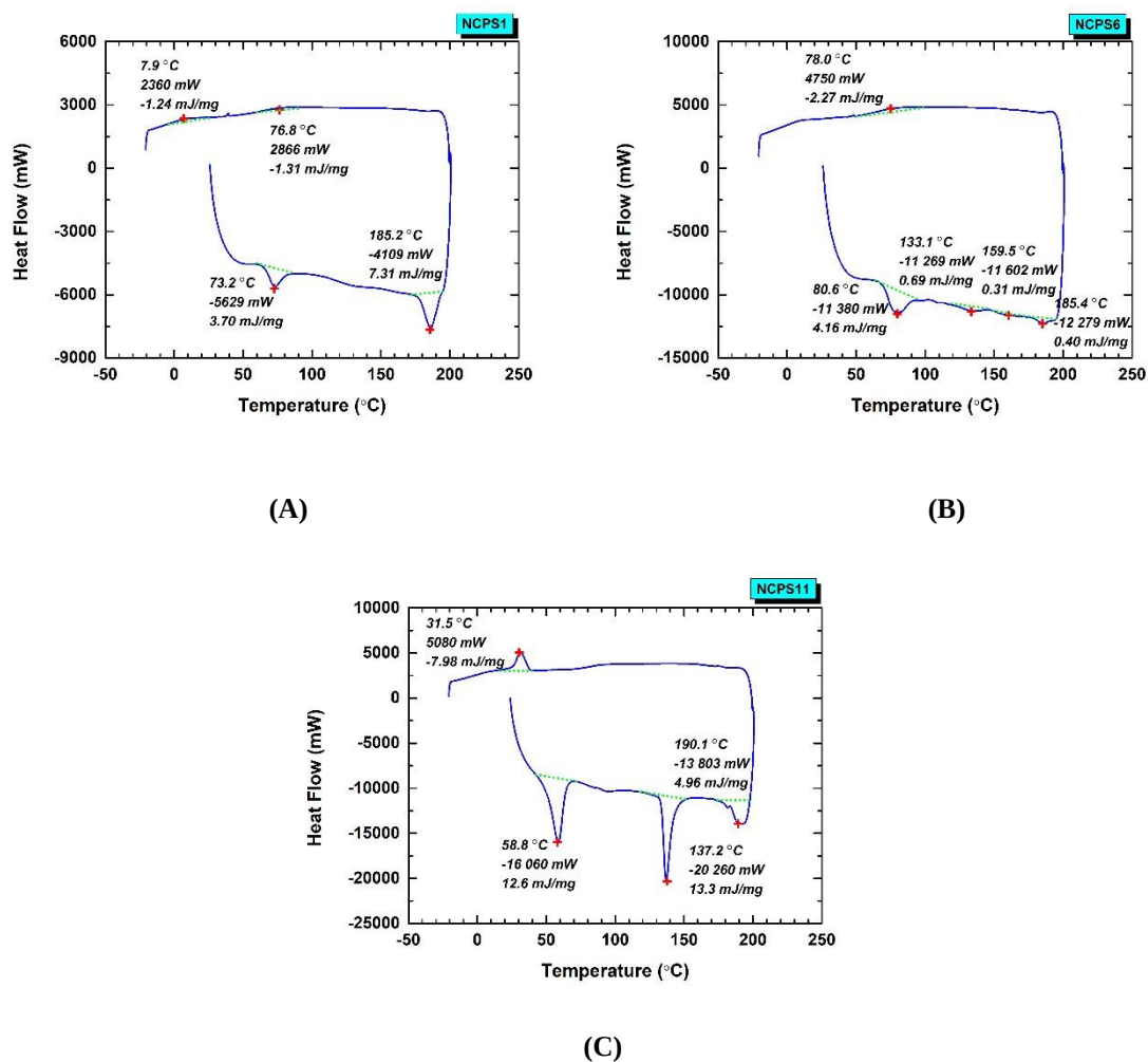
Figure S7. Thermal behavior of PS-PEG PCMs: (A) NCPS1, (B) NCPS6, (C) NCPS11
