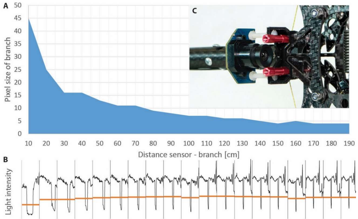
Fig. S6. Branch detection sensor.
