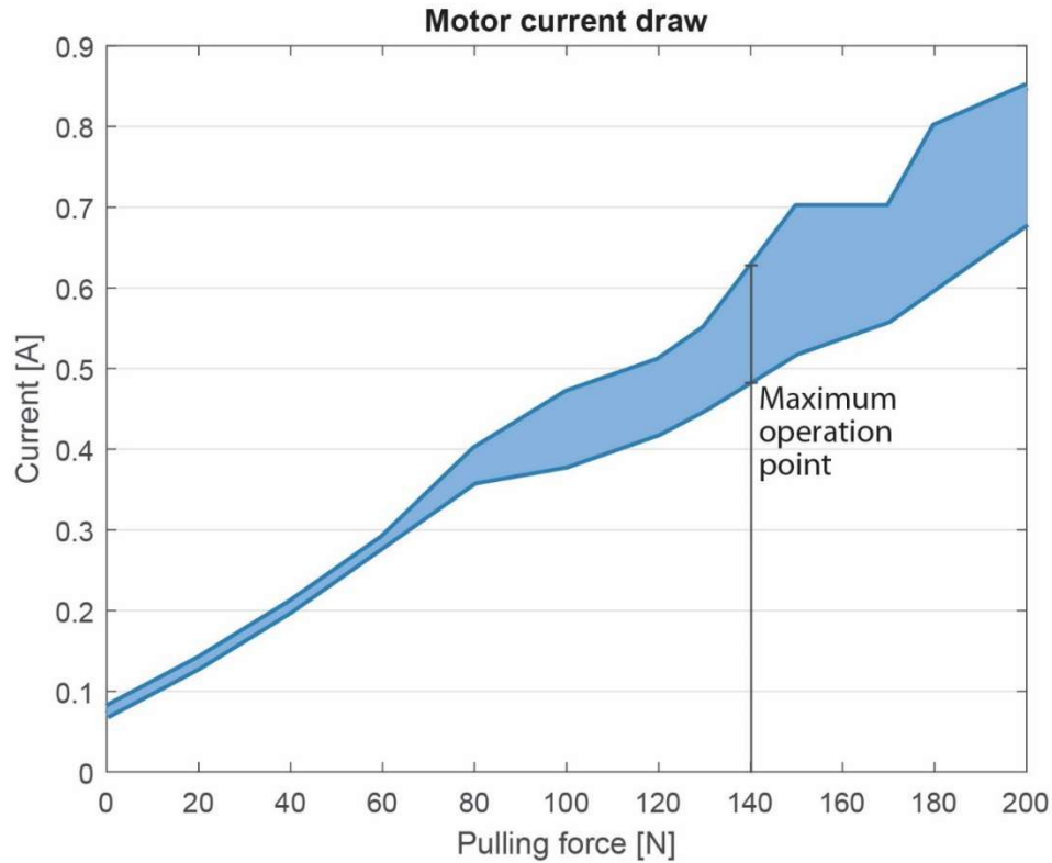
Fig. S1. Re-opening system tension test.
