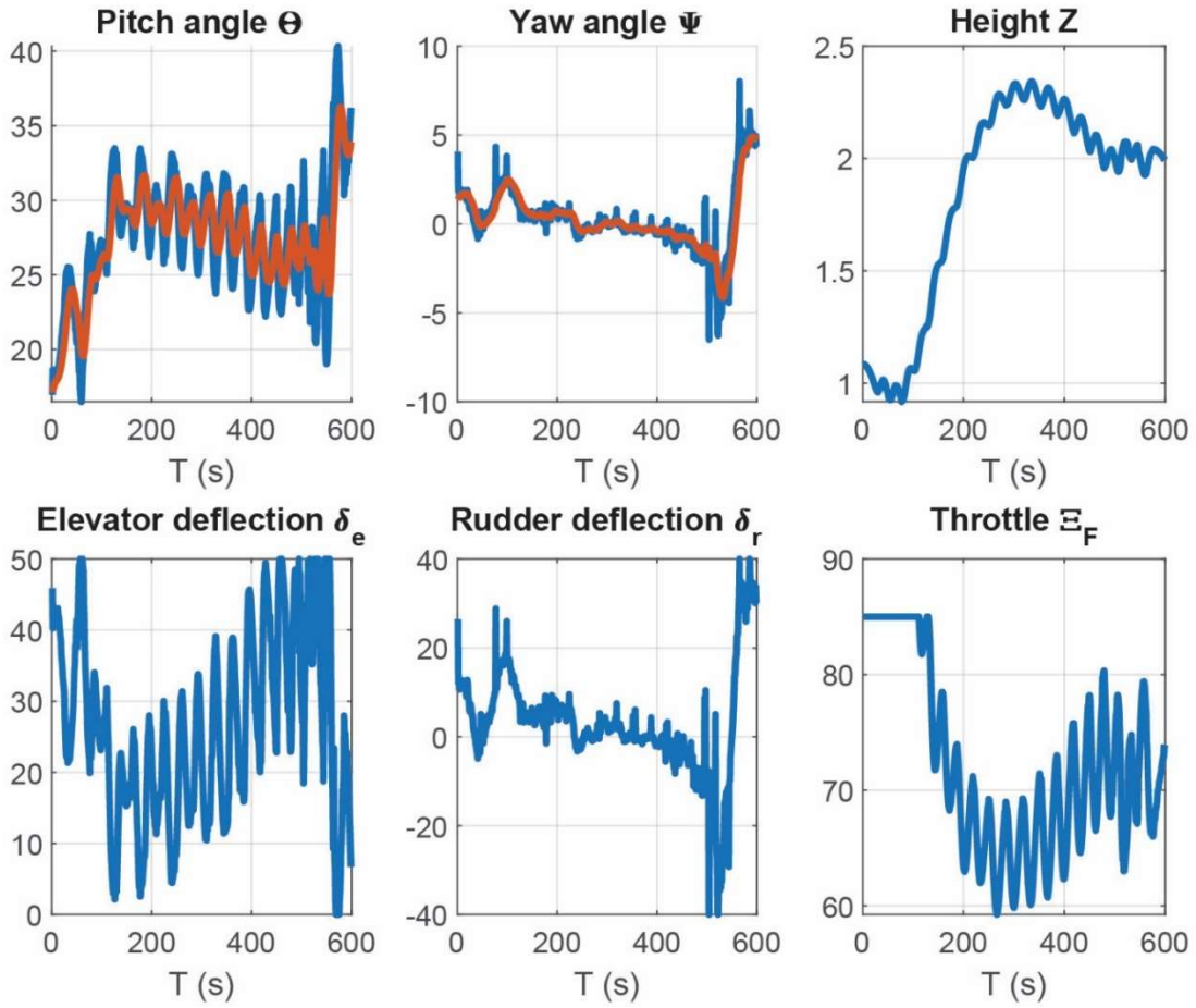
Fig. S7. Control actions.
