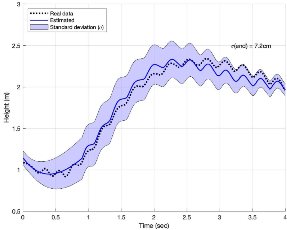
Fig. S17. Model response vs real response in typical flight.
