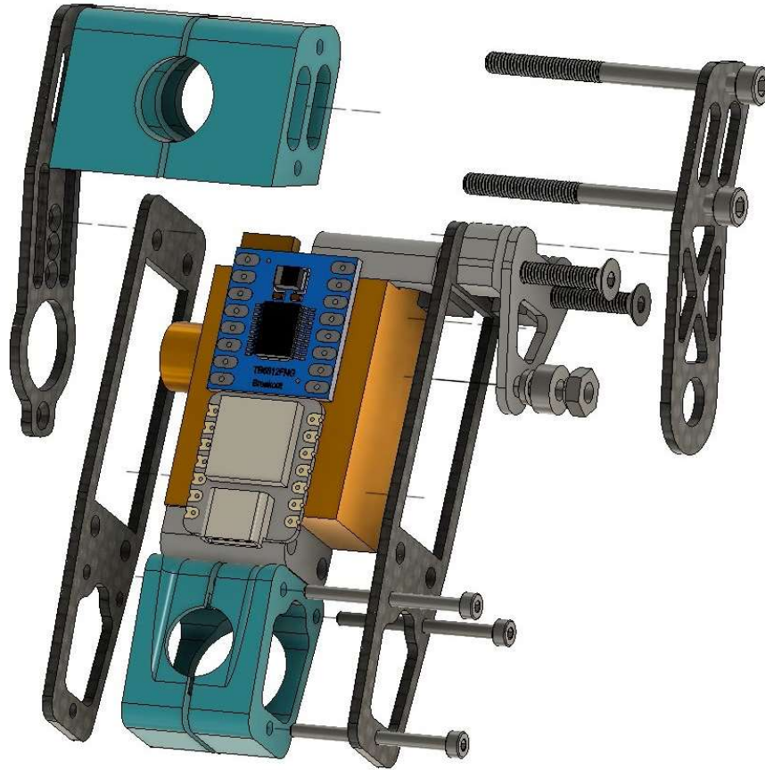
Fig. S13. Leg exploded view.
