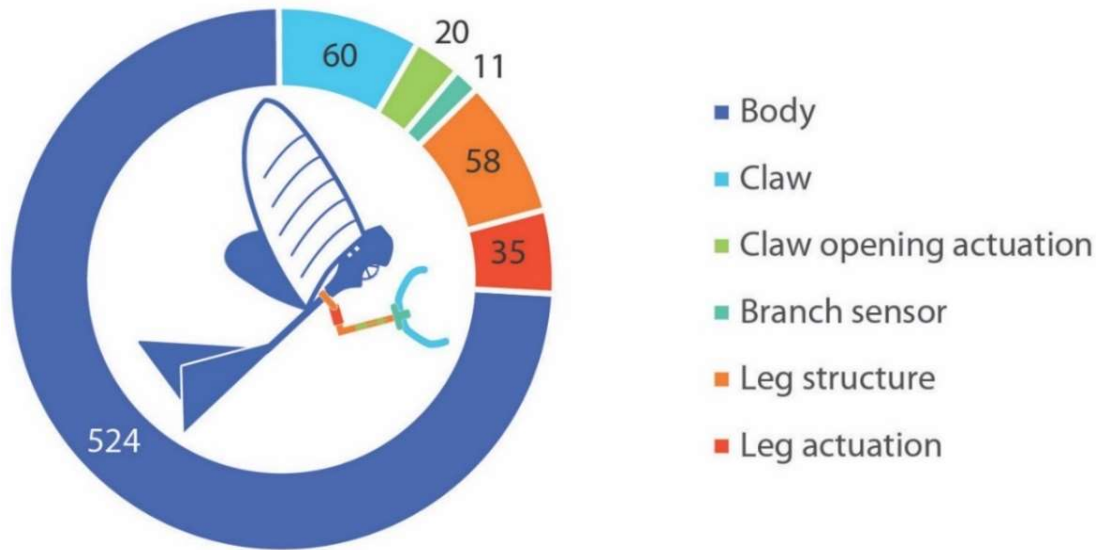
Fig. S9. Payload breakdown.
