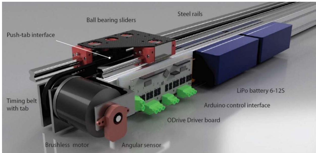
Fig. S10. Launcher assembly.
