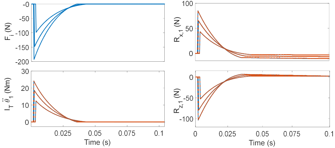
Fig. S4. Validation of the analytical model.
