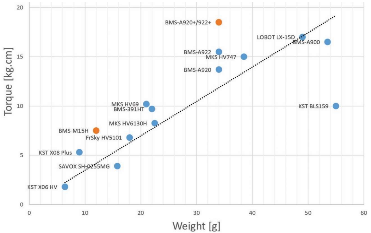
Fig. S2. Servo actuator comparison.
