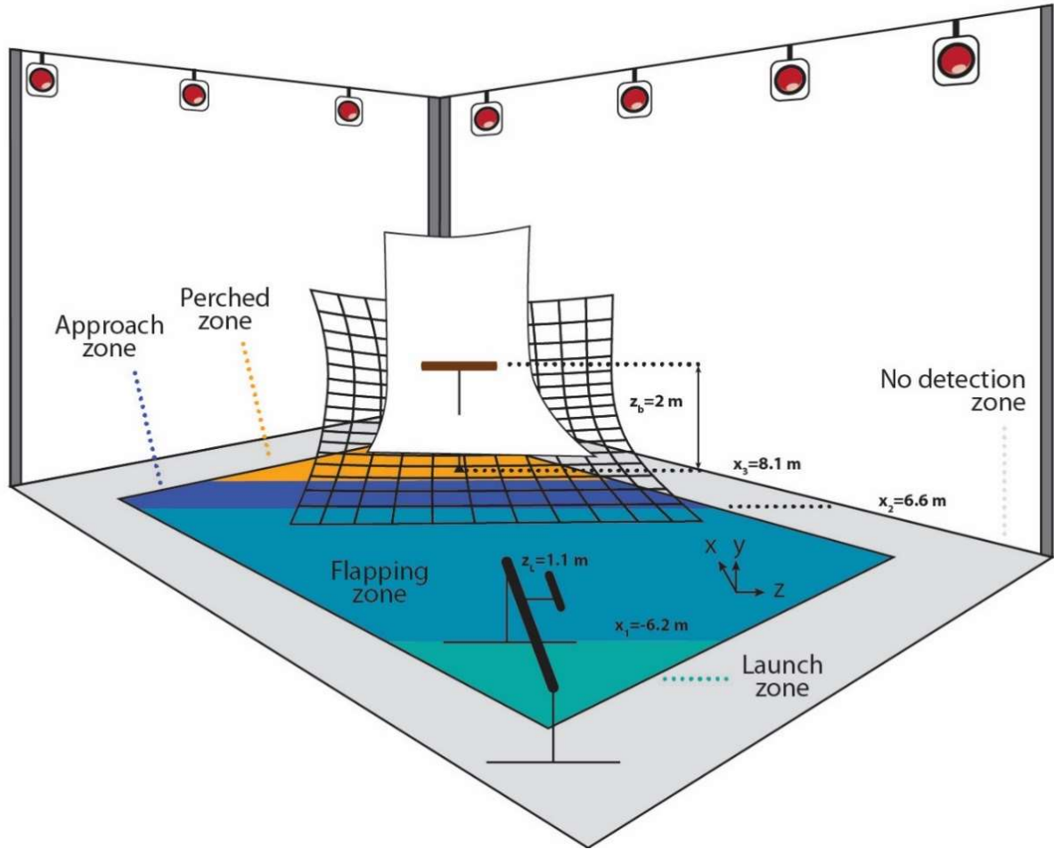
Fig. S8. Flight experiment setup.
