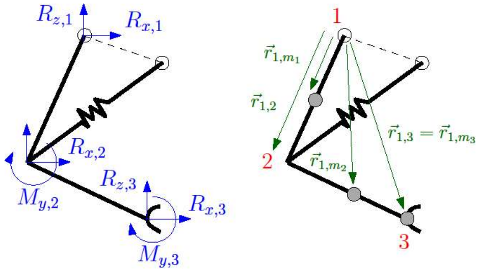
Fig. S3. Schematic of the leg with the hip joint.
