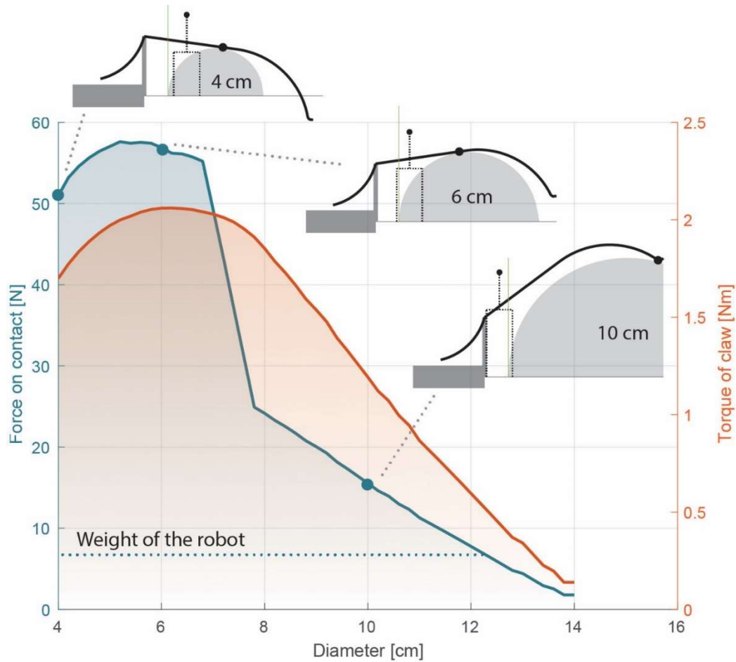
Fig. S16. Branch diameter parametric analysis.
