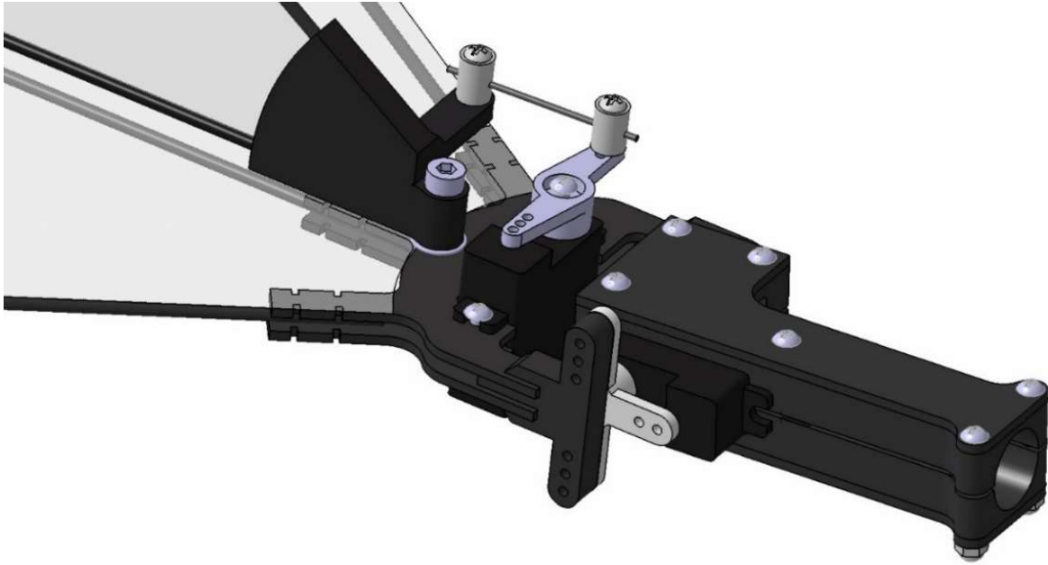
Fig. S14. Tail assembly view.
