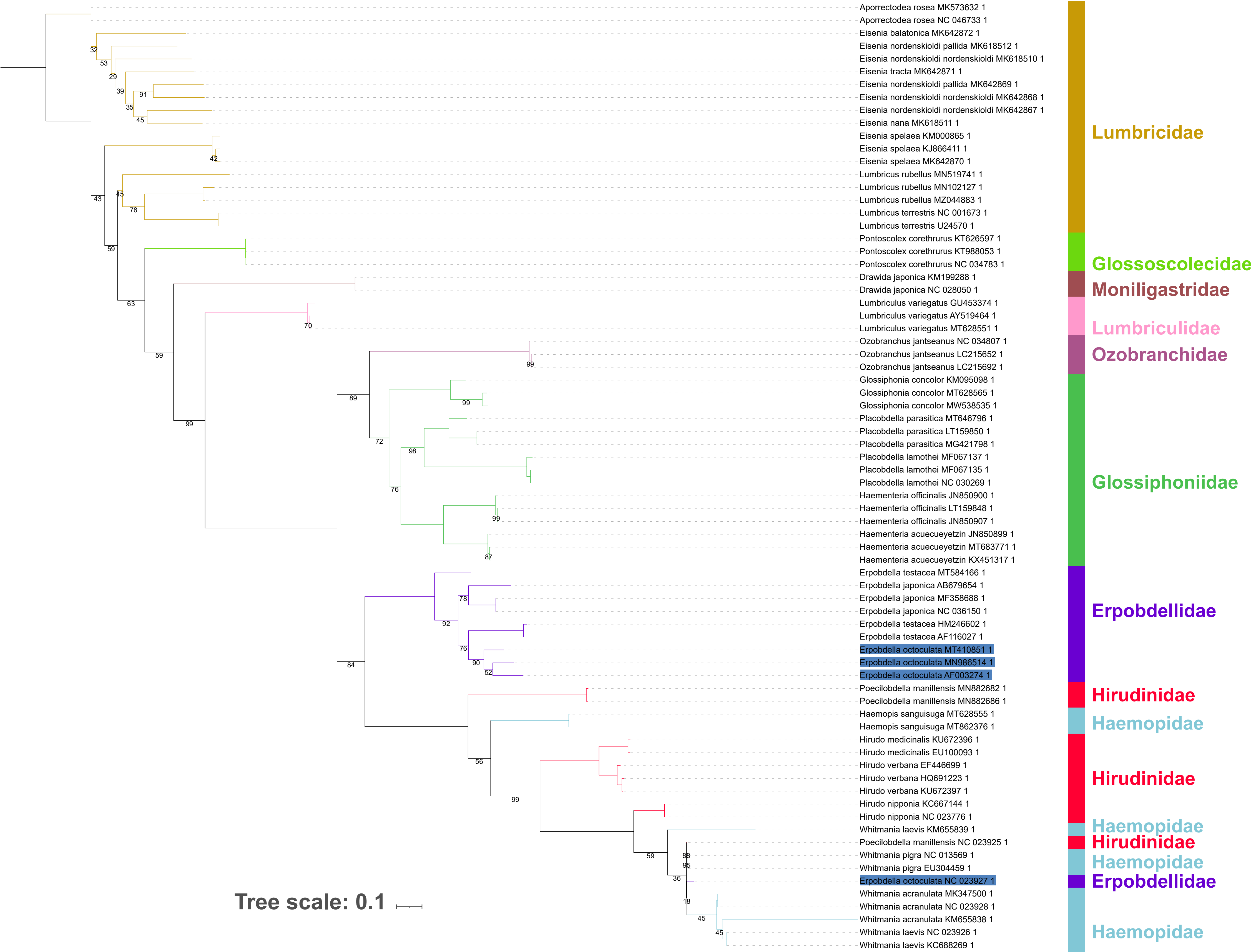
Additional file 13. Phylogeny of all Clitellata species from the 174 mitogenomes dataset, minus the Megascolidae. The phylogram was inferred using the cox1 gene and RAXML. The figure shows (from left to right): a tree with bootstrap values < 100% shown at nodes, species names and taxonomy (family).
