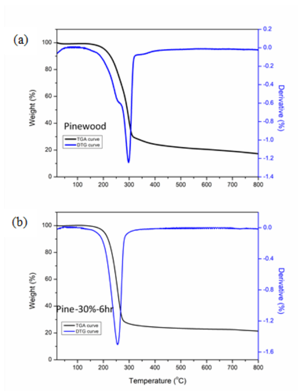
Fig. S2 TGA and DTG curves of (a) Pine-0hr, (b) Pine-30%-6hr product
