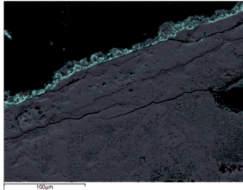
Supplementary Fig. 1 Si-rich layer above the pictorial layer in the sample TBE 5
