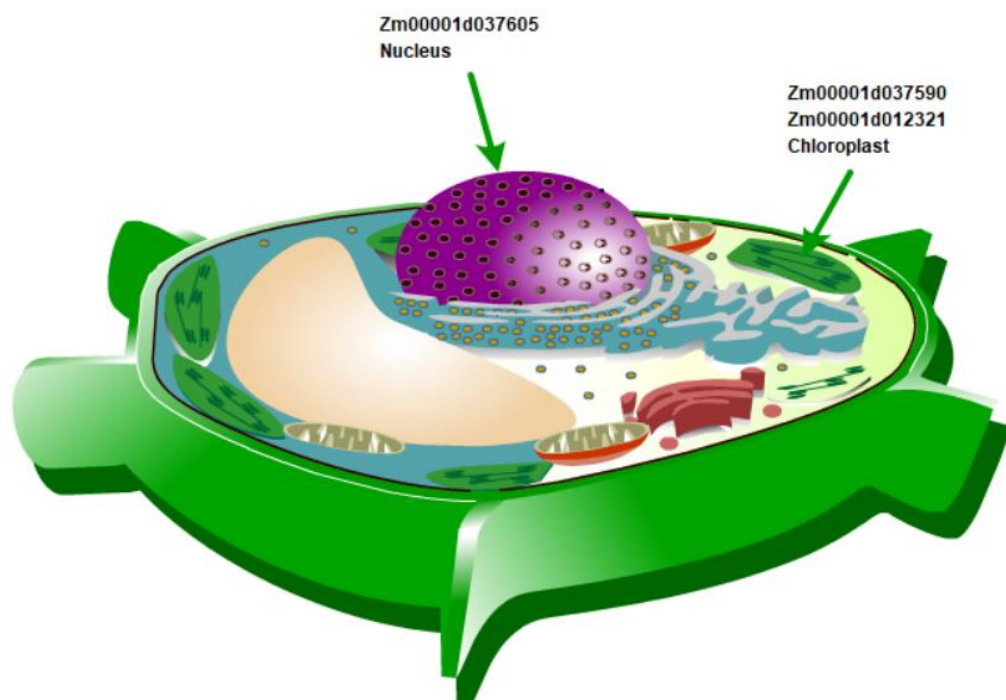
Figure S11 Prediction of subcellular localization of core genes
