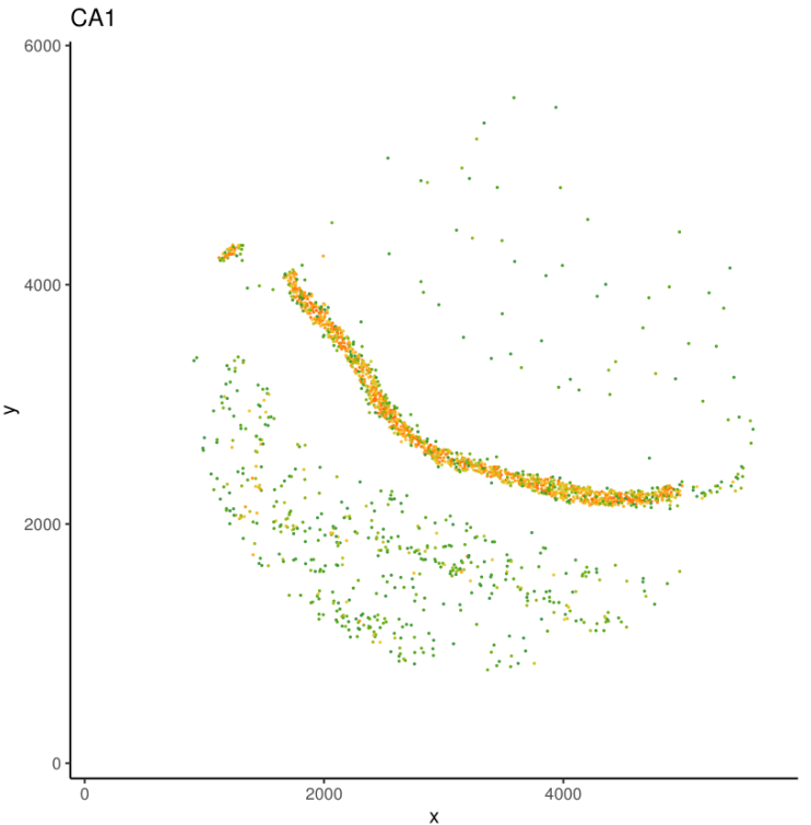
scCapsNet-mask
