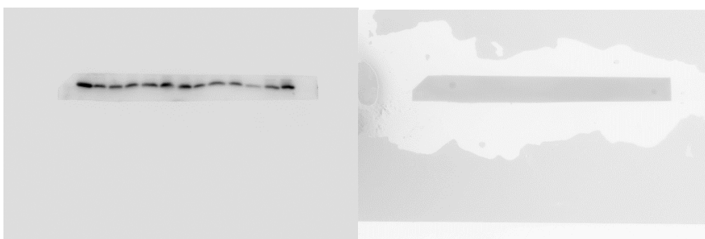
16. Figure5-HIF-1 \alpha -W
