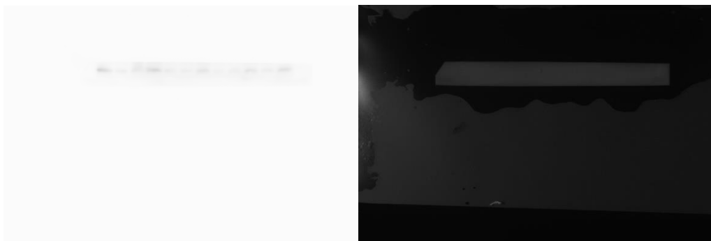
13. Figure4- \beta -actin (down)
