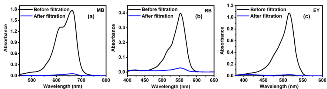
Fig. S4 UV-Vis absorption spectra of (a) MB, (b) RB and (c) EY before and after filtration with nanocomposite membrane
