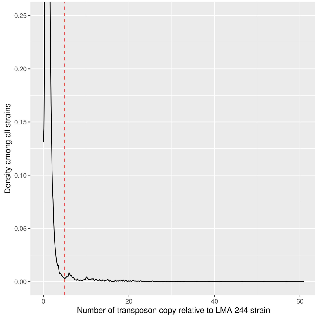
Figure S5: Density of transposable elements copy number relative to the LMA-244 strain To better show the fat tail distribution, the y-axis (density) was cut at 25%. A red dashed line indicates the threshold of five times more copy number than the LMA-244 strain. This threshold was set to identify repeats expansion related to small peaks on the density curve
