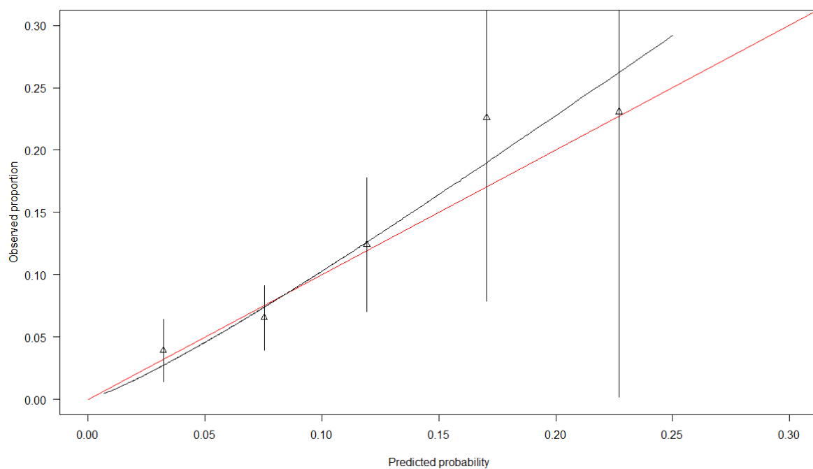
Supplementary Figure 8: Internal validation. Calibration plot (expected vs predicted probabilities) for M3
