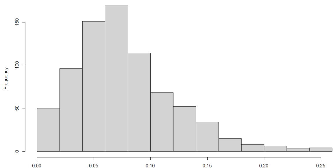
Supplementary Figure 4: Internal validation. Distribution of predicted probabilities for the main model – LASSO
