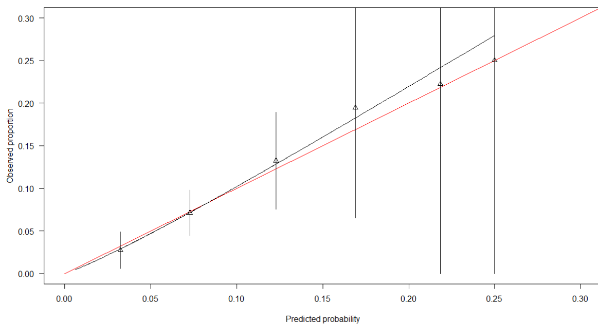
Supplementary Figure 10: Internal validation. Calibration plot (expected vs predicted probabilities) for M4
