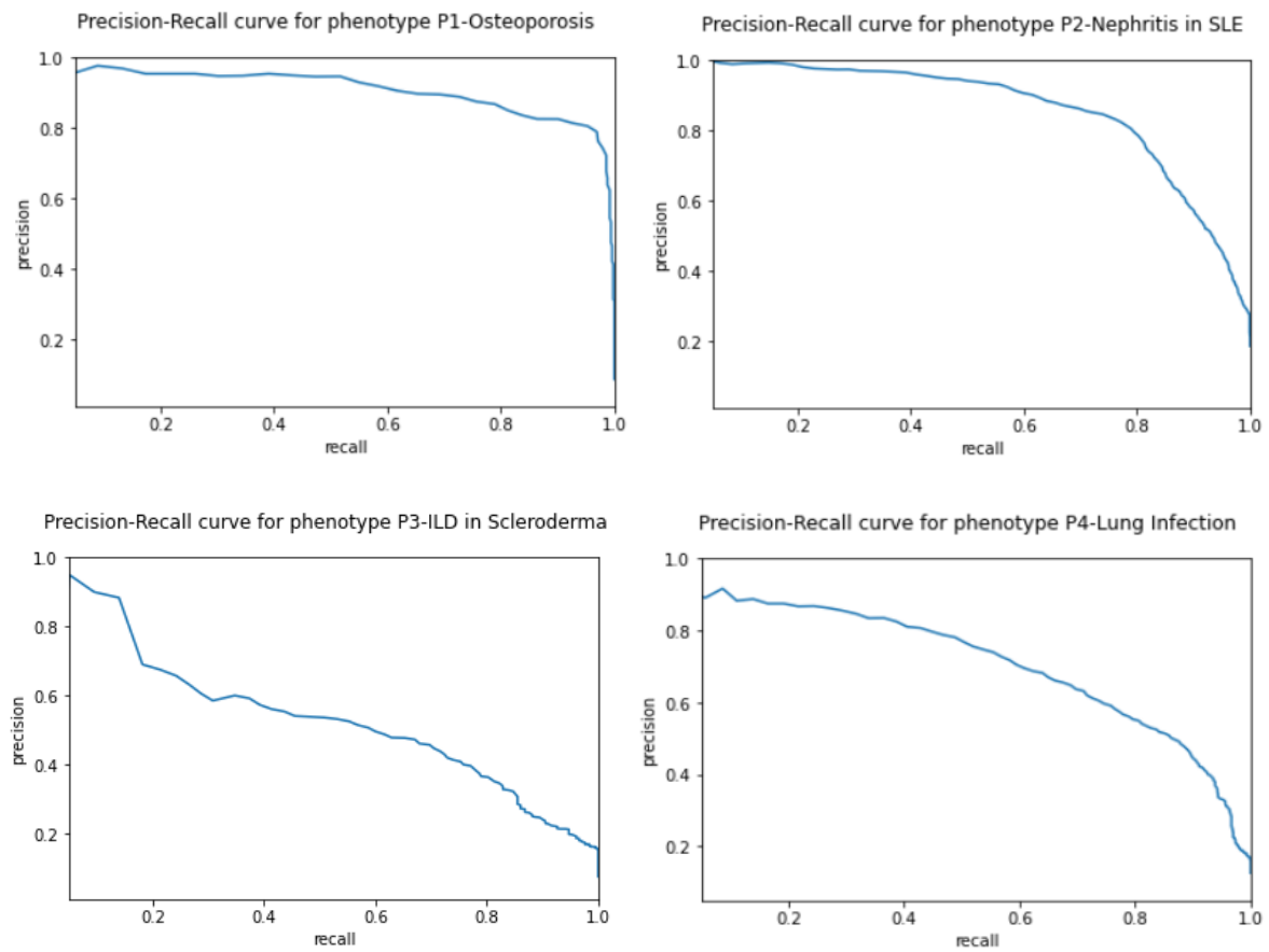
Figure 9: Precision-Recall curves for the four phenotypes
