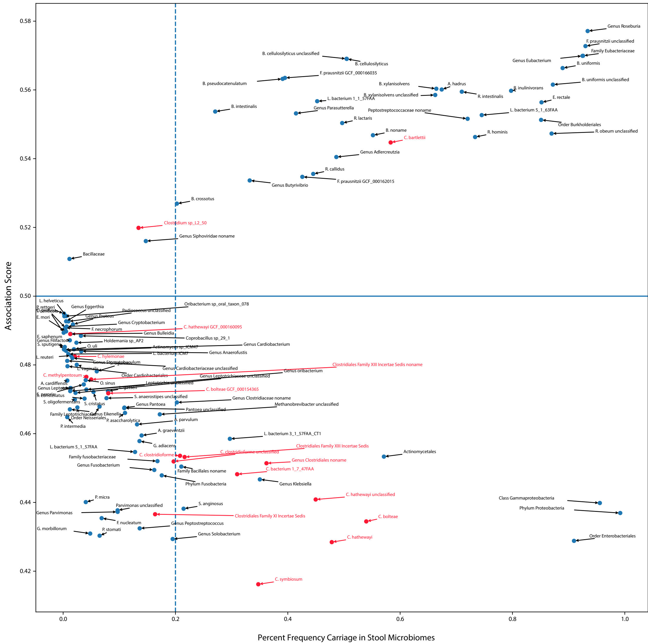
Association Score Vs. Percent Frequency Carriage in Stool Microbiomes
