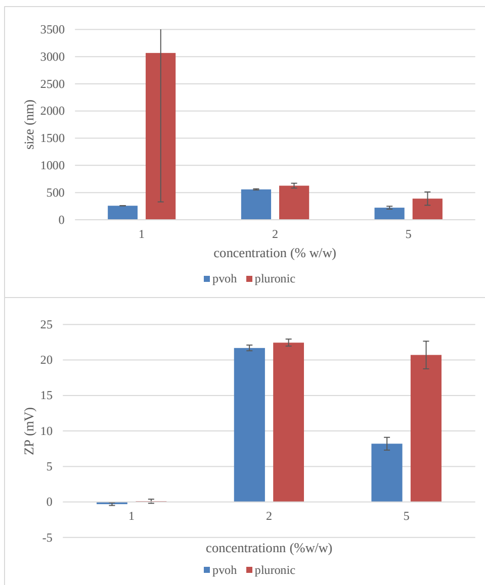
Figure 1S. The effect of concentration of stabilizers on the initial NP size (top) and zeta potential (bottom).
