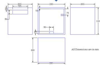
2D Design of Gas Analyser Chamber
