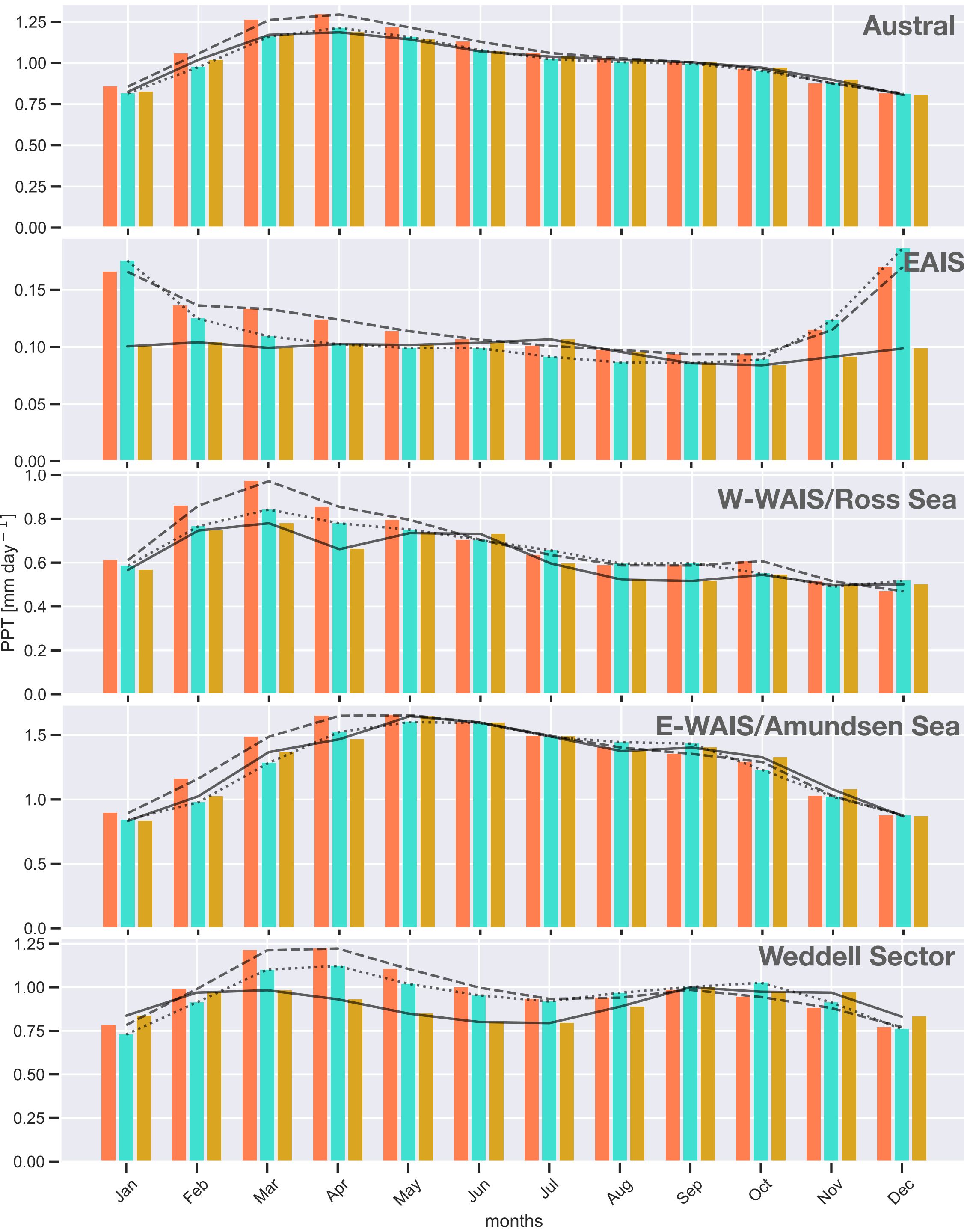
A. Seasonal cycle comparison
