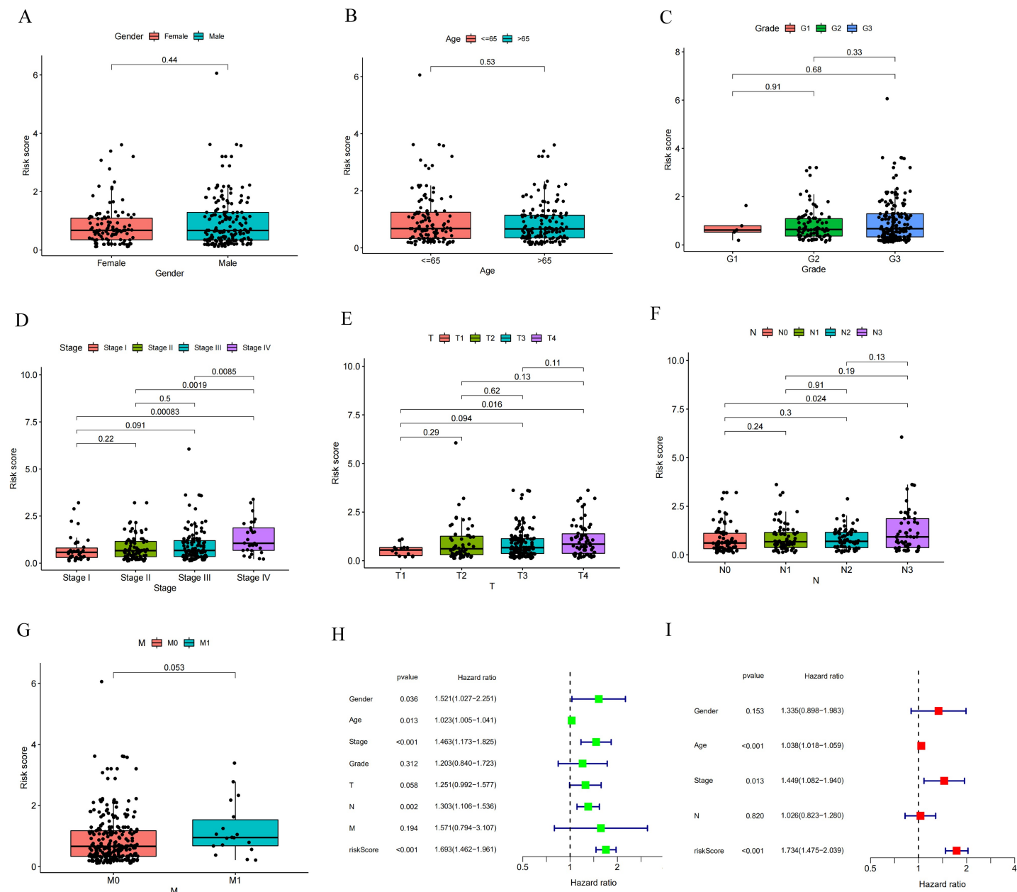
Supplementary Figure 1: Spearman correlation analysis between risk score and clinical features included gender (A), age (B), grade (C), pathological stage (D), T stage (E), N stage (F), M stage (G). Gender, age, stage, and risk score were all found to be independent predictive variables in univariate regression analysis (H). Age, stage, and risk score were all found to be independent predictive variables in multivariate regression analysis (I).
