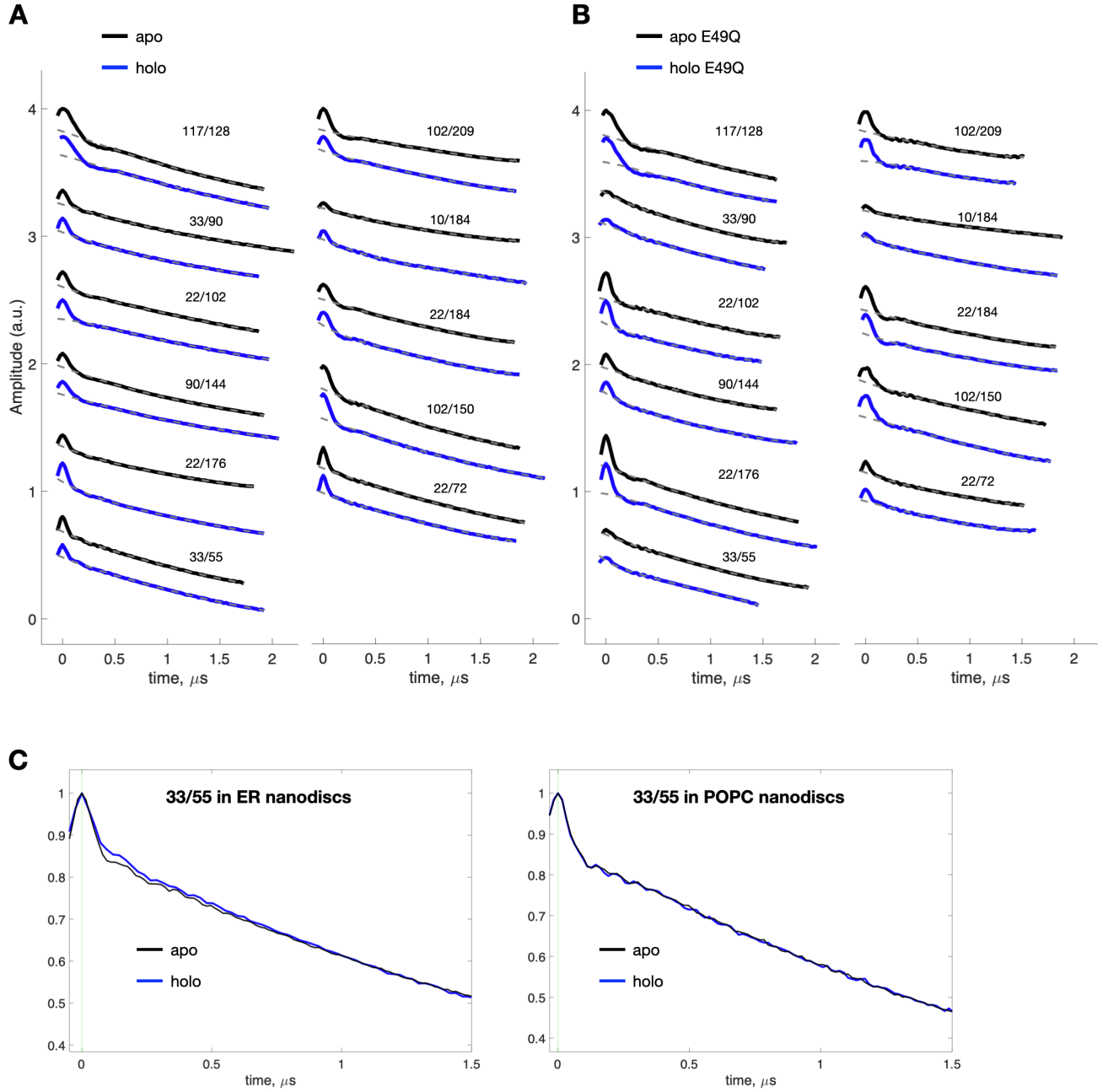
Figure S2. DEER measurements of spin-labeled BsYetJ in apo and holo states. (A) Primary DEER traces of the spin-labeled BsYetJ variants. (B) Primary DEER traces of the spin-labeled BsYetJ E49Q variants. (C) A close-up view on the DEER traces of 33/55. Left: shown are raw DEER traces of apo and holo 33/55 in ER nanodiscs. There are small but significant differences in the DEER traces, providing evidence for the differences in the distance distributions obtained in the Tikhonov analysis (Fig. 2C). We repeated the measurements to verify the reproducibility. Right: shown are raw DEER traces of apo and holo 33/55 reconstituted in pure POPC nanodiscs. The two DEER traces overlap well with
