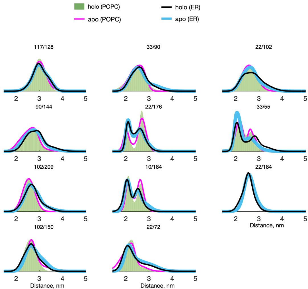
Figure S3. A comparison of the DEER results obtained in different lipid environments.
