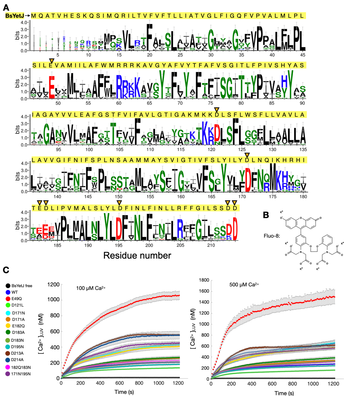
Figure S1. Information about the sequence analysis and the Fluo-8 molecule. (A) Sequence conservation of selected amino acids in BsYetJ. Totally 30 homologous sequences with more than 50% similarity are collected using HMMER search against UNIREF90 database by ConSurf web server ( http://consurf.tau.ac.il/ ) (Ashkenazy et al., 2016, 2010). Multiple Sequence Alignment was built using MAFFT and the conservation was depicted using WebLogo ( http://weblogo.threeplusone.com/create.cgi ) (Crooks et al., 2004). Conservation is measured in bits, each residue height shows the degree of conservation, and
