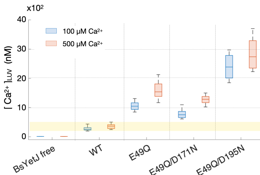
Figure S6. Calcium influx activity of E49Q/D171N and E49Q/D195N. To support our hypothesis that D171- or D195-associated sites act as a minor selectivity filter than E49 in controlling the calcium influx activity, we performed the calcium activity assay on two BsYetJ variants, E49Q/D171N and E49Q/D195N, each having two mutations at their two respective selectivity filters proposed in the present study. For a convenient comparison of the activity, we also provide the results of BsYetJ-free, WT, and E49Q in the present plot. We found that [Ca^{2+}]_{LUV} of E49Q/D171N is comparable to that of E49Q, but E49Q/D195N has a distinctly greater [Ca^{2+}]_{LUV} than all other BsYetJ. As D195N alone is not sufficient to cause a large change in [Ca^{2+}]_{LUV} (shown in Fig. 1D), our results here demonstrate that D195 acts as a relatively minor selectivity filter than E49 in determining the calcium influx activity and that D195 is more important than D171 in controlling the calcium influx activity of the minor selectivity filter.
