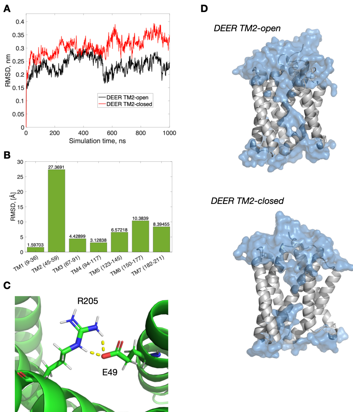
Figure S4. Results of the MD simulations and modeling. (A) RMSD values from the MD simulations to validate the two DEER-derived models, DEER TM2-open and -closed structures. RMSD is calculated from the root mean-square-average distances between C \alpha atoms of two superimposed structures (i.e., the initial and a MD-snapshot structure), providing a quantitative measure of how a modeled structure deviates from the initial structure during MD simulations. Overall, the RMSD values converged rapidly and became approximately constant for at least 600 ns. The converged values are in the range of 0.24 to 0.32 nm, indicating that the final and initial structures are similar. It supports that the initial
