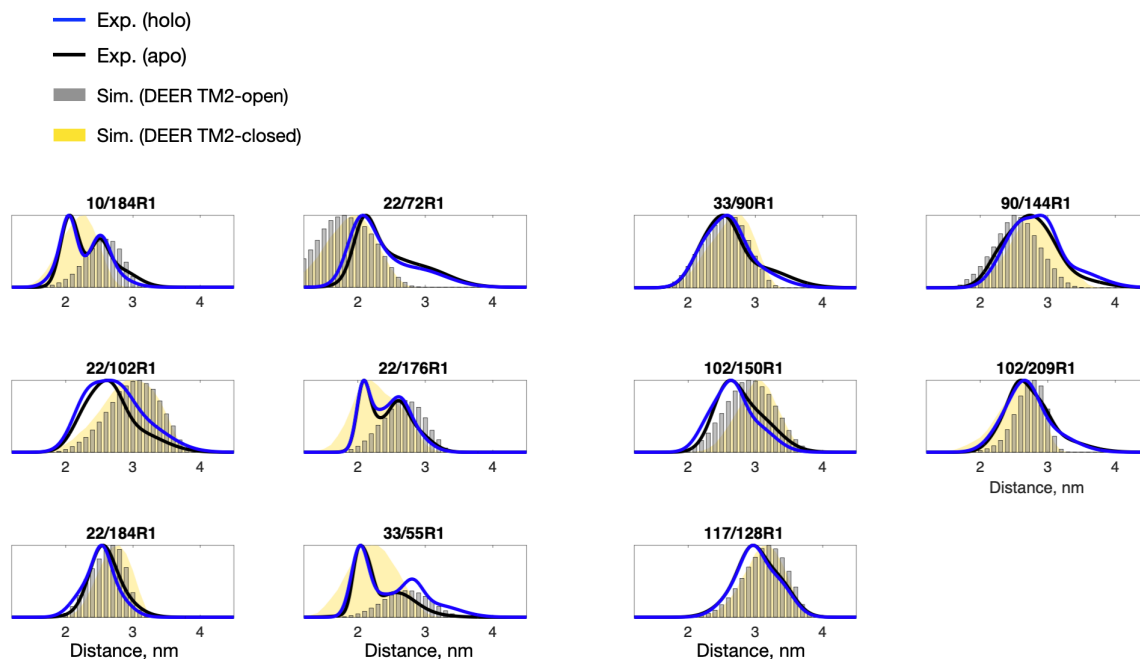
Figure S5. Distance distributions simulated from our DEER-derived models. Based on our DEER-derived models (Fig. 4A), we generated interspin distance distributions for the DEER TM2-open and -closed structures using the MtsslWizard program. The simulations (Sim.) are in a good agreement with the DEER experimental (Exp.) results in both apo and holo states.
