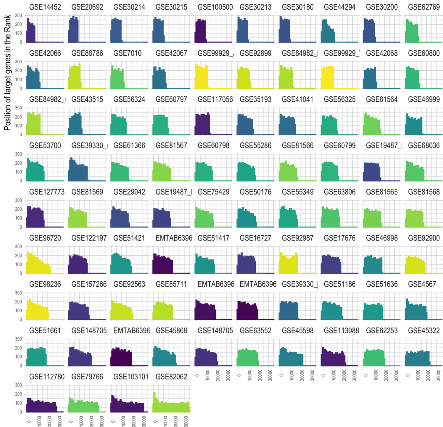
Figure S2: Distribution of the position of the transcripts regulated by the identified transcription factors in each dataset included and excluded from the initial pool of Säärimäki et al. Transcripts are ranked according to the p-value of the detected alteration.
