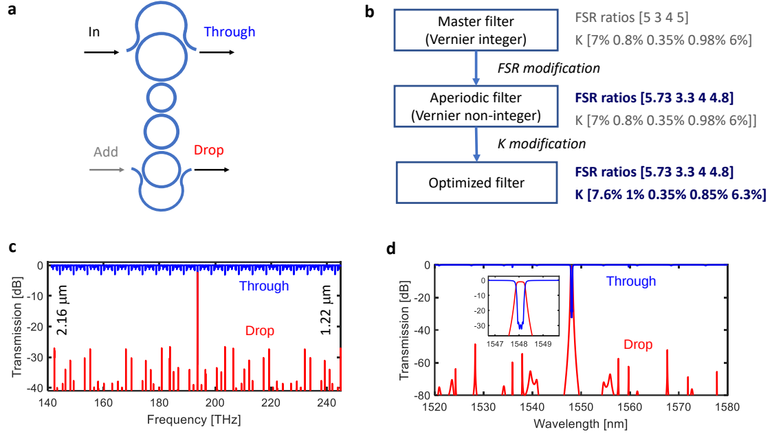
Figure S1: (a) Schematic of 4 th order Vernier filter with two tunable couplers connecting it to input/output bus waveguide. (b) Flowchart of design procedure, with FSRs and couplers values. (c) Through and Drop port simulation of filter designed based on non-integer Vernier scheme neglecting the dependence of coupler on wavelength presenting more than 120THz of FSR. (d) Frequency response of 4 th order filter with 40GHz bandwidth and more than 90nm of FSR.
