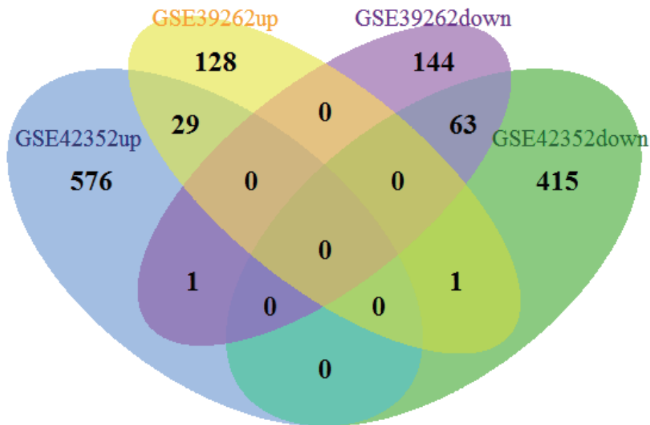
Fig. S1 Identification of DEGs in mRNA expression profiling datasets GSE42352, GSE39262
