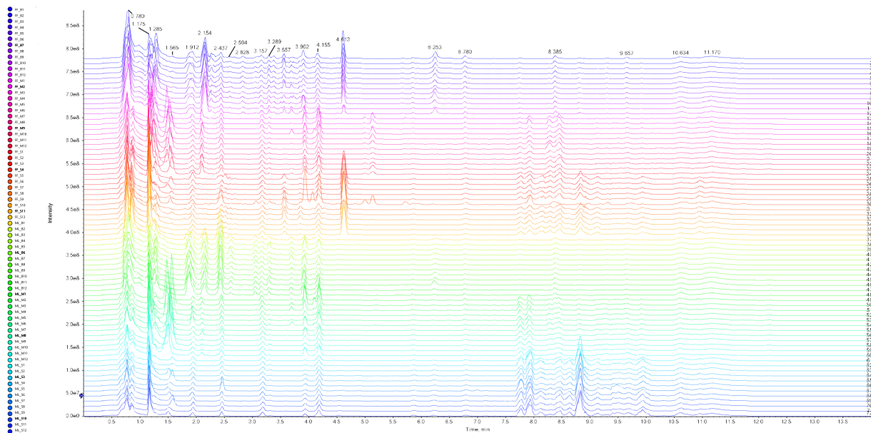
Fig S1. The total ion chromatogram information under positive (a) and negative (b) ion modes.
