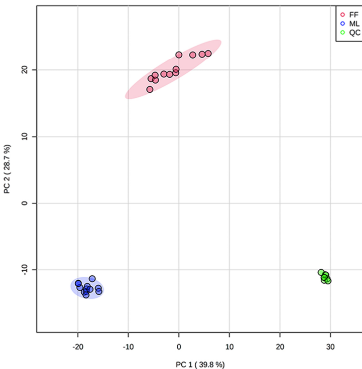
Scores Plot
