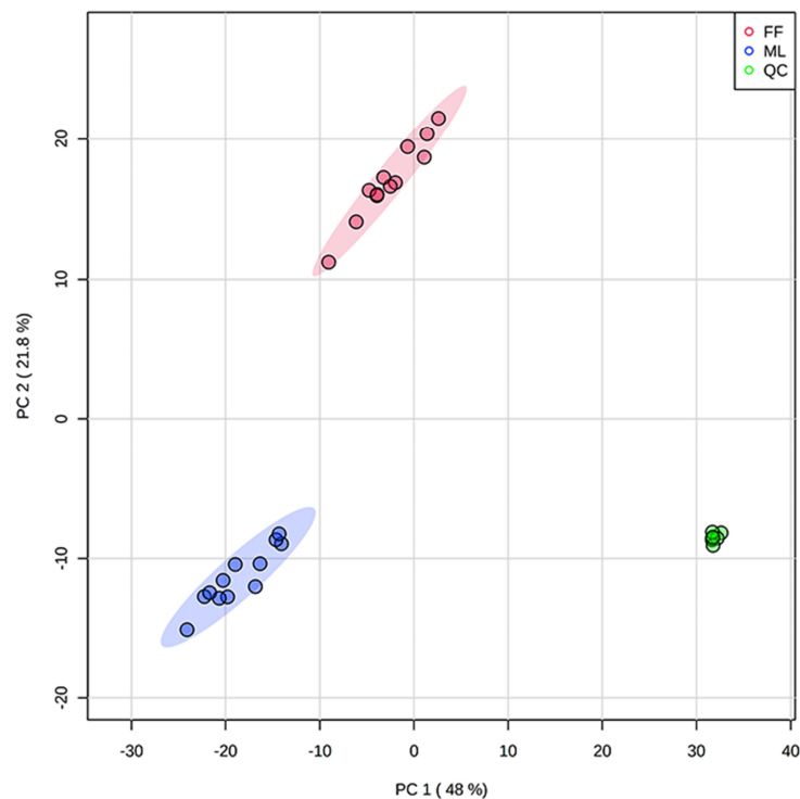
Scores Plot
