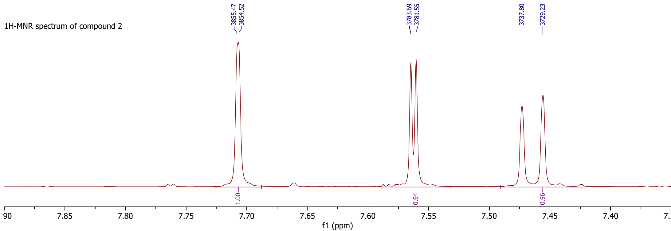
1 H-NMR spectrum of compound 2
