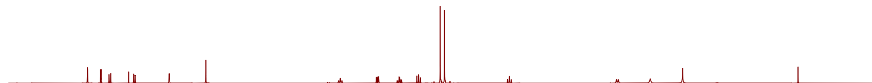
HMBC spectrum of compound 2
