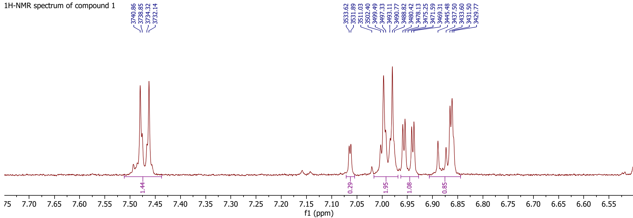
1 H spectrum of compound 1
