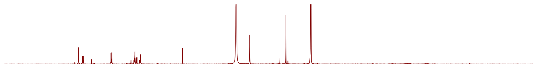
HMBC spectrum of compound 1
