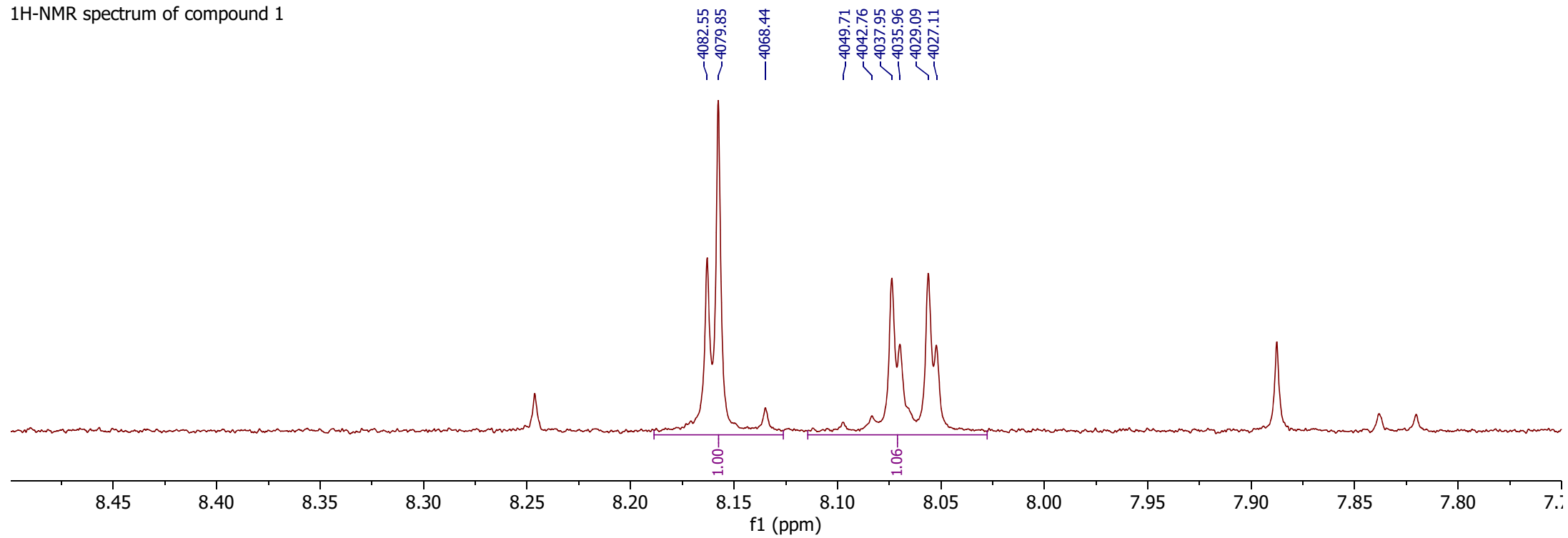
1 H-NMR spectrum of compound 1
