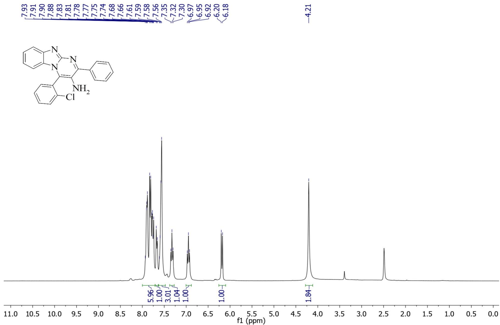
1 H NMR spectrum of 4-(2-chloro-phenyl)-2-phenyl-benzo[4,5]imidazo[1,2-a]pyrimidin-3-ylamine ( 3e )
