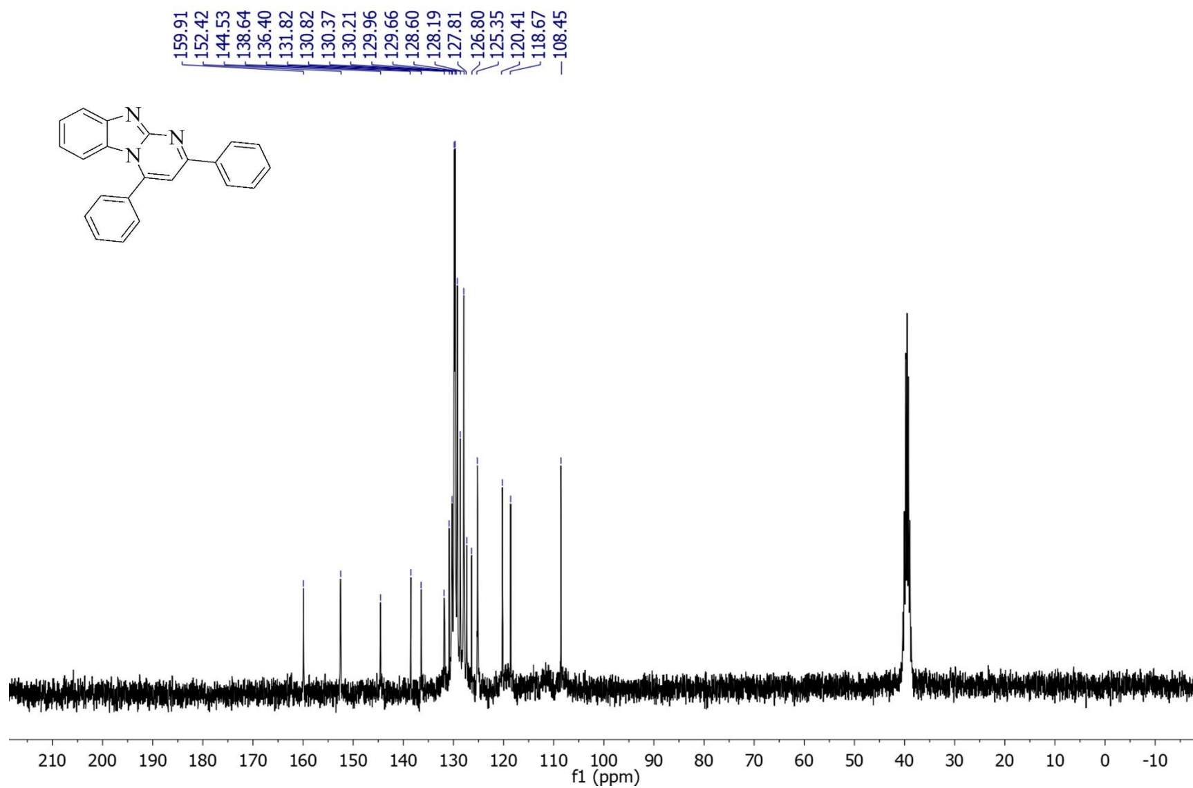
13 C NMR spectrum of 2,4-diphenyl-benzo[4,5]imidazo[1,2-a]pyrimidine ( 6a )
