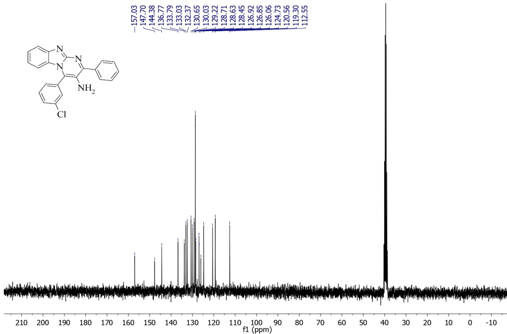
13 C NMR spectrum of 4-(3-chloro-phenyl)-2-phenyl-benzo[4,5]imidazo[1,2-a]pyrimidin-3-ylamine ( 3f )
