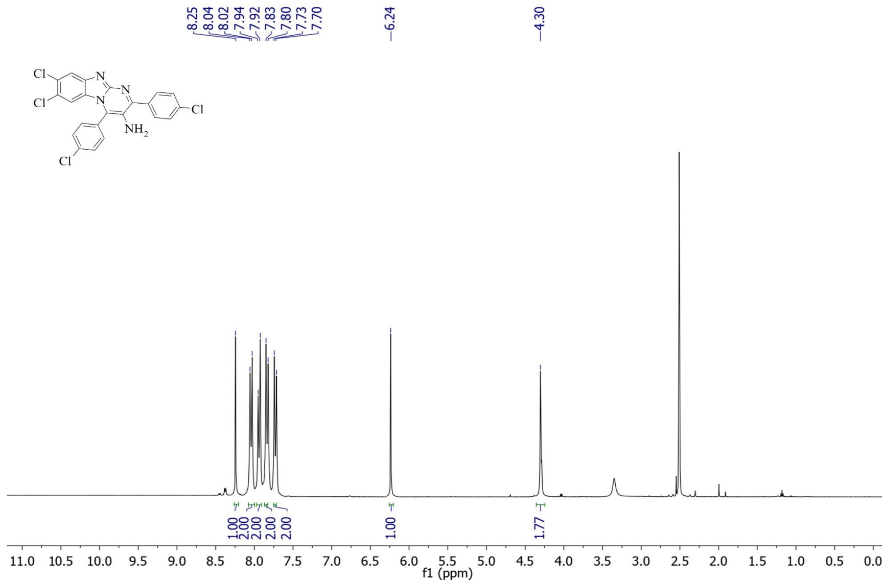
1 H NMR spectrum of 7,8-dichloro-2,4-bis-(4-chloro-phenyl)-benzo[4,5]imidazo[1,2-a]pyrimidin-3-ylamine ( 3ad )
