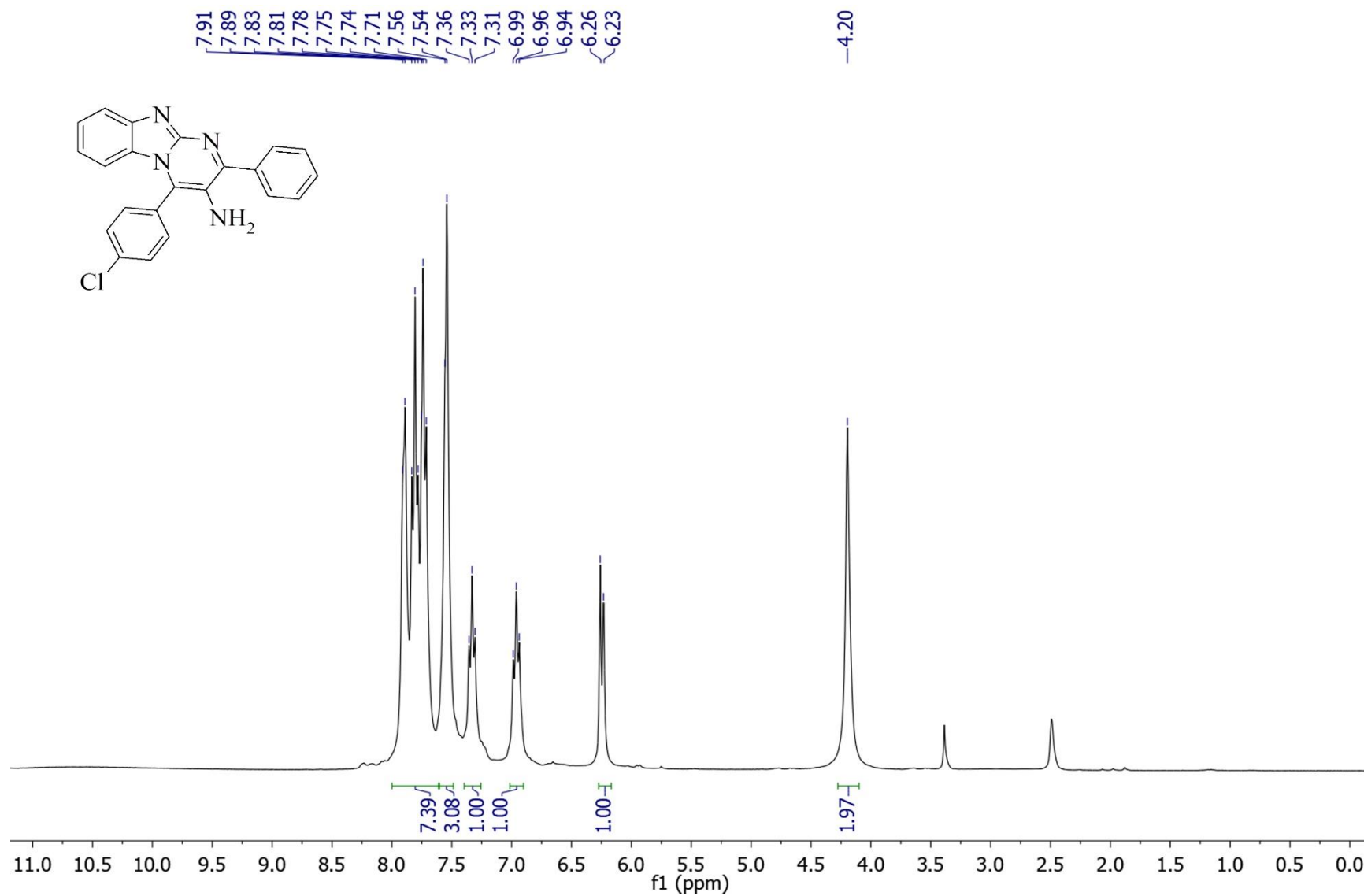
^1\text{H} NMR spectrum of 4-(4-chloro-phenyl)-2-phenyl-benzo[4,5]imidazo[1,2-a]pyrimidin-3-ylamine ( 3d )
