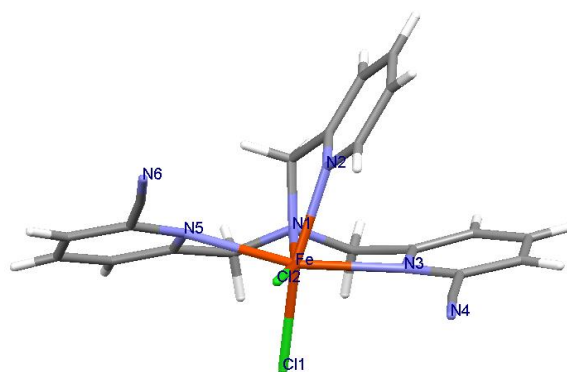
Figure 8: Mercury representation of the (CN) 2 TPAFFeCl 2 complex. The main distances and angles are given in Table 3.
