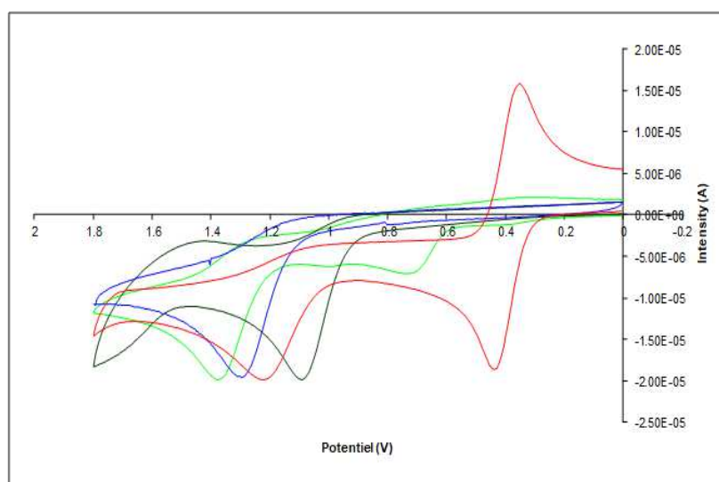
Figure3: Voltammerogram of ligands(TPA; CNTPA; (CN)2TPA;and (CN)3TPA), with TPA in black, CNTPA in red, (CN)2 TPAin blue, (CN)3TPAin green.
