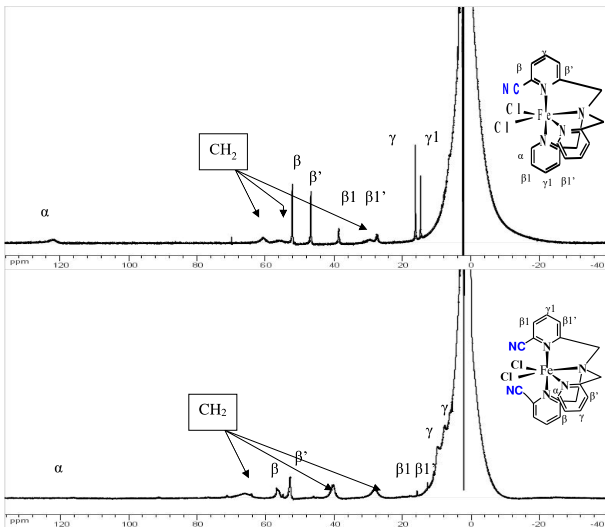
Figure 5: Paramagnetic ^1\text{H} NMR spectrum for the \text{CNTPAFeCl}_2 and (\text{CN})_2\text{TPAFeCl}_2 complexes.
