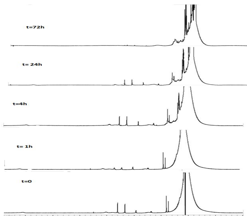
Figure 10: The 1 H NMR spectra, for the oxygenation kinetics of the CNTPAFeCl 2 complex at: a) t = 0, b) t = 1h, c) t = 4h, d) t = 24h, e) t = 72h. The stars correspond to the signals of the traces of the starting product.
