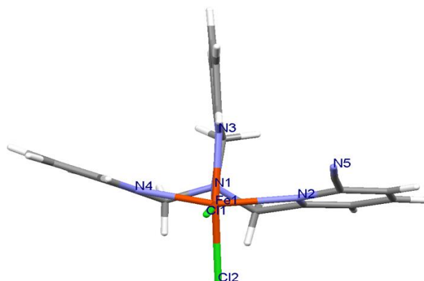
Figure 7: Mercury representation of the \text{CNTPAFeCl}_2 complex. The main distances and angles are given in Table 3.
