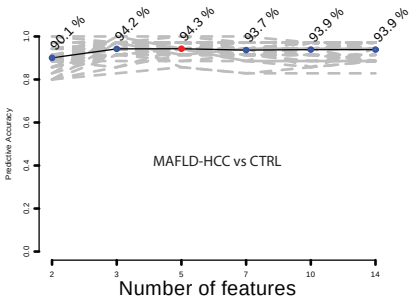
Predictive accuracies with different features
