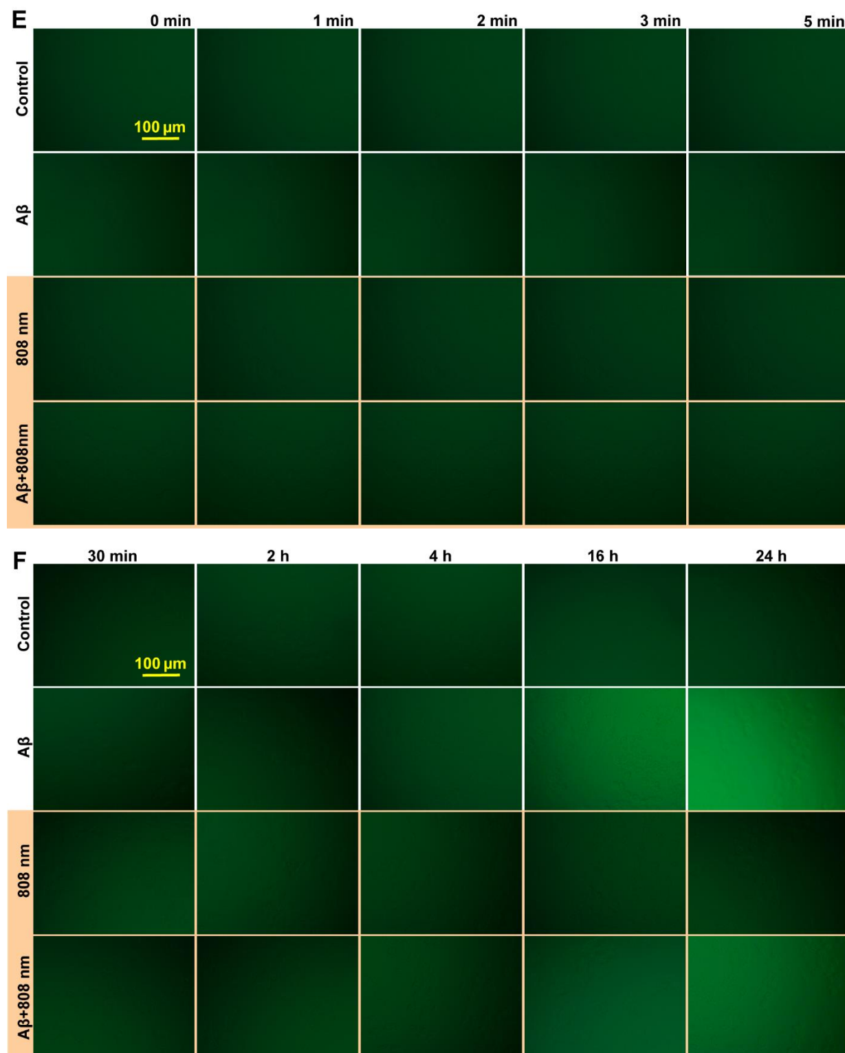
Fig. S6 NIR light effect on general ROS generation, mitochondrial ROS generation and ROS generation in the medium measured for Aβ-treated microglia. Epifluorescence microscopy images showing the effect of 808 nm light with 10 J/cm 2 , Aβ and both Aβ with light on microglia cells stained with (A), (B) CM-H2DCFDA for general ROS detection, (C), (D) MitoSOX™ for mitochondrial ROS detection, and (E), (F) ROS-Glo™ for ROS detection in the medium. Dynamic images showing the effect during (A), (C), (E) 5 min and (B), (D), (F) 24 h.
