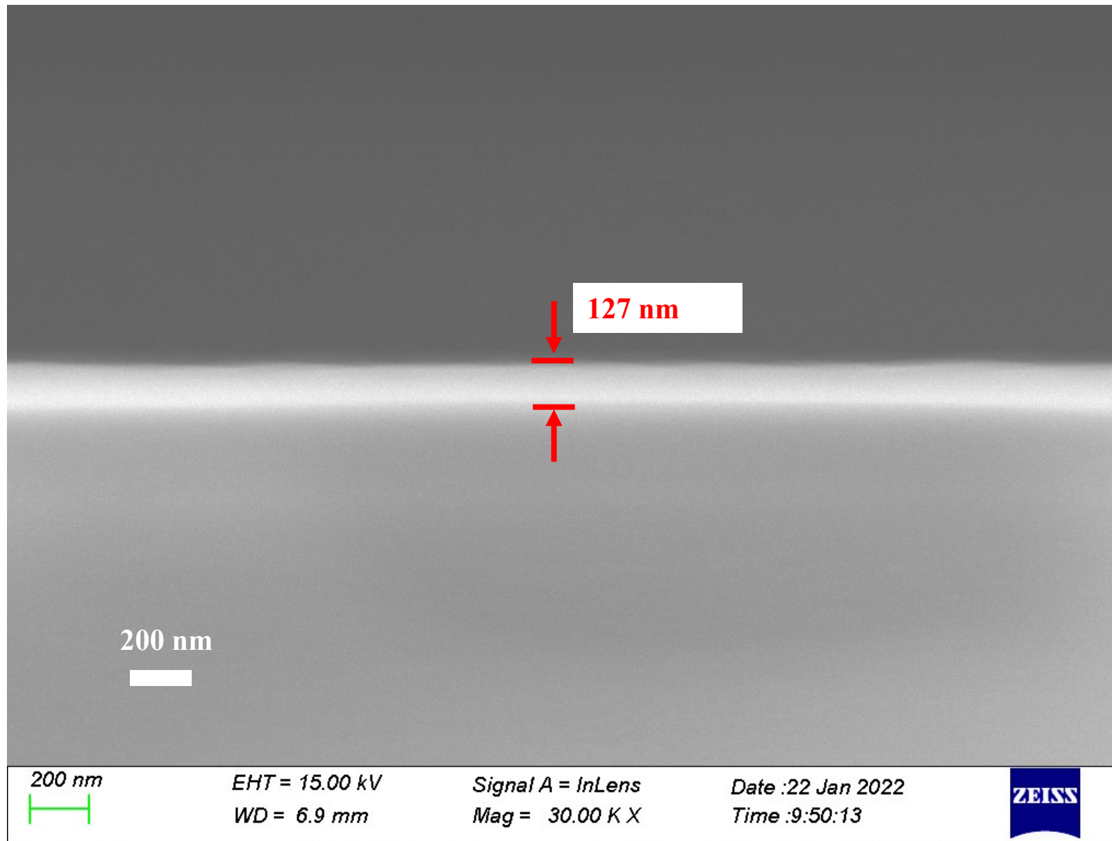
Fig.S-5: SEM cross sectional image of YIG film grown on (111) YAG, film growth time is 30 min
