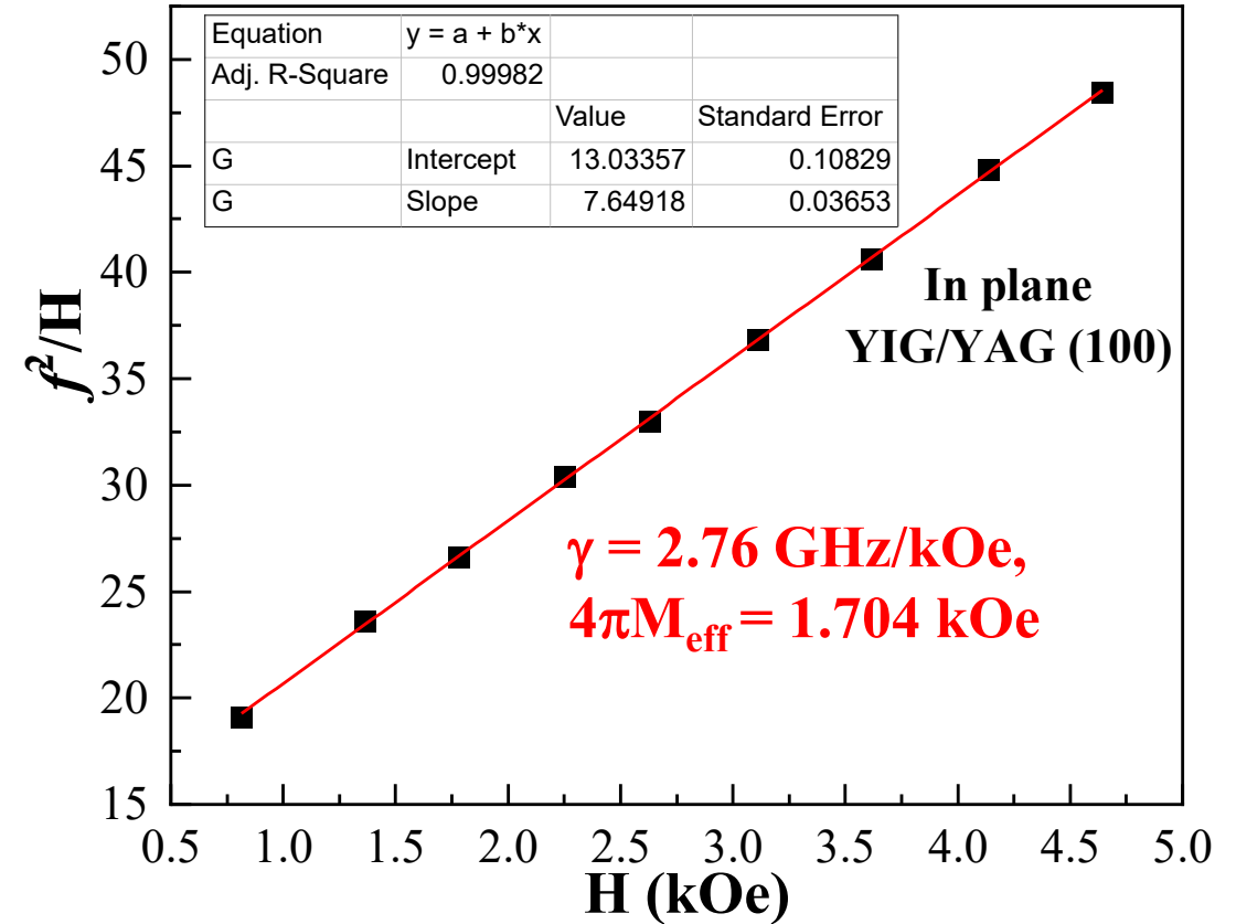
Fig. S-17. (Left) Profiles of amplitude scattering matrix S_{21} vs H showing FMR in 380 nm thick YIG/(100) YAG for in-plane H along [001] direction of YAG. (Right) Theoretical fit to data on resonance frequency and field for estimation of magnetic parameters for the film.
