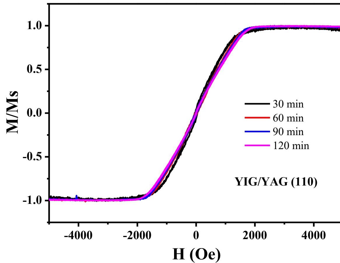
Figure S-13: Normalized magnetization vs H hysteresis loops for out-of-plane H as in Fig.S12 for YIG films on (110) YAG.
