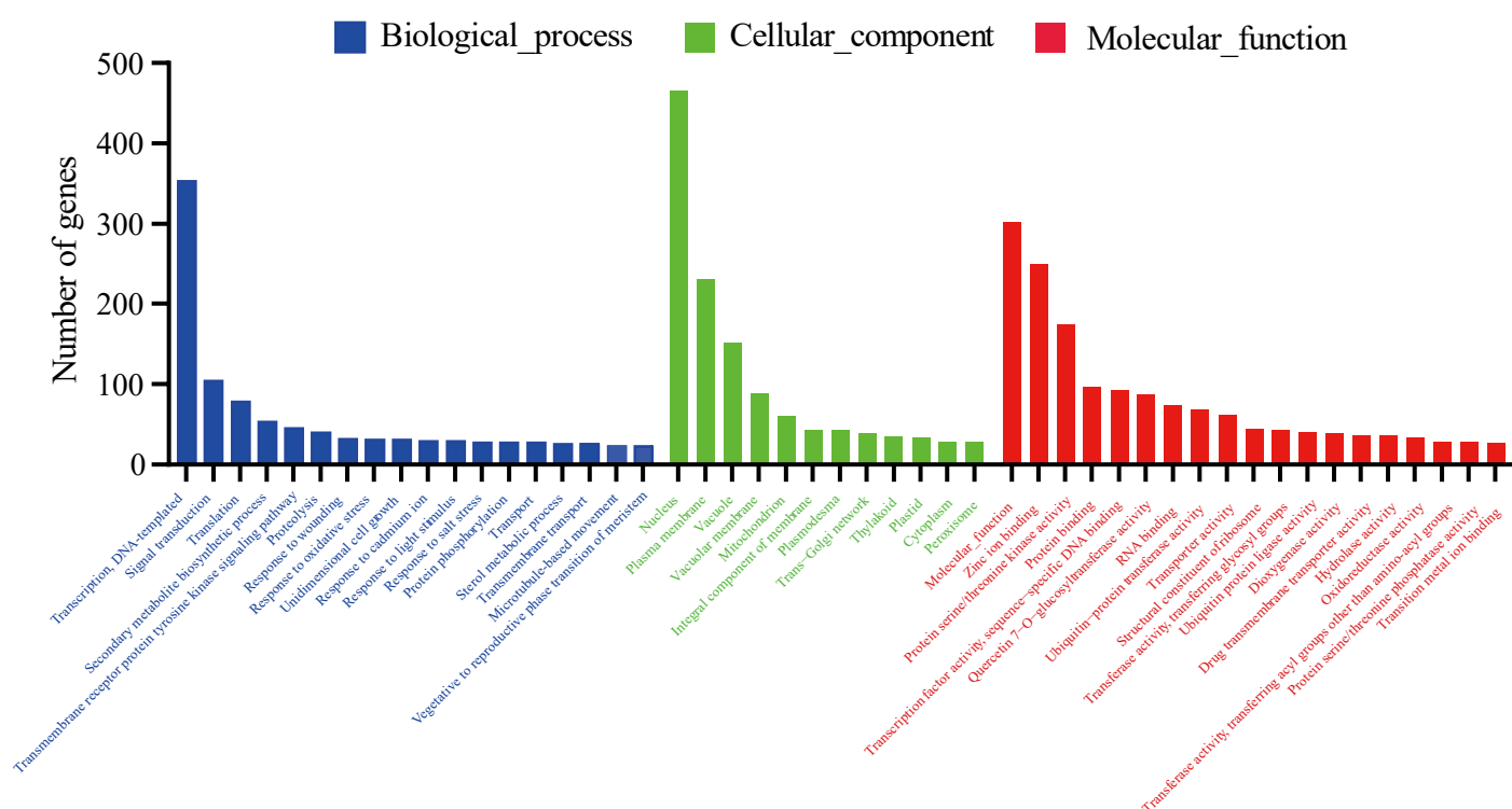
Fig. S2 | Histogram presentation of GO classification in different genes. Bas represent the numbers of unigenes matched of each GO term of three categaories. Biological process (blue), Cellular component (green). Molecular function (red).
