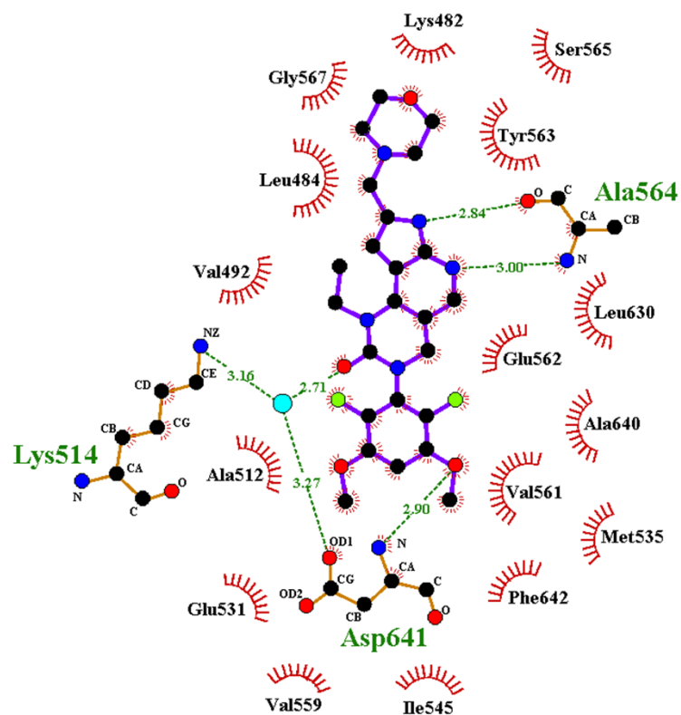
Figure S1. Ligand interaction diagram (LID) demonstrated the interaction of FGFR1/Pemigatinib. Hydrogen bonds (distance \leq 3.35 Å) are designated with a green dashed line, and van der Waals interactions (distance \leq 3.9 Å) are shown by a red half “sun” arrangement. The water is showed as blue sphere. Graphics were drawn by LigPlot+
