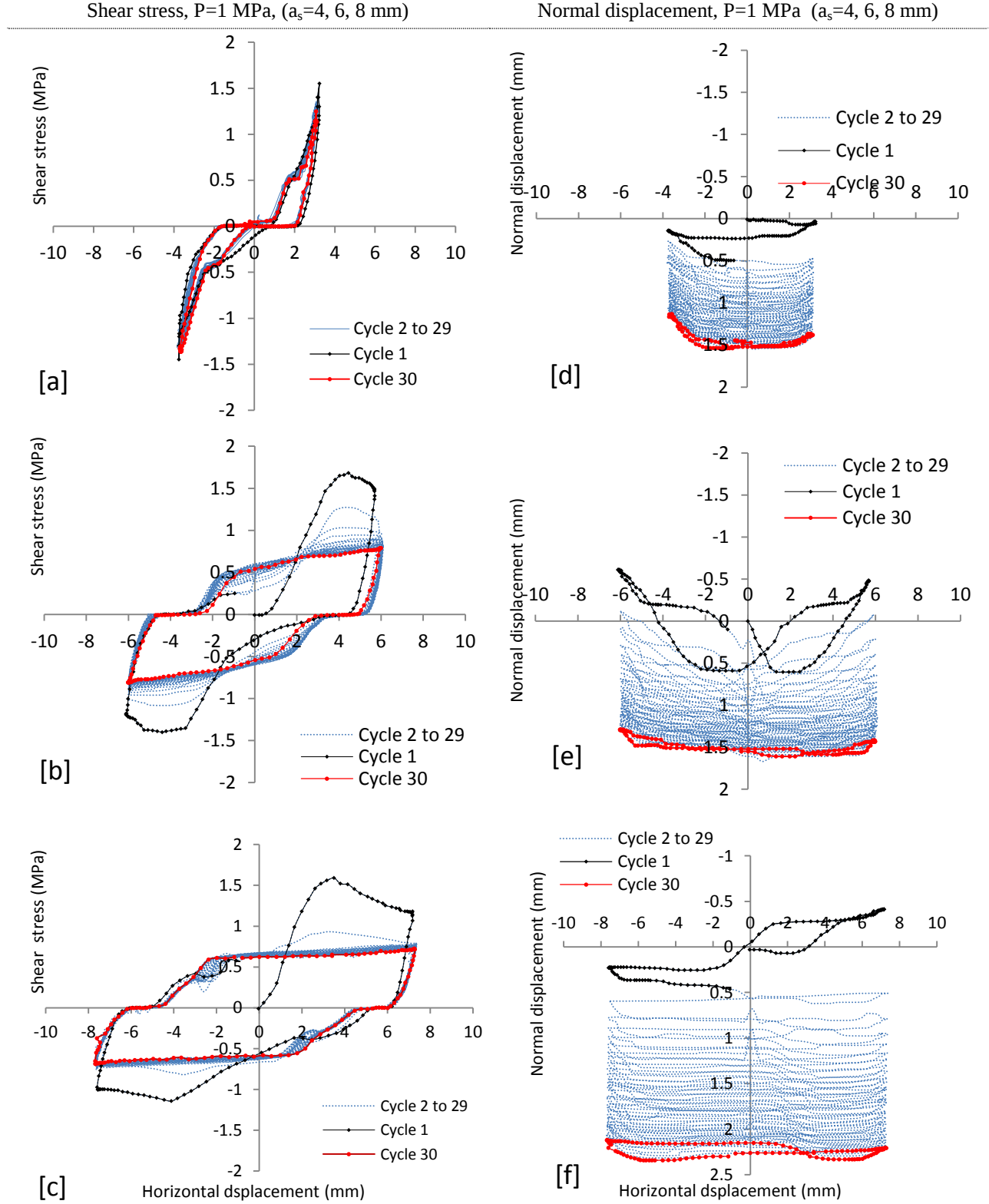
Fig. 15 Shear stress and normal displacement vs. horizontal displacement of 30°-30° joint for cyclic shear load with different amplitudes, a_s=4, 6 and 8 mm respectively ( P=1 MPa)
