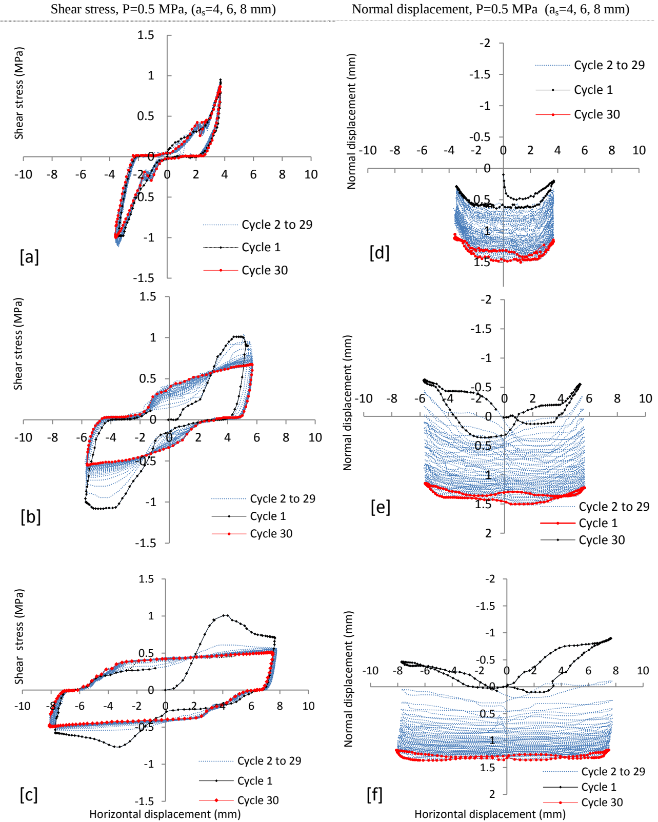
Fig. 14 Shear stress and normal displacement vs. horizontal displacement of 30°-30° joint for cyclic shear
