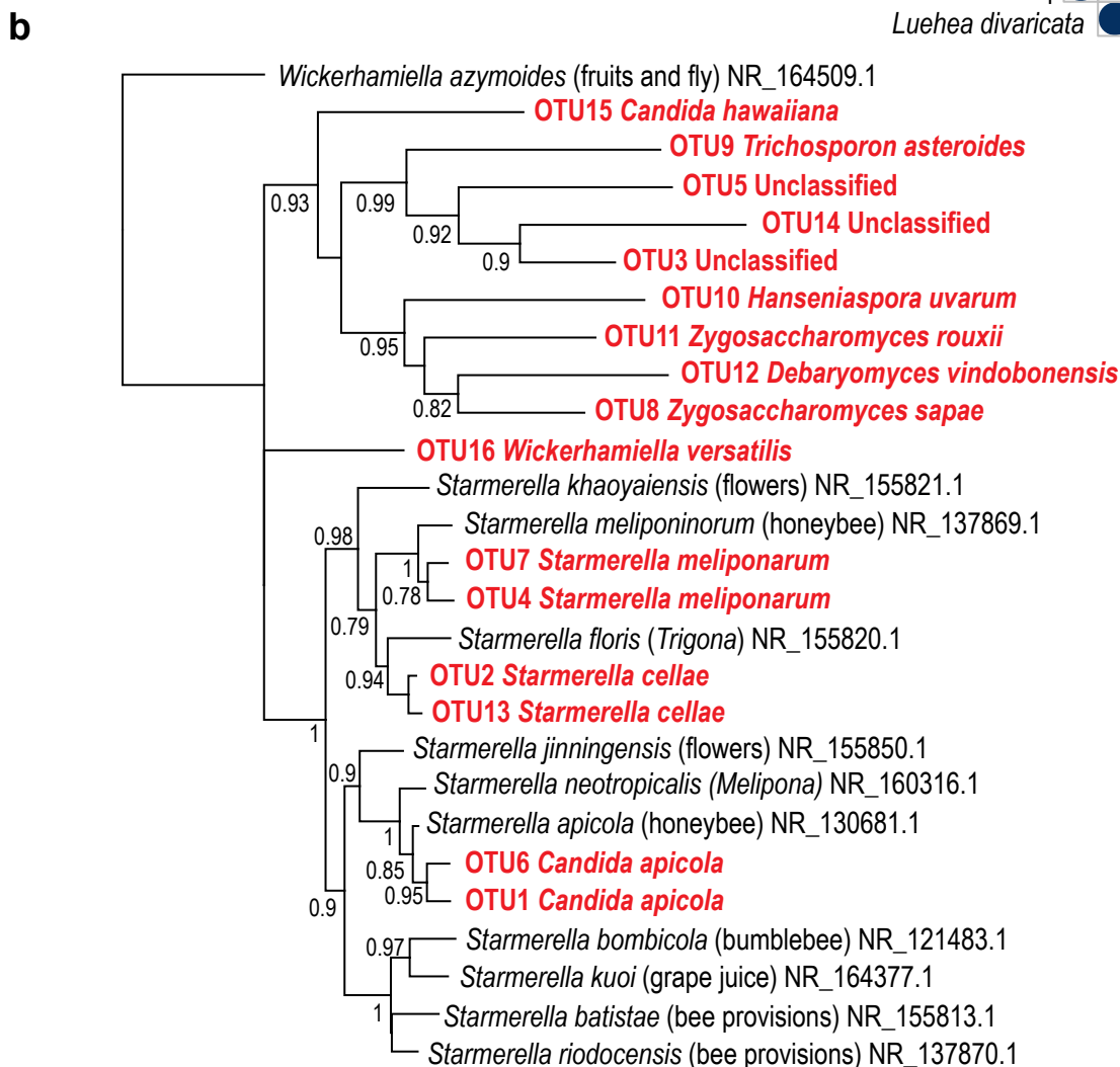
Supplementary Fig. 5 - Pairwise correlation analyses between the fungal and pollen taxa identified in our study (a), and phylogenetic analyses of the representative fungal OTUs, using the same ITS2 sequences from Cerqueira et al. (2021) as references.
