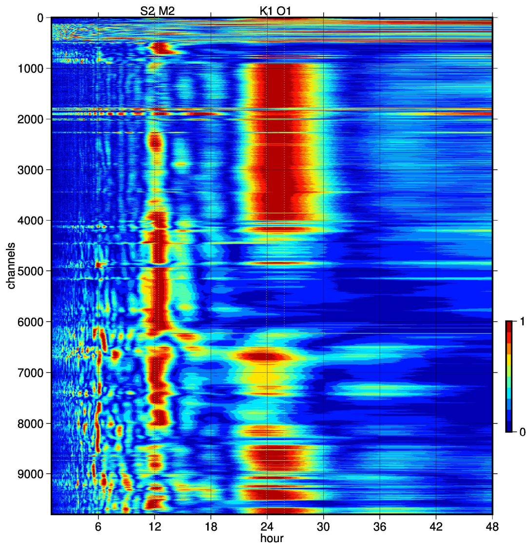
Figure S3. Strain rate periodogram for each channels. Normalized for each channels. S2, M2, K1, and O1 show the period of four large tide constituents.
