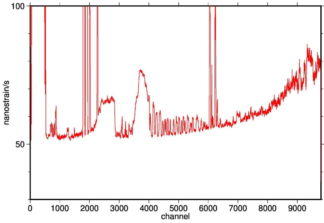
Figure S1. Standard deviation of observation at each channel. Median values of standard deviation of strain rate, measured for each five minute at each channels.
