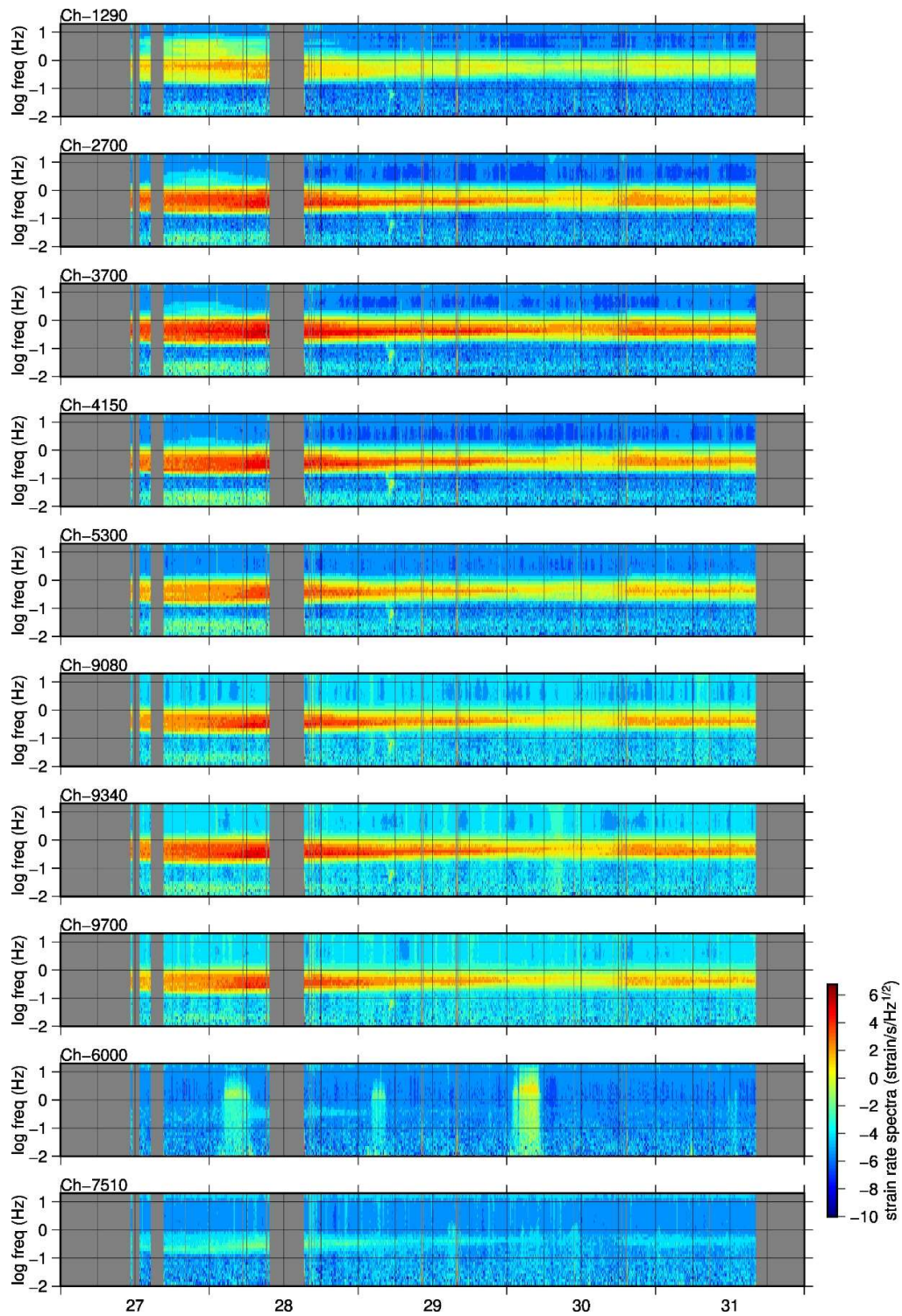
Figure S2. Spectrogram at 10 selected channels. This shows periodogram of strain rate calculated for every five minutes.
