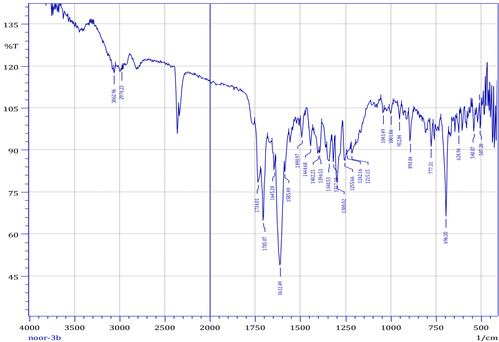
FTIR spectrum of compound ( 3b )
