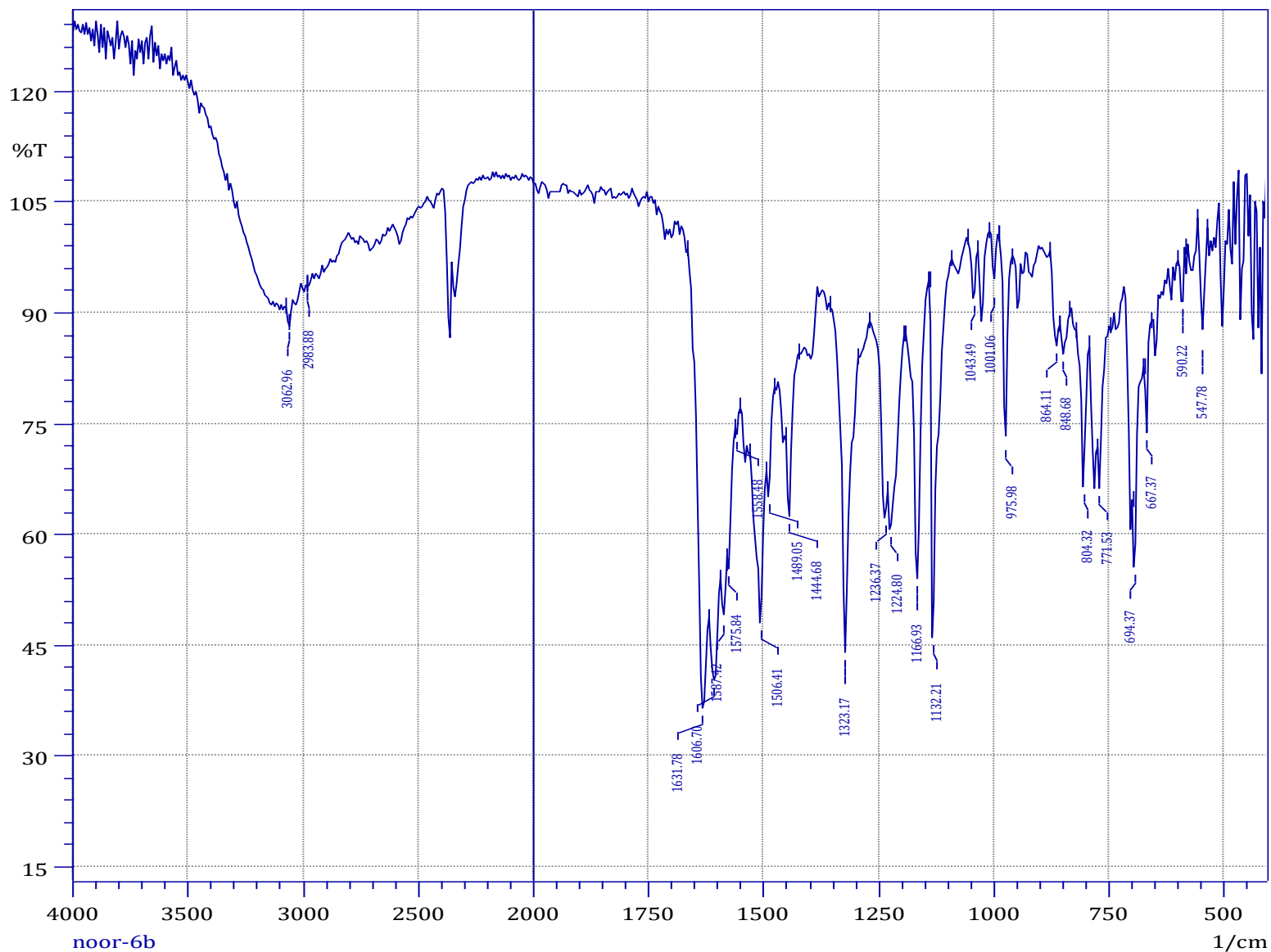
FTIR spectrum of compound ( 6b )
