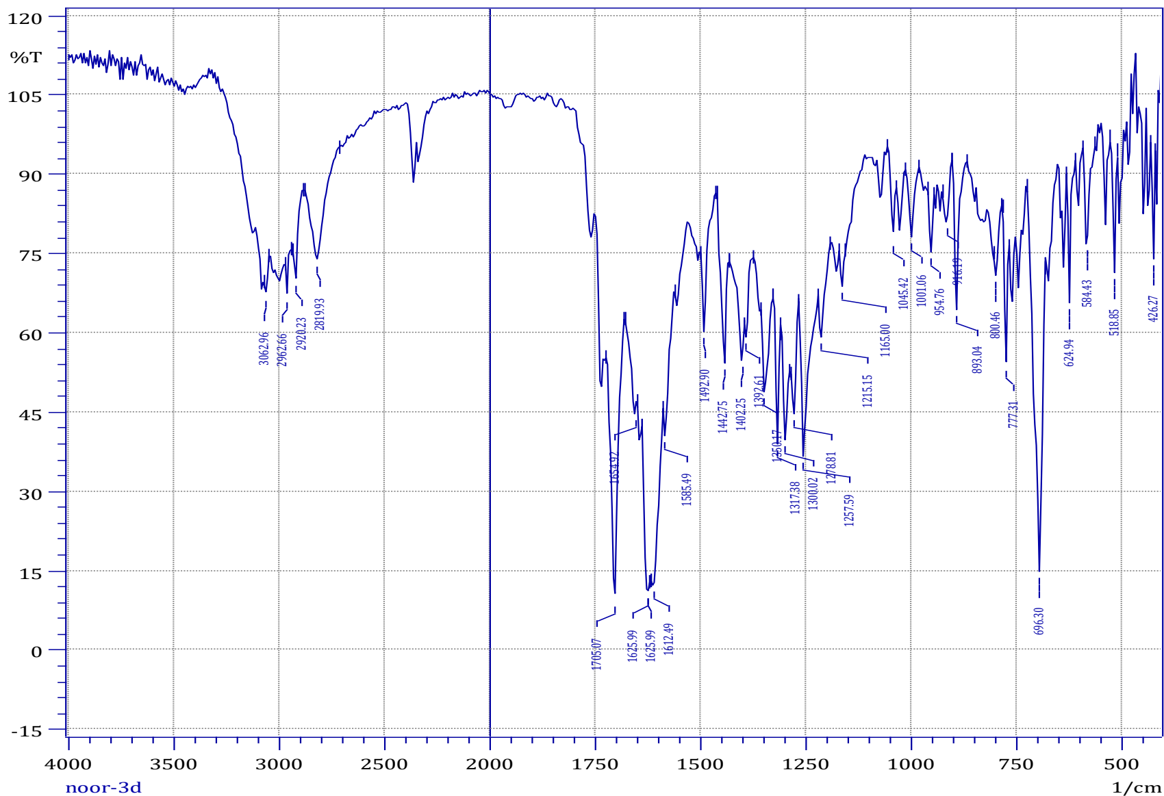
FTIR spectrum of compound (3d)
