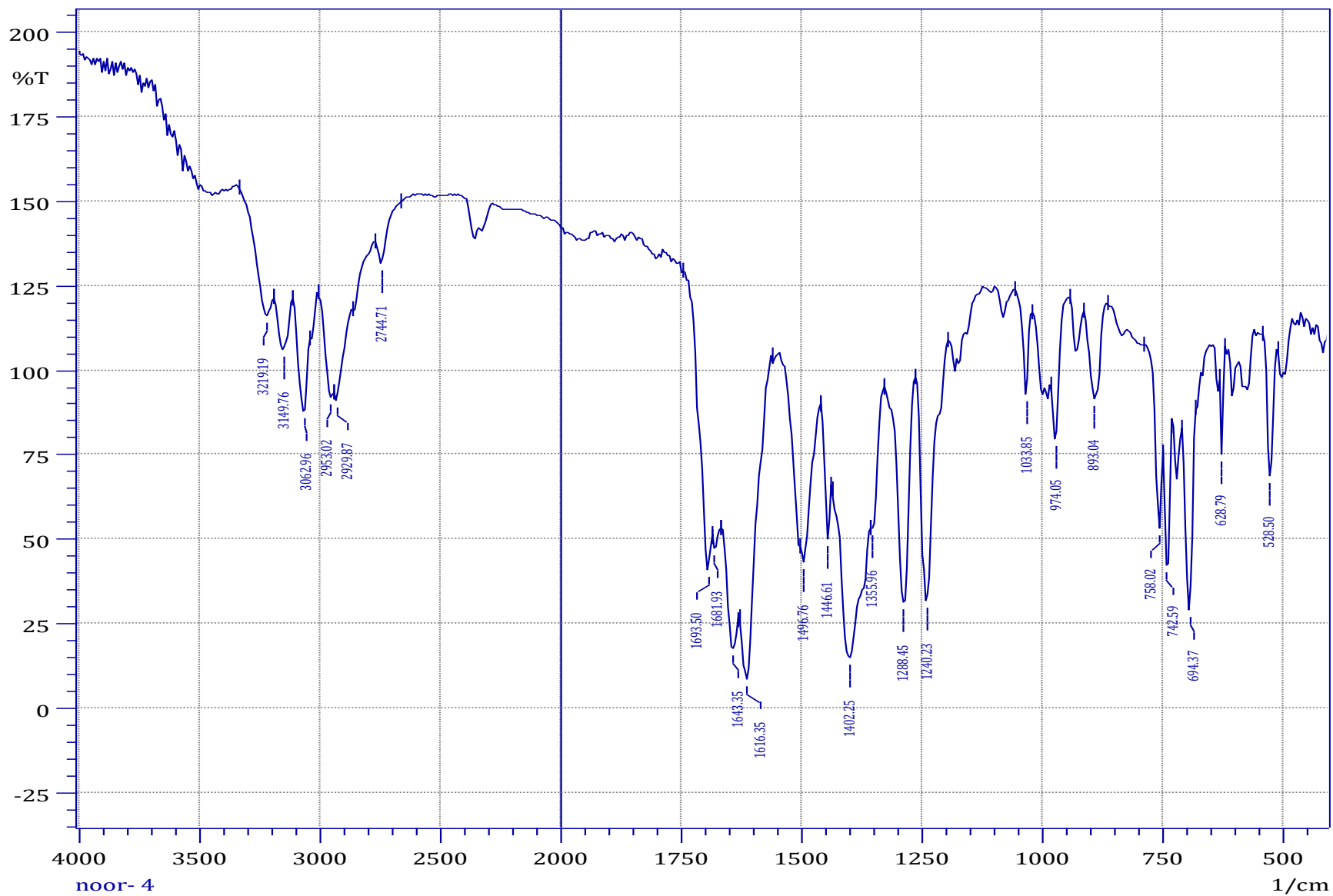
FTIR spectrum of compound ( 4 )
