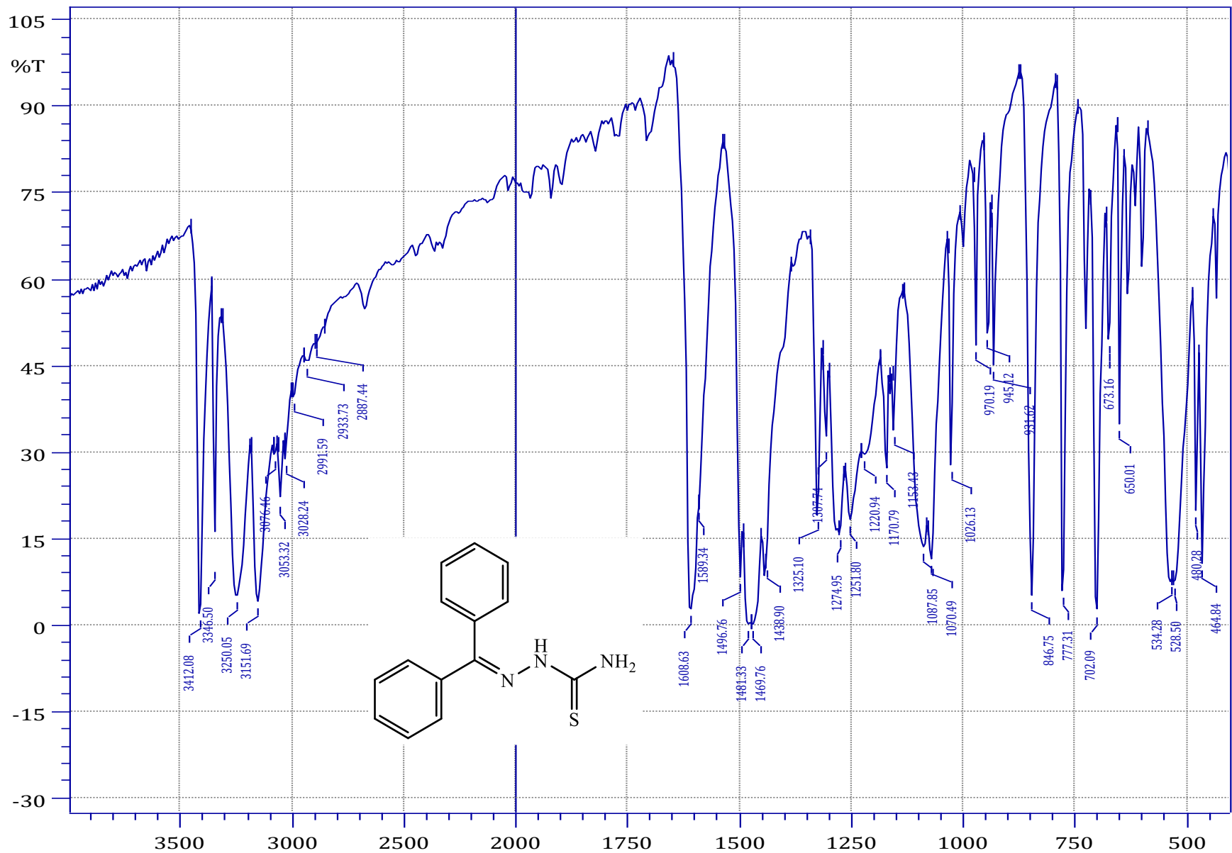
FTIR spectrum of compound ( 1 )
