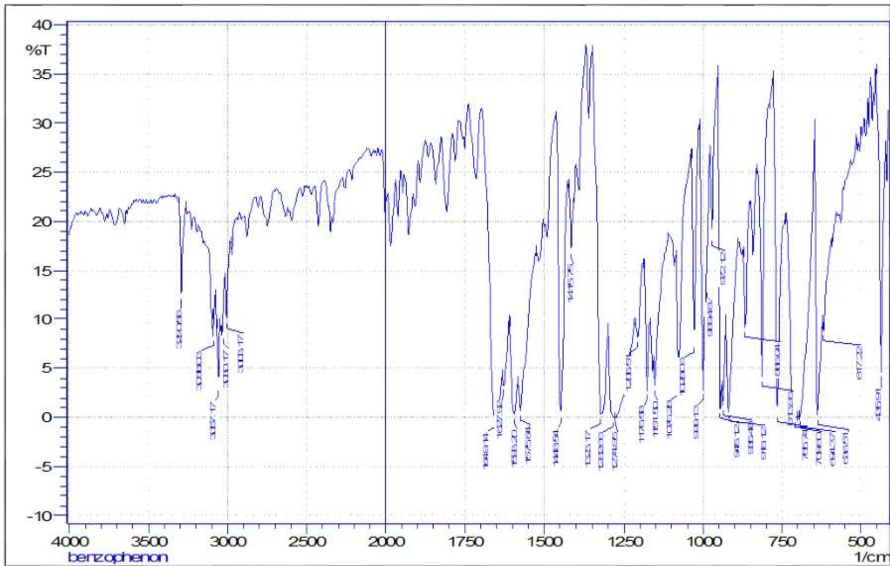
FTIR spectrum of benzophenone
