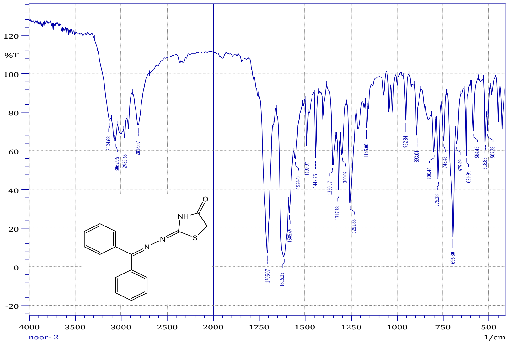
FTIR spectrum of compound ( 2 )
