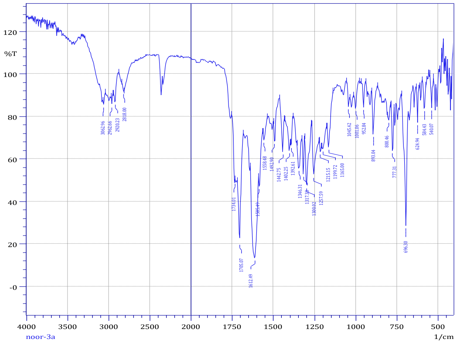
FTIR spectrum of compound ( 3a )
