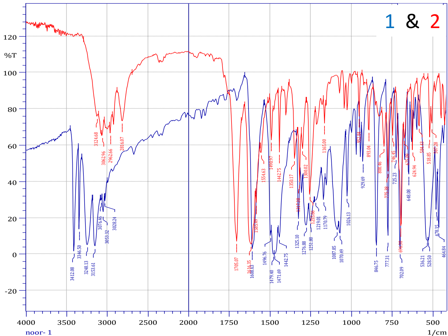
FTIR spectrum of compound ( 1 and 2 )
