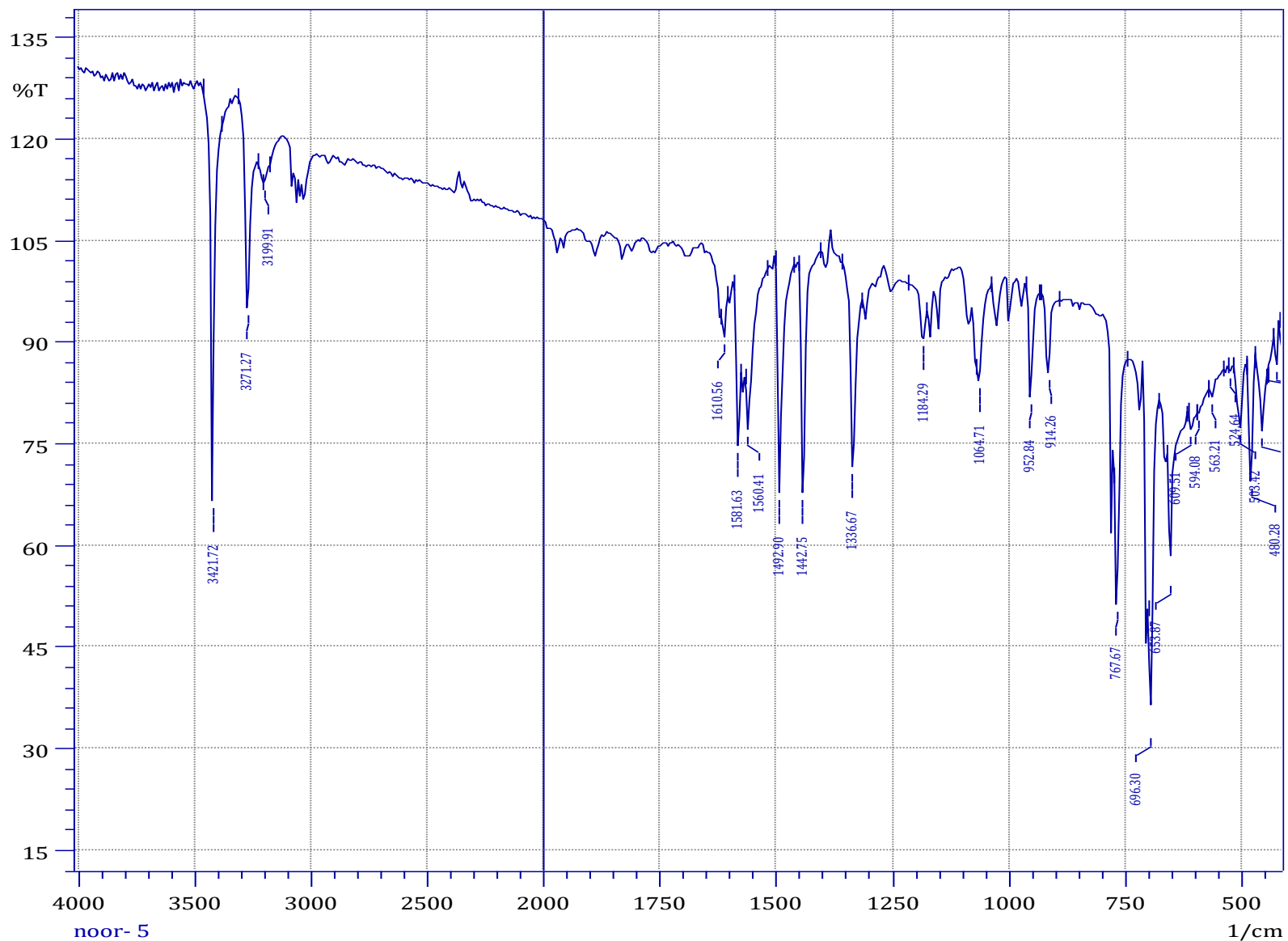
FTIR spectrum of compound ( 5 )
