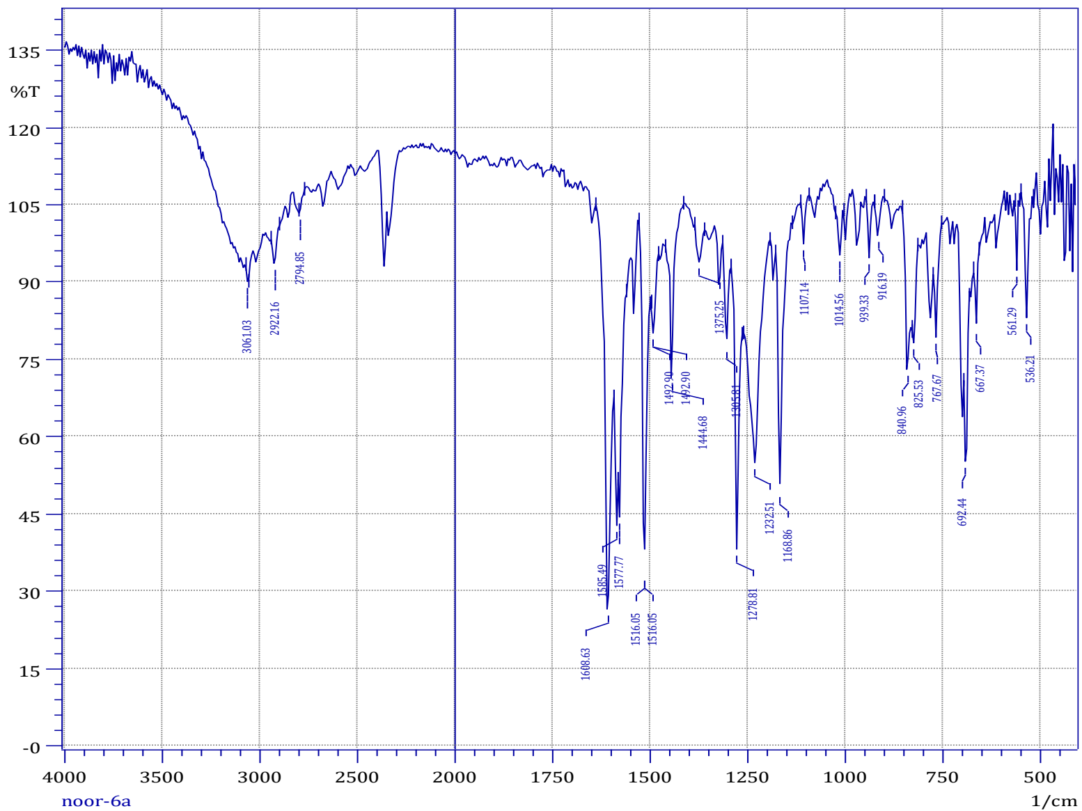
FTIR spectrum of compound ( 6a )
