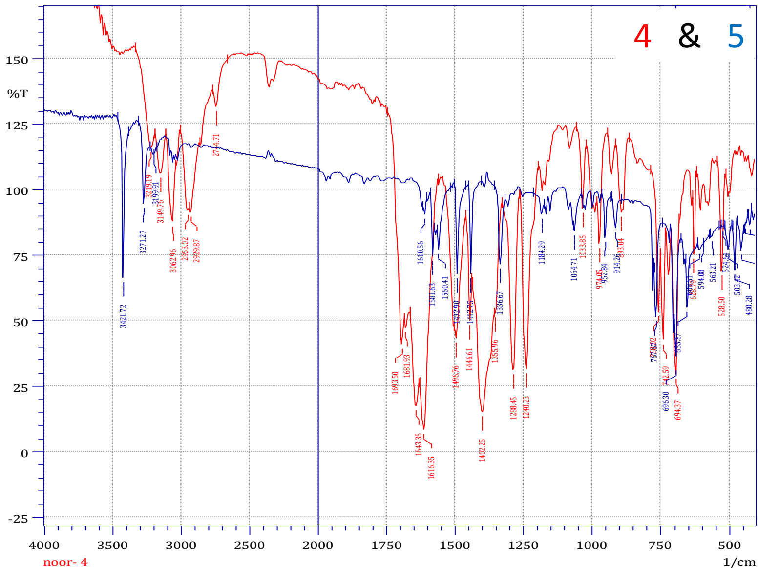
FTIR spectra of compound (4,5)
