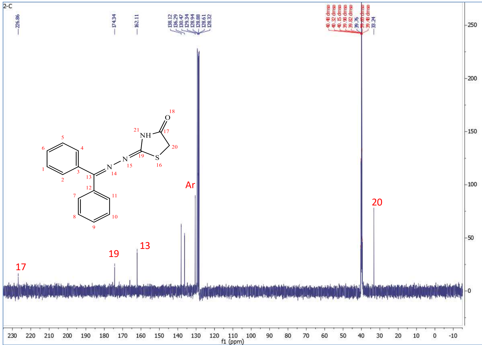
^{13}\text{C} NMR spectrum of compound 2
