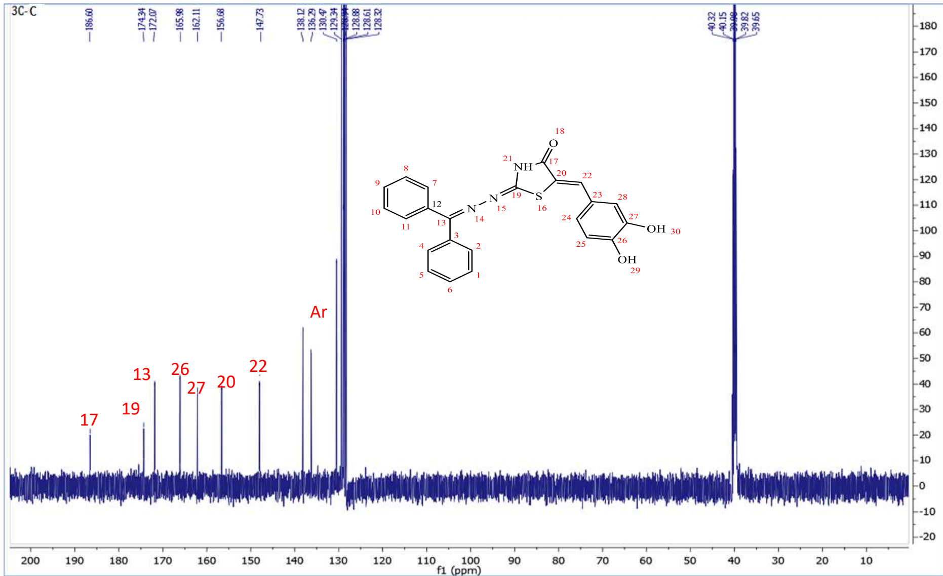
^{13}\text{C} NMR spectrum of compound 3c
