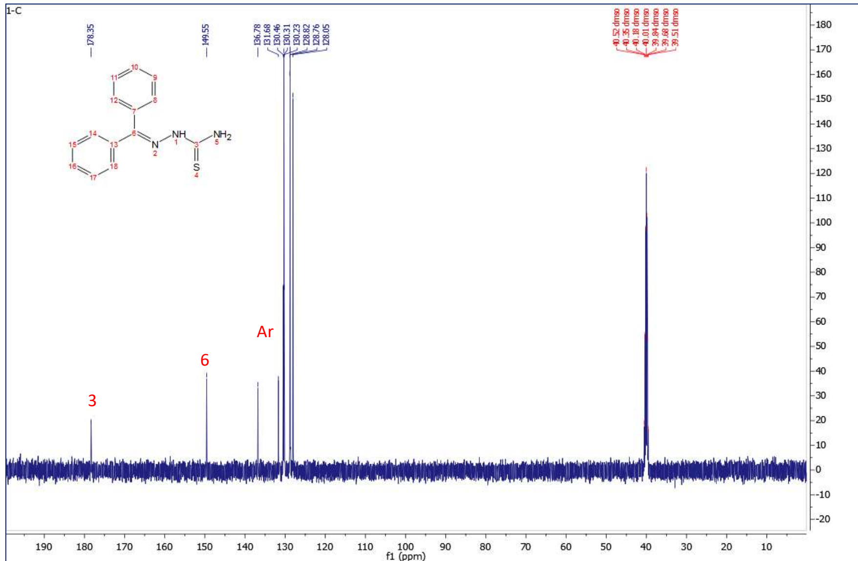
13 CNMR spectrum of compound 1
