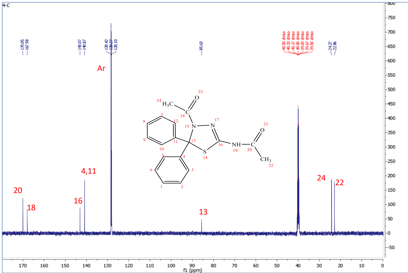
^{13}\text{C} NMR spectrum of compound 4
