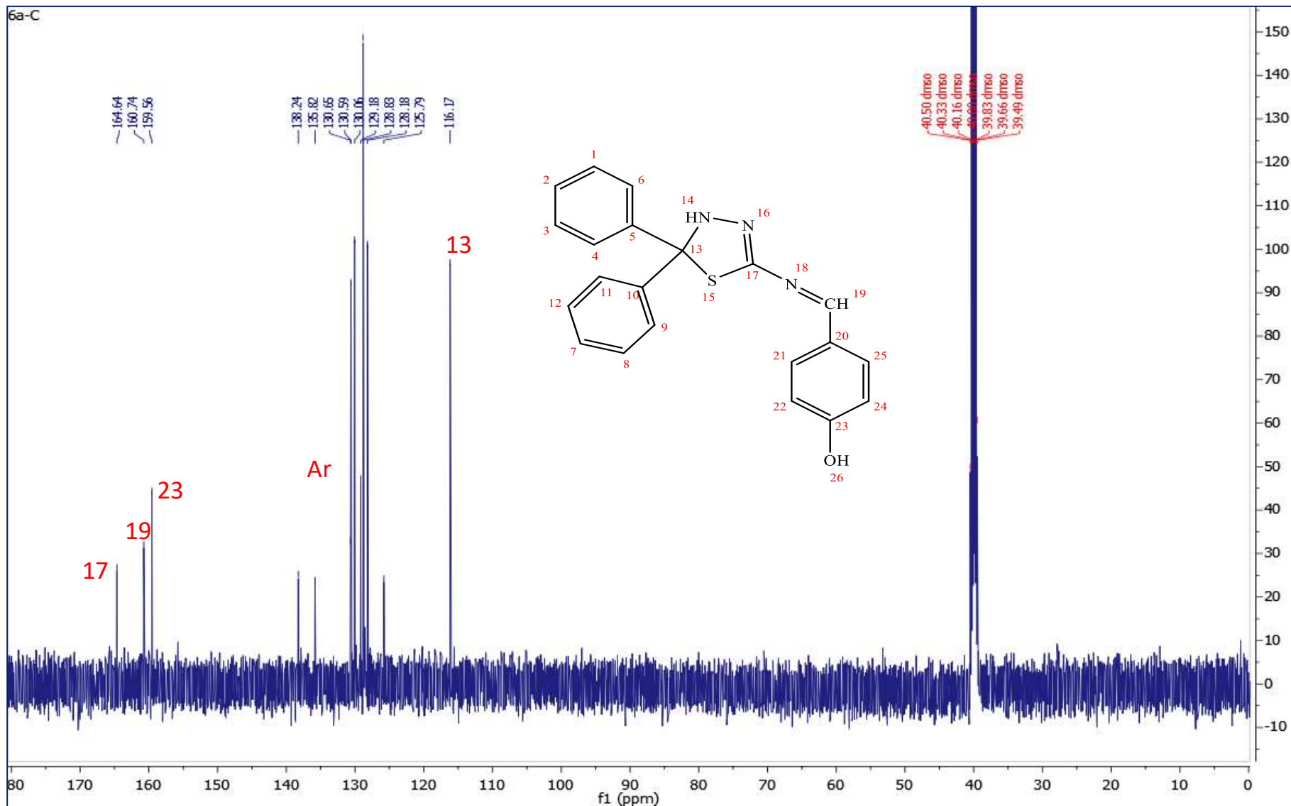
13 CNMR spectrum of compound 6a
