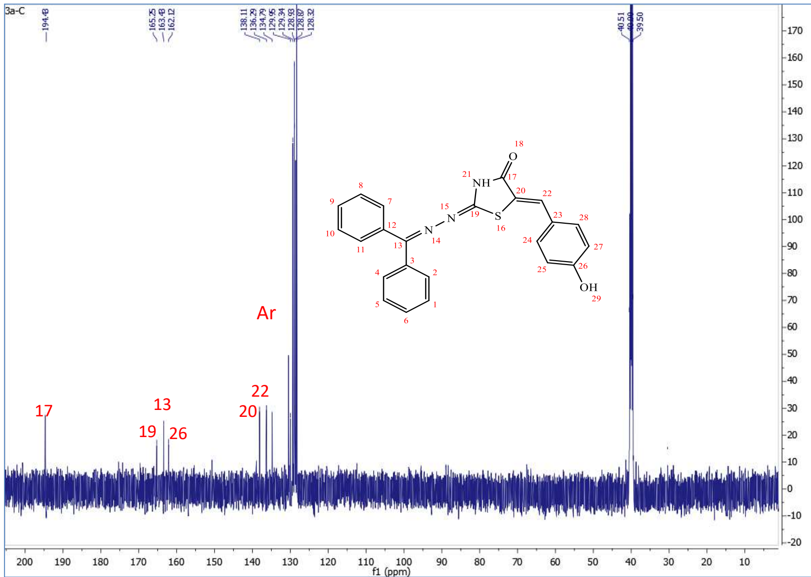
13 CNMR spectrum of compound 3a
