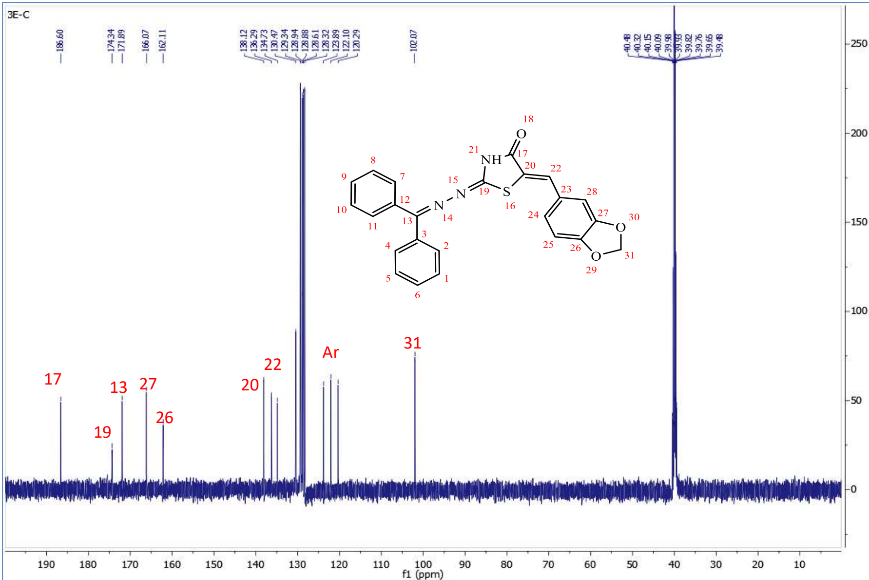
13 CNMR spectrum of compound 3d
