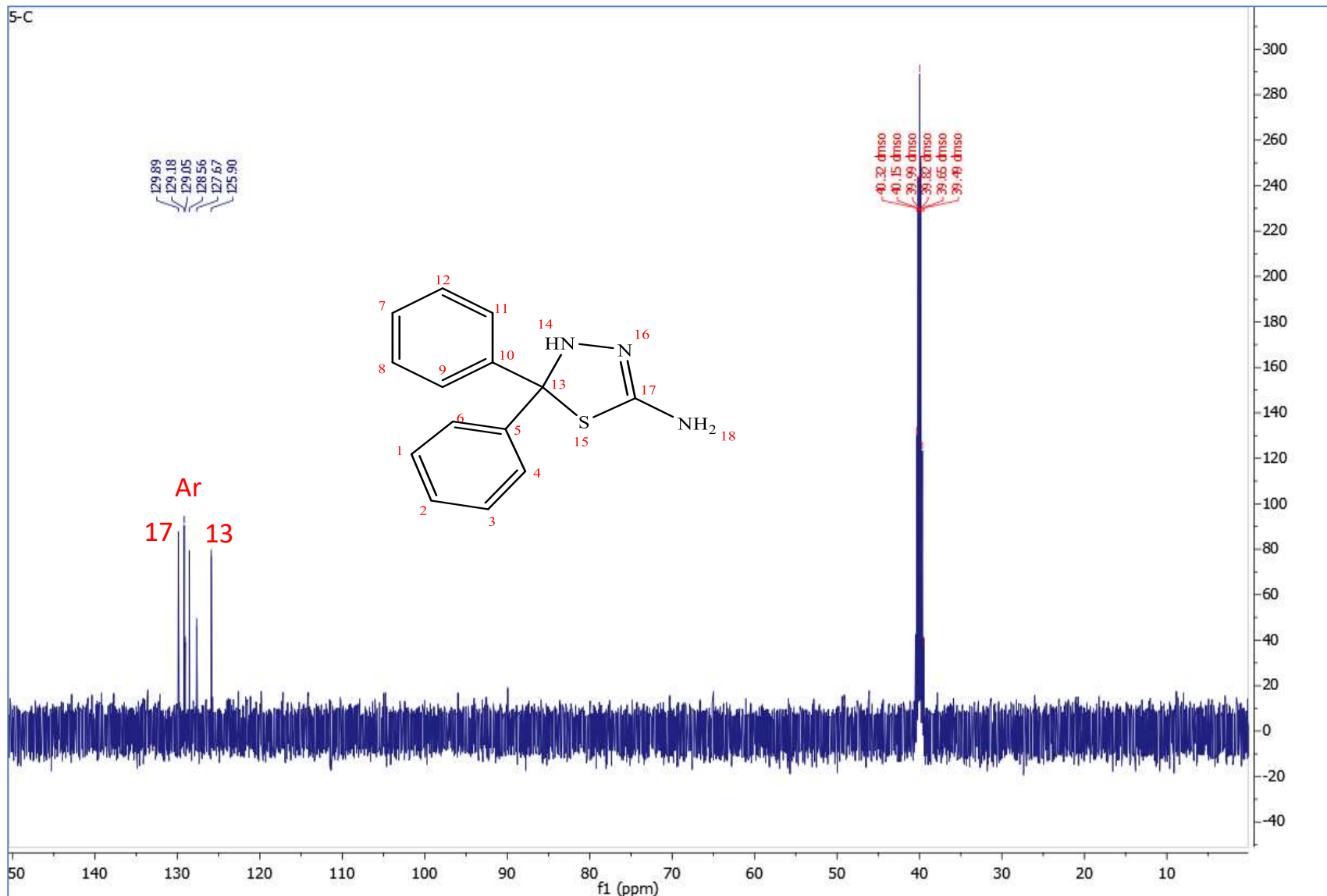
^{13}\text{C} NMR spectrum of compound 5
