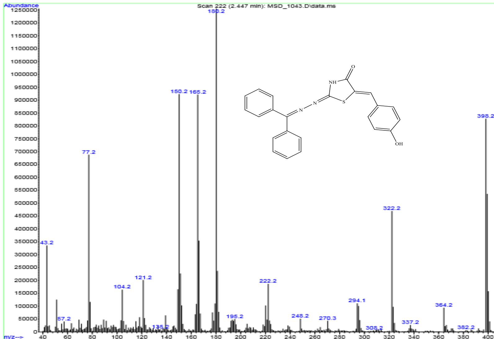
Mass spectrum of compound 3a
