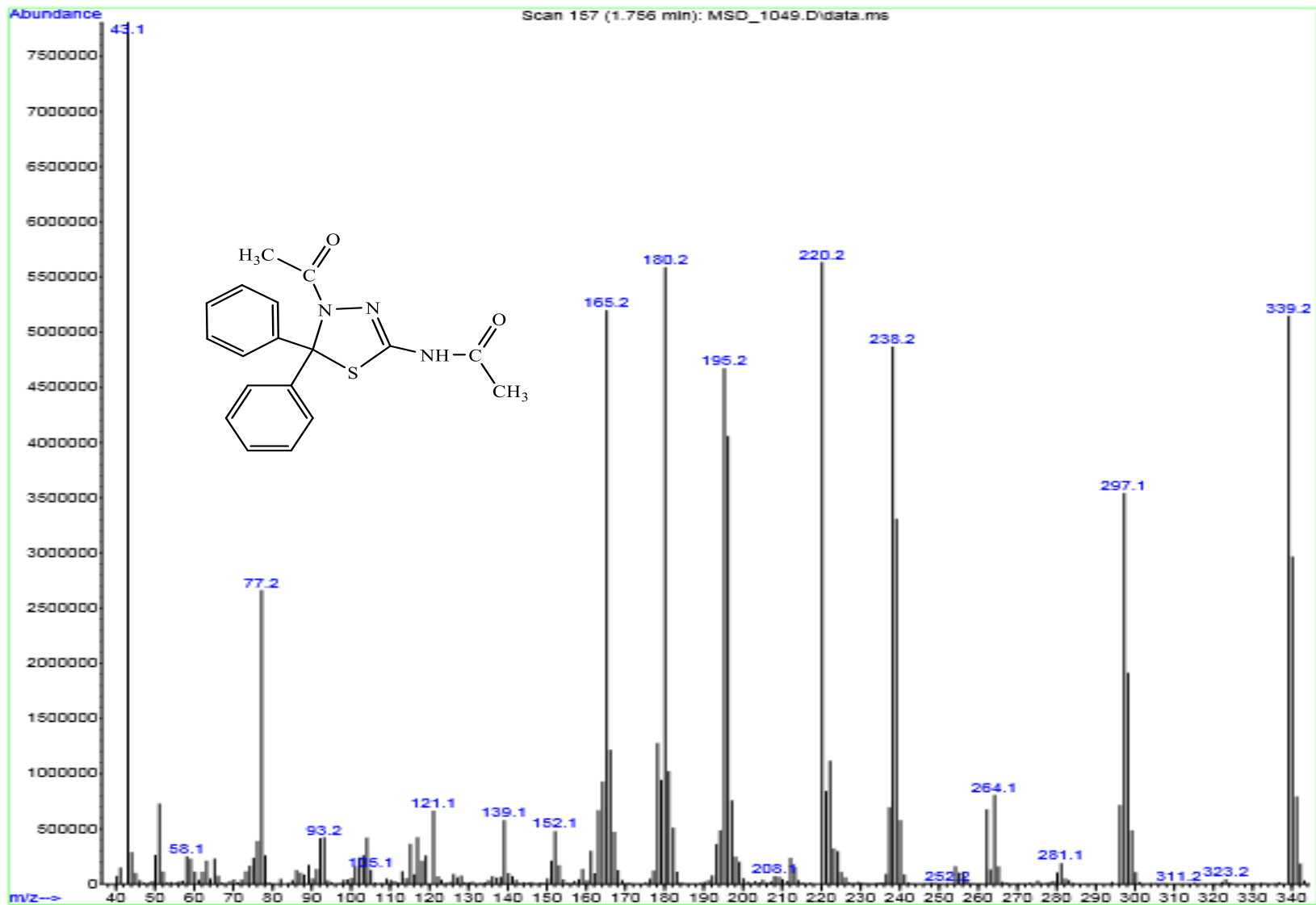
Mass spectrum of compound 4
