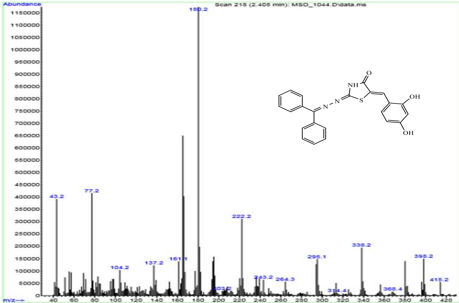
Mass spectrum of compound 3b
