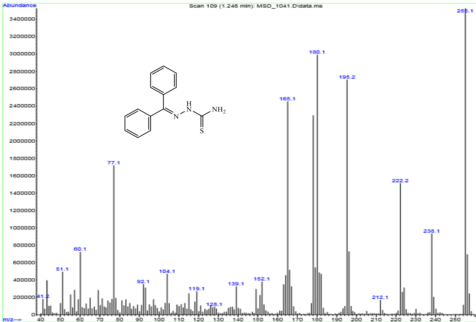
Mass spectrum of compound 1
