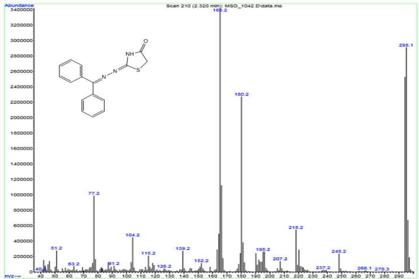
Mass spectrum of compound 2
