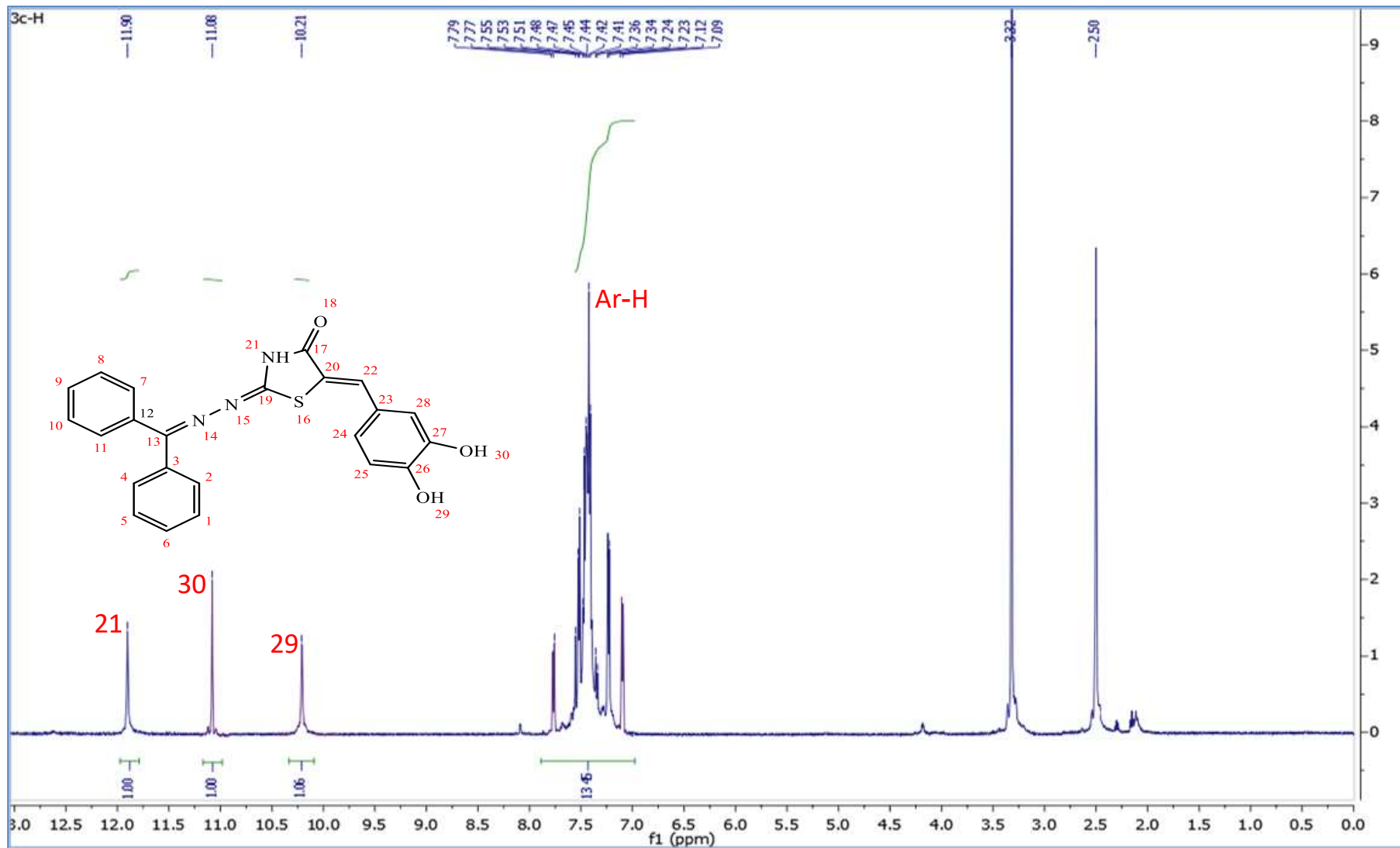
1H NMR spectrum of compound 3c
