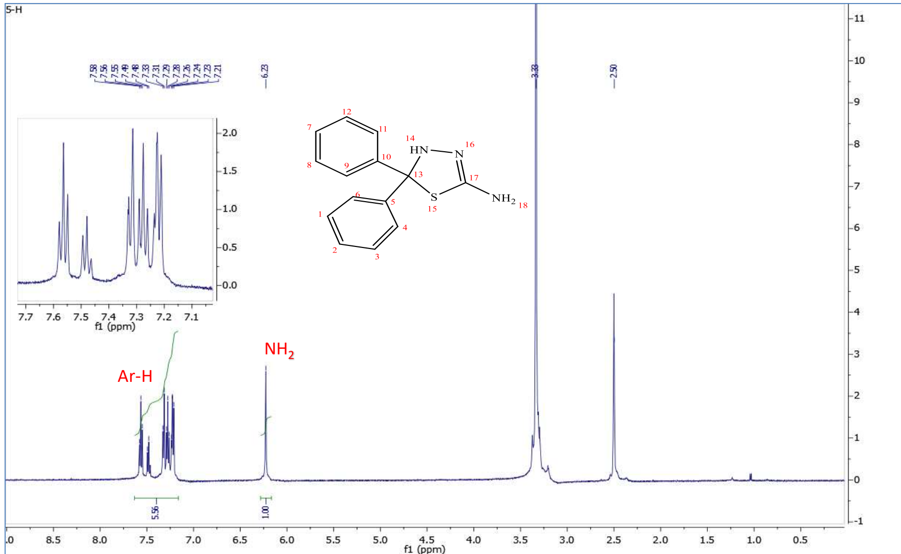
1H NMR spectrum of compound 5
