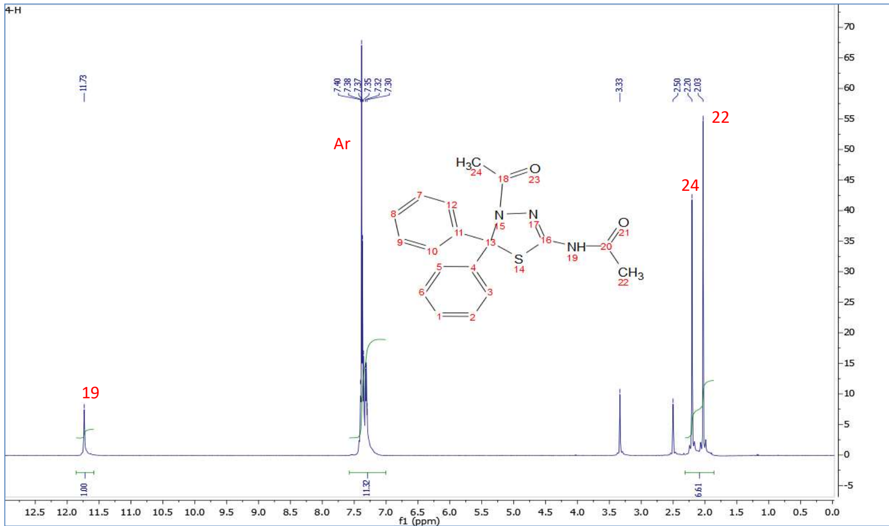
1H NMR spectrum of compound 4
