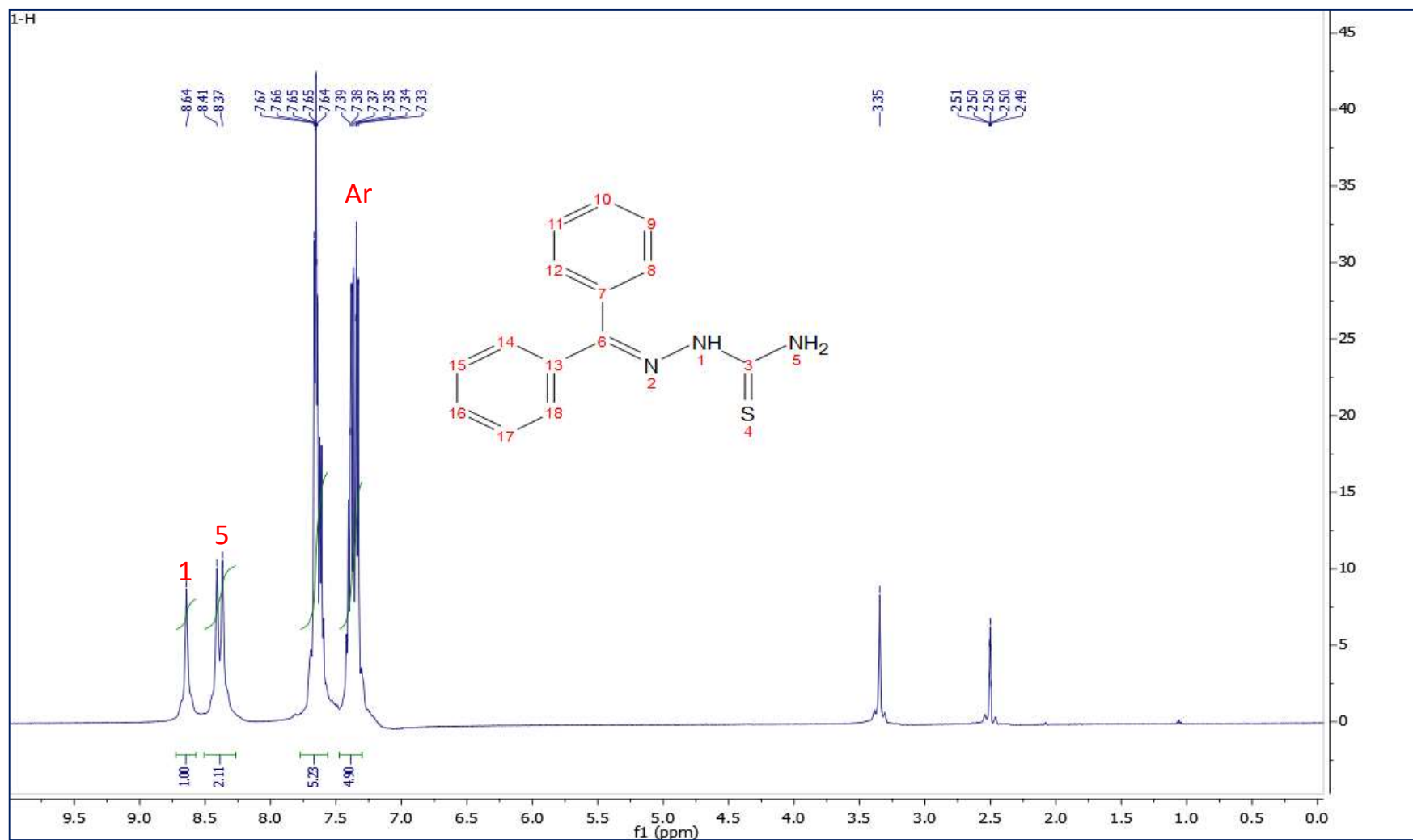
1H NMR spectrum of compound 1
