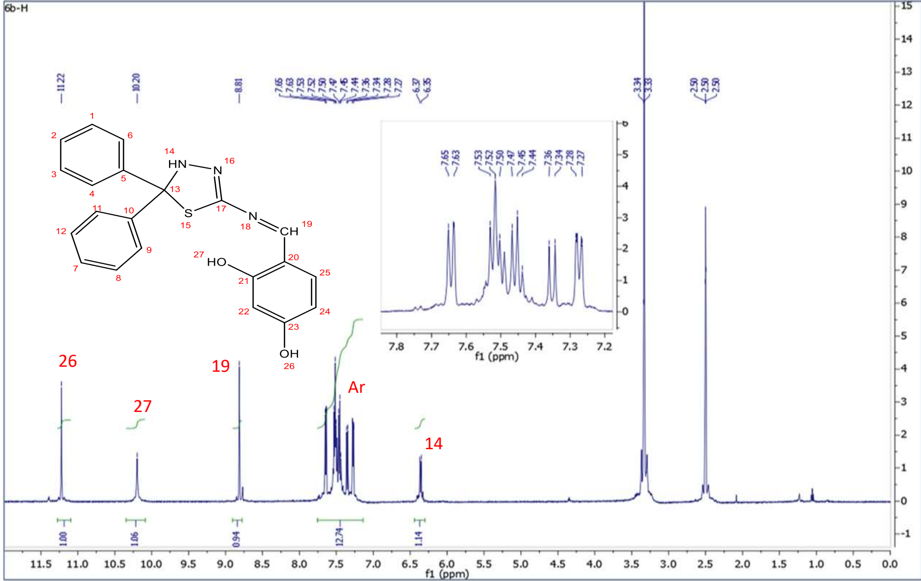
1 H NMR spectrum of compound 6b
