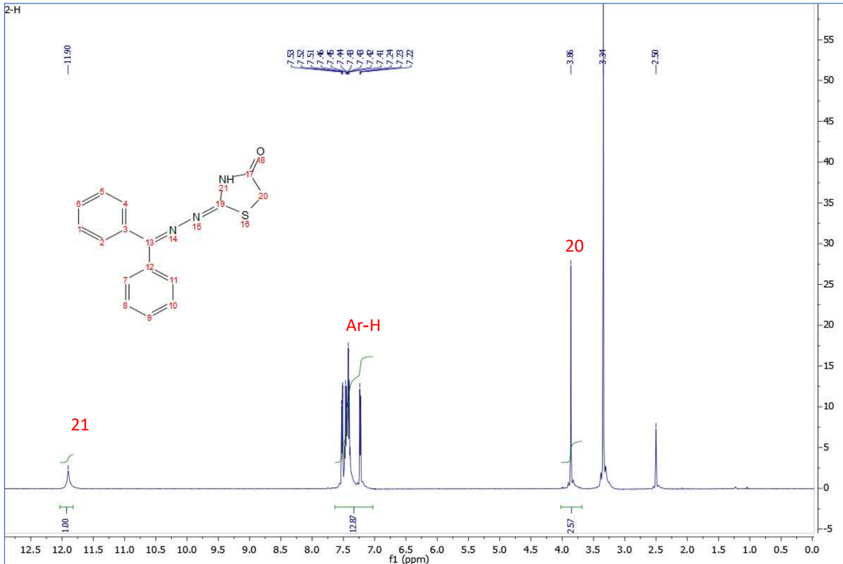
1HNMR spectrum of compound 2
