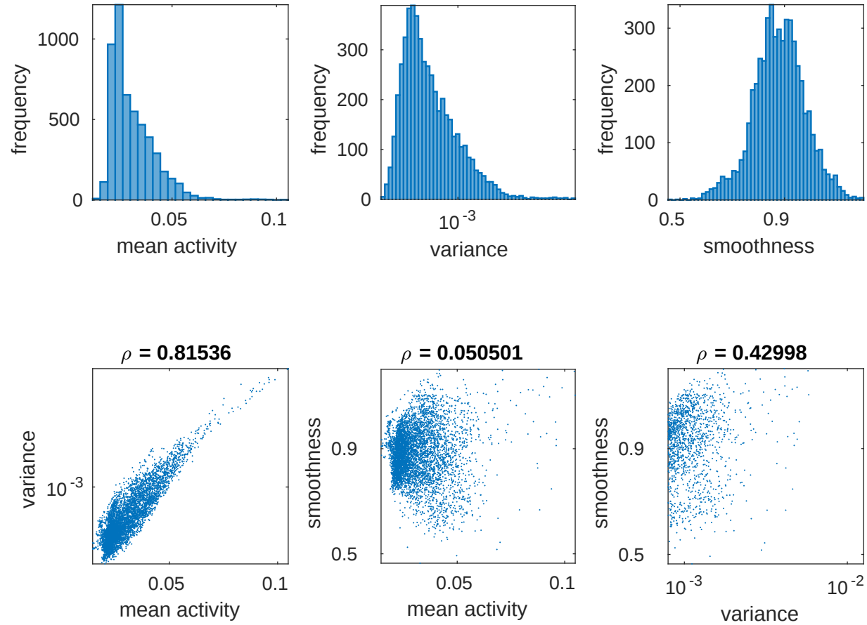
Extended Data Figure 4: Histograms and scatter plots of mean, variance, and time-resolved smoothness for a single representative recording. Note that variance and smoothness are log-transformed. \rho denotes the Spearman correlation coefficient.
