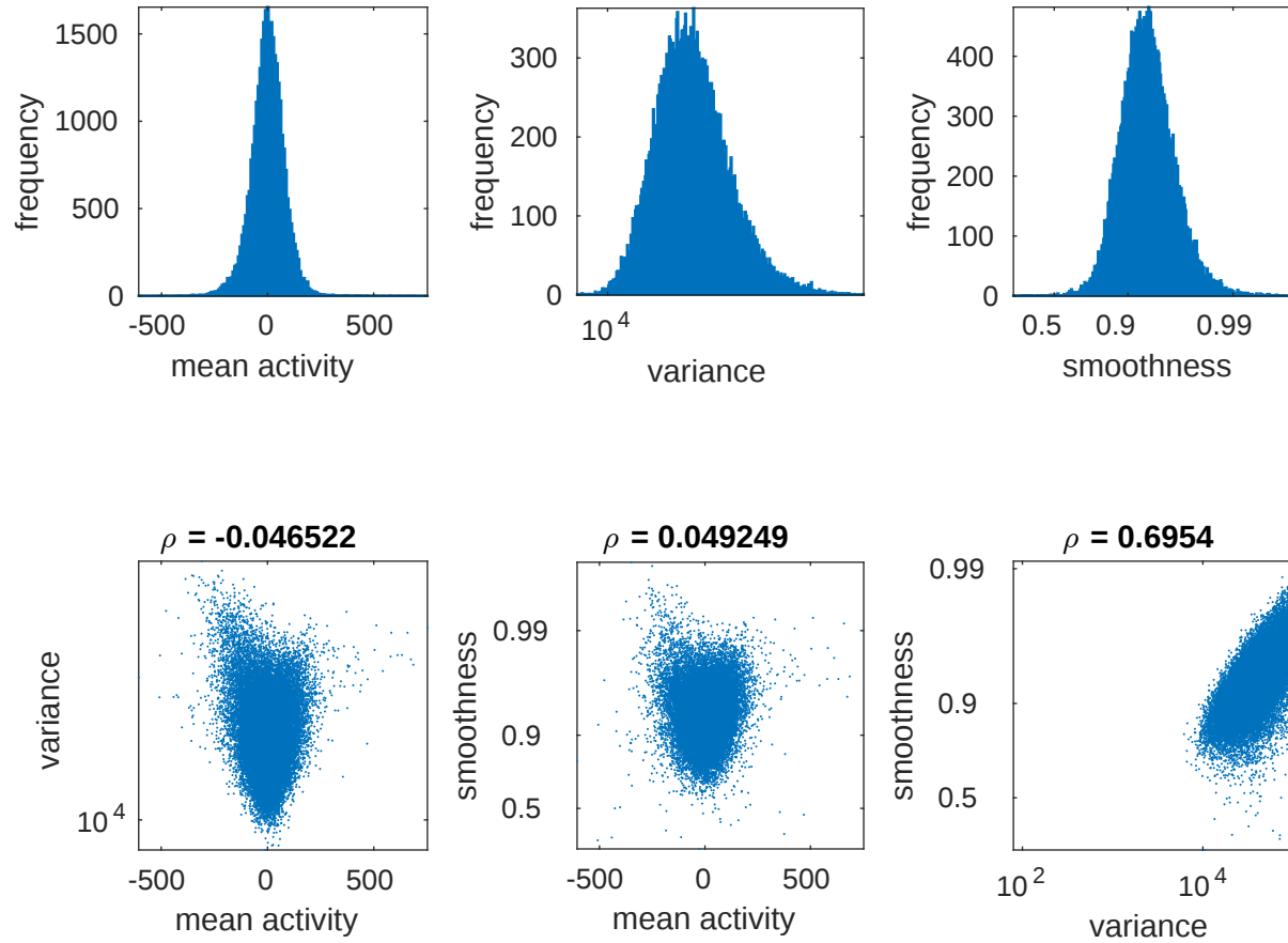
Extended Data Figure 3: Histograms and scatter plots of mean, variance, and time-resolved smoothness for a single representative recording. Note that variance and smoothness are log-transformed. \rho denotes the Spearman correlation coefficient.
