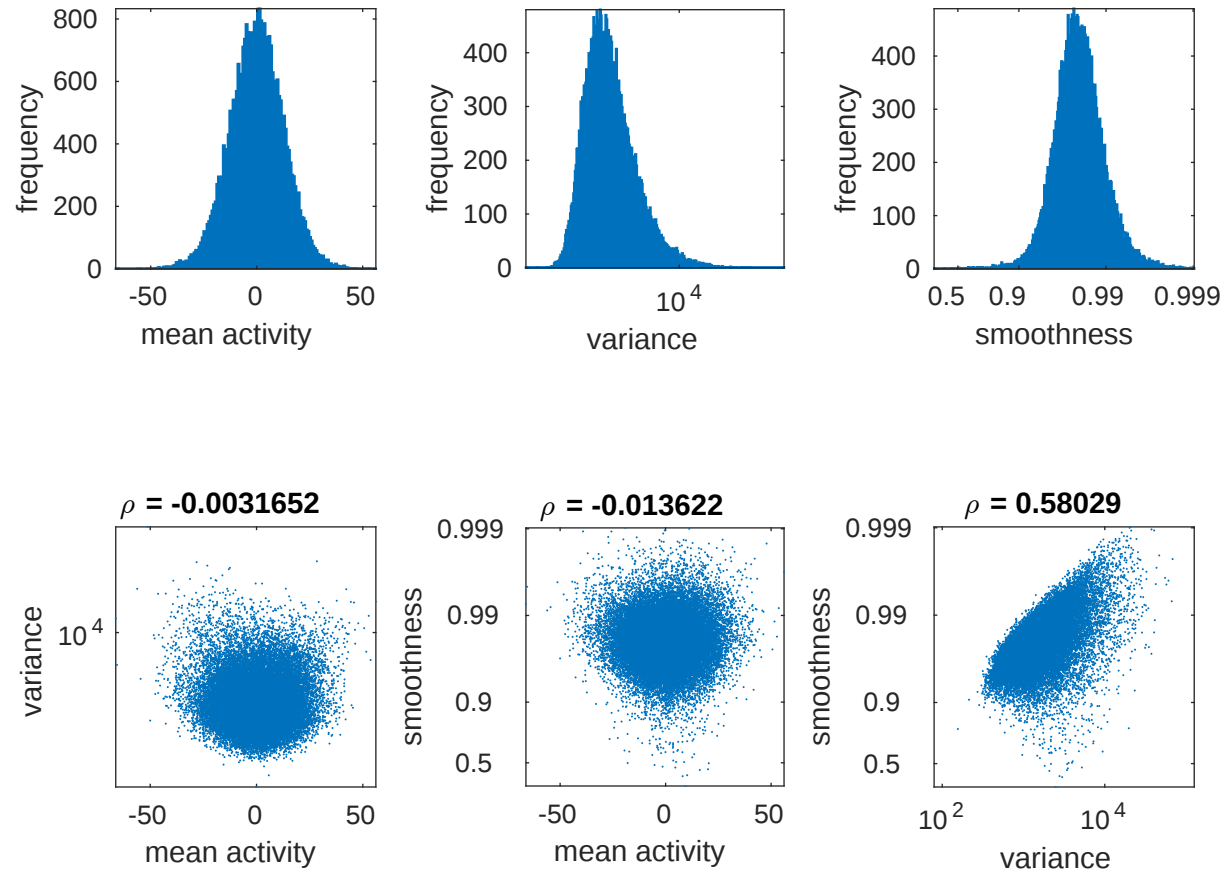
Extended Data Figure 1: Histograms and scatter plots of mean, variance, and time-resolved smoothness for a single representative recording. Note that variance and smoothness are log-transformed. \rho denotes the Spearman correlation coefficient.
