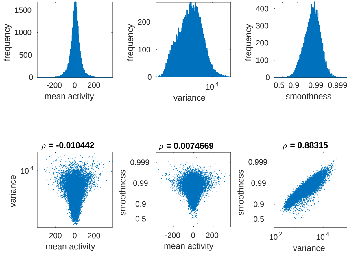
Extended Data Figure 2: Histograms and scatter plots of mean, variance, and time-resolved smoothness for a single representative recording. Note that variance and smoothness are log-transformed. \rho denotes the Spearman correlation coefficient.
