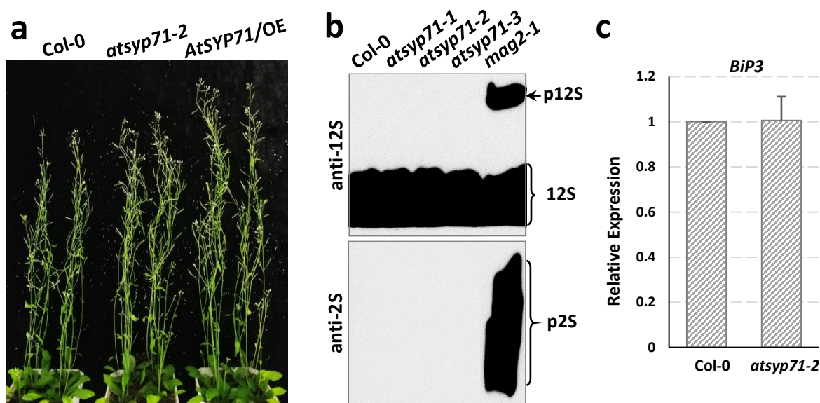
Fig. S1 Phenotypes of atsyp71-2 and AtSYP71/OE . a: 60-day-old plants of Col-0, atsyp71-2 and AtSYP71/OE . b: Detection of SSP precursors by immunoblot with anti-12S globulin and anti-2S albumin antibodies. The mag2-1 seeds were used as positive control. c: qRT-PCR detection of expression of BiP3 . 12S, pro12S globulin; p12S, precursors of 12S. p2S, precursors of 2S albumin.
