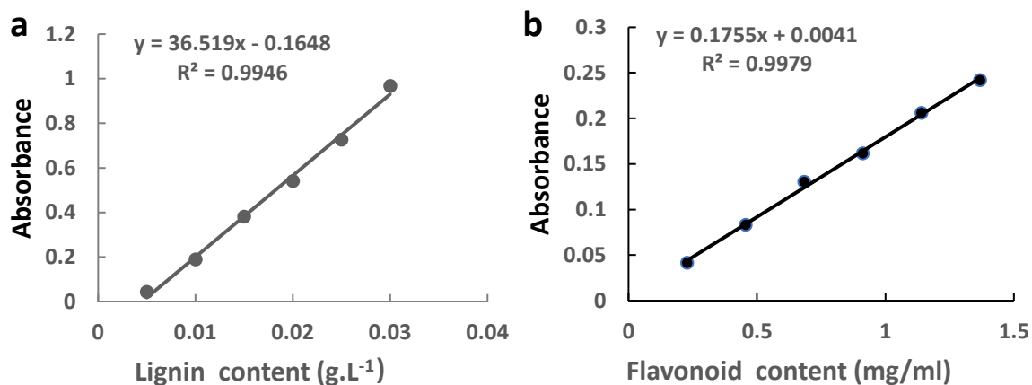
Fig. S2 Standard curves for lignin and flavonoids determination. a: Standard curve for determination of lignin content. b: Standard curve for determination of flavonoids content. Each measurement was repeated more than three times.
