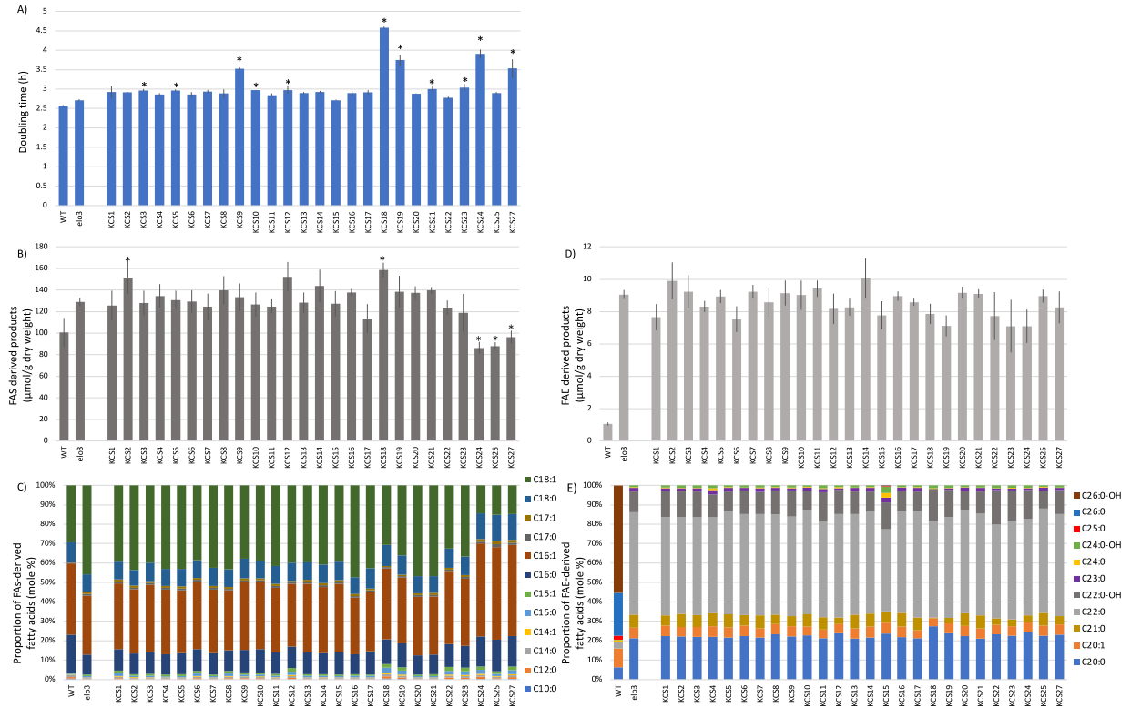
Supplementary Fig. 3. Growth rates and fatty acid profiling of scelo3 yeast strains expressing ZmKCS sequence. A) Culture doubling time. B) Yield of FAS-derived products. C) Proportion of individual FAS-derived products. D) Yield of FAE-derived products. E) Proportion of FAE-derived products. See Methods for details on data gathering and analysis. Fatty acid profiles were determined by either GC-MS analysis of FAMES. Error bars represent standard error from 3 replicates, and “*” identifies statistical significance from the recipient scelo3 strain, based on Student’s t-test ( p < 0.05 ).
