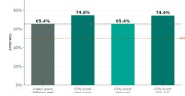
Fig. 2. The distance metric’s discrimination stated against its majority-class baseline. Raw accuracy is reported only alongside the baseline, because the pair set is imbalanced 524:992.
