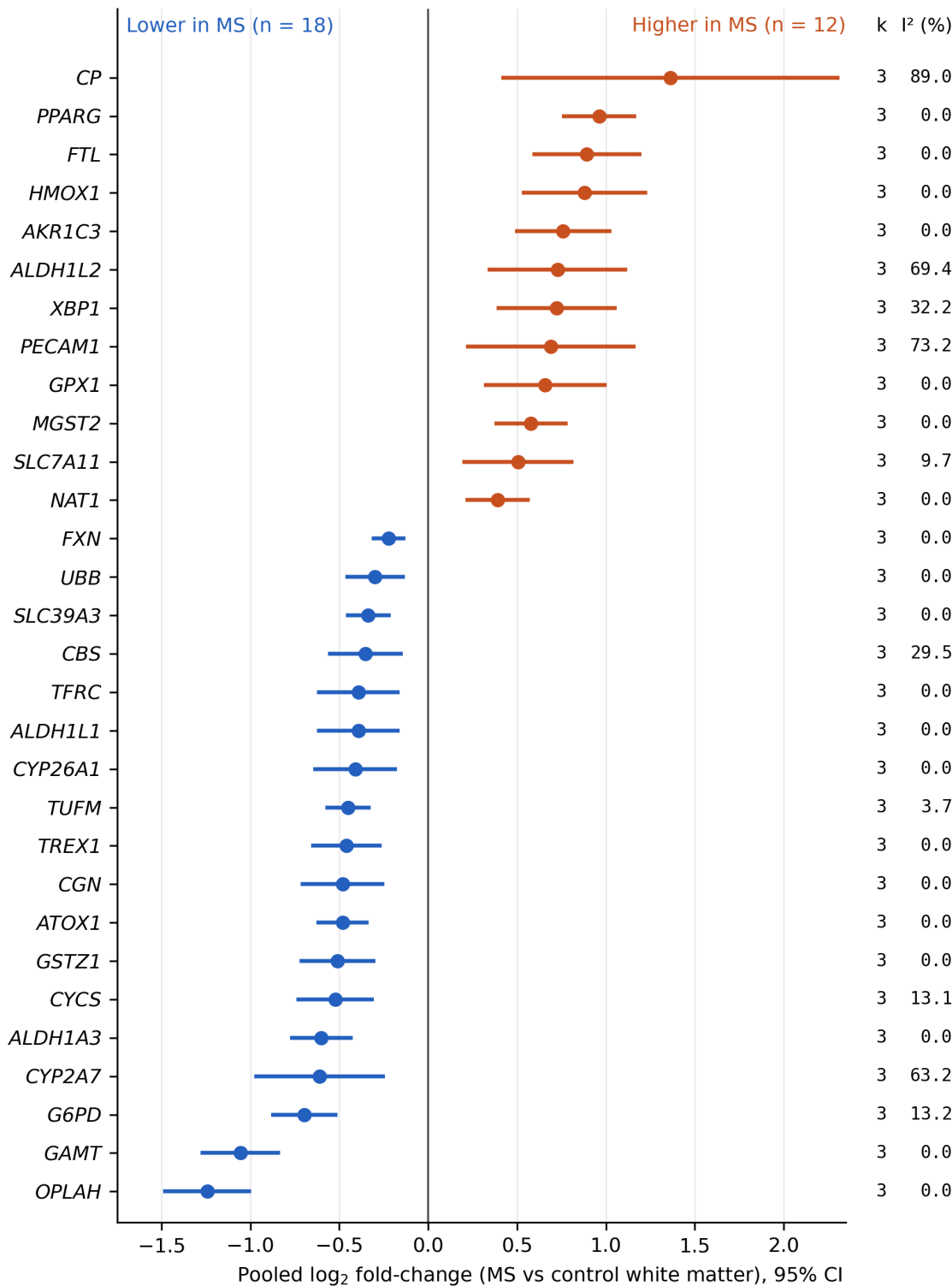
Figure 1 The 30 high-confidence genes of the three-cohort white-matter meta-analysis. Points are pooled log 2 fold-changes (MS vs control white matter; DerSimonian–Laird random effects across GSE138614, GSE32915 and GSE108000) and bars are 95% confidence intervals (pooled estimate \pm 1.96 \times \text{SE} ). Orange, higher in MS (n = 12); blue, lower in MS (n = 18). k (number of contributing cohorts) and I 2 are printed at the right of each row. High-confidence rule: FDR < 0.05, measured in \geq 3 cohorts, direction-
