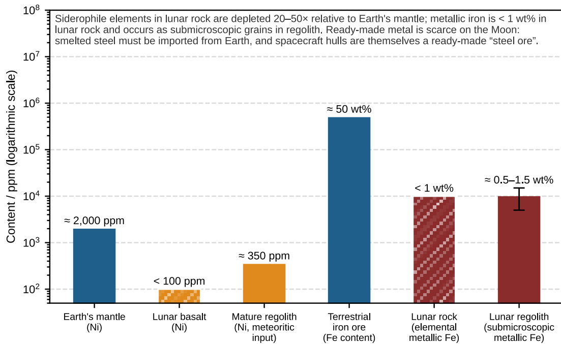
Fig. 13. Comparison of iron and nickel resources on the Moon and on Earth (schematic; order of magnitude of content from the literature 26 ).
