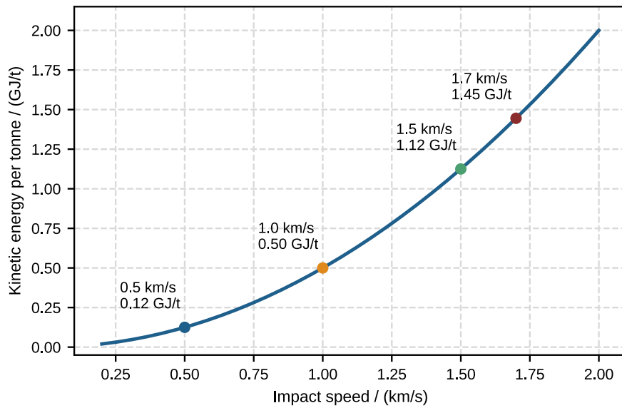
Fig. 8. Impact energy of an object in the near-vacuum environment of the lunar surface.
