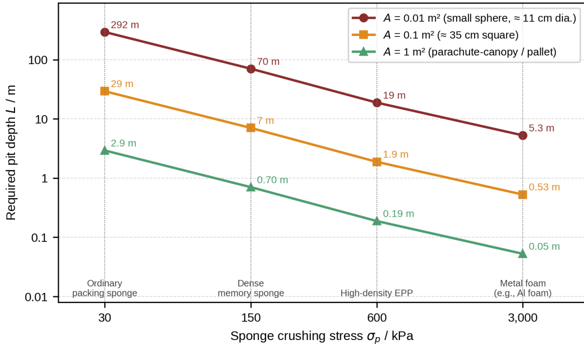
Fig. 10. Variation of pit depth with sponge stiffness and contact area (logarithmic coordinates); the idealized pit depth can be looked up according to the projected area of the actual item.
