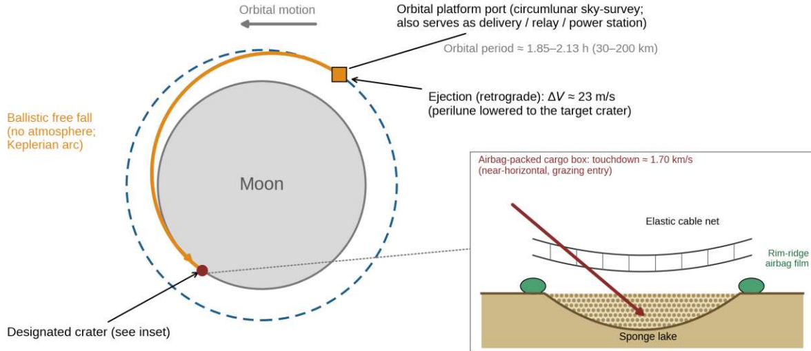
Fig. 7B. The grazing delivery trajectory enables the maximum buffering length along the inclined path of the lunar crater at the incidence angle into the sponge-lake.
