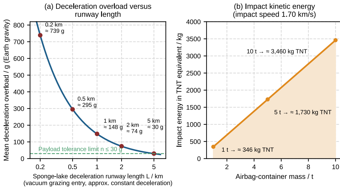
Fig. 9. Splashdown deceleration model: (a) deceleration overload versus energy-absorption scale; (b) impact kinetic energy of items of different mass.
