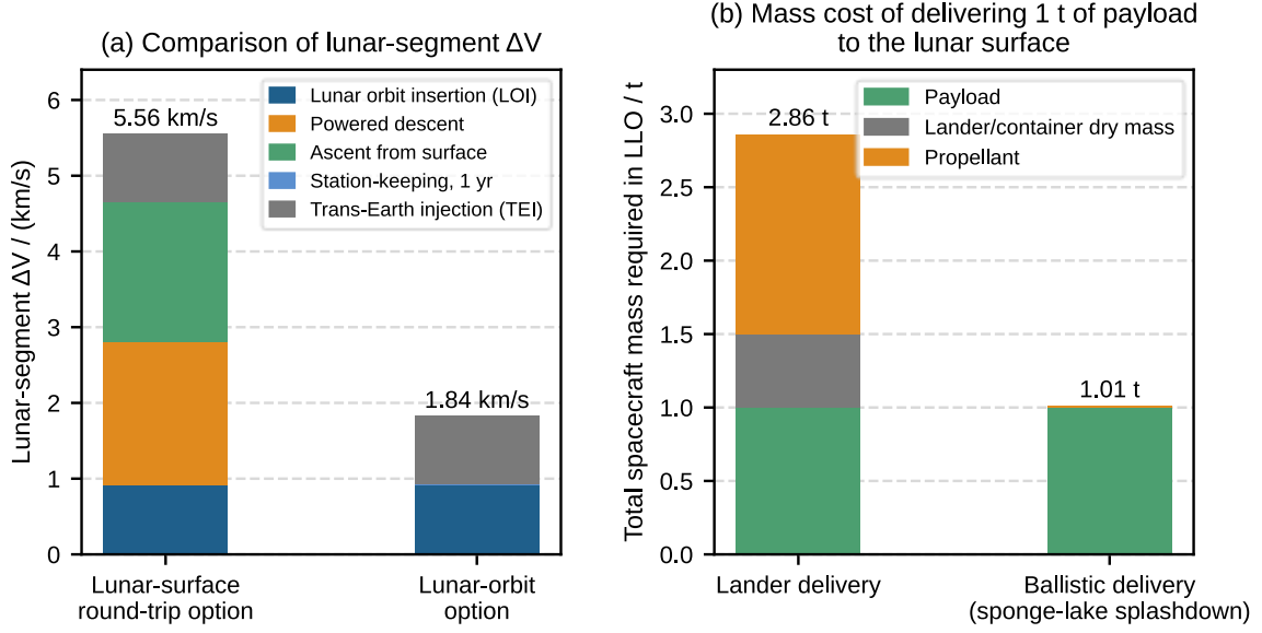
Fig. 1. Comparison of (a) the lunar-segment velocity increments of lunar-surface residence and circumlunar-orbit residence and (b) the mass cost of delivering 1 t of payload to the lunar surface.
