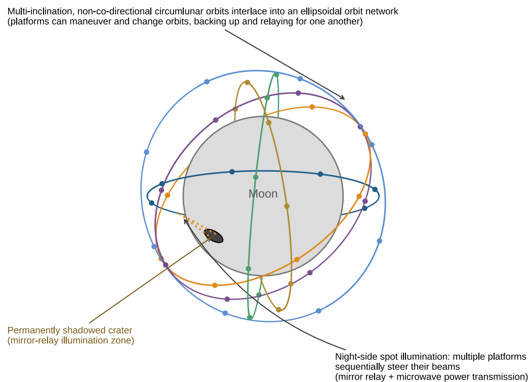
Fig. 12. Multi-platform circumlunar orbit network, with energy supply and illumination (schematic).
