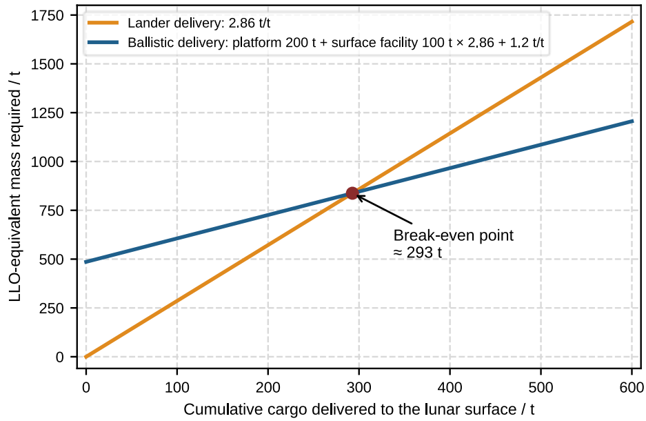
Fig. 6. Break-even of ballistic delivery relative to direct lander delivery (illustrative parameters: M_{\text{plat}} = 200 \text{ t} , M_{\text{inf}} = 100 \text{ t} , c_L = 2.86 , c_B = 1.2 ).
