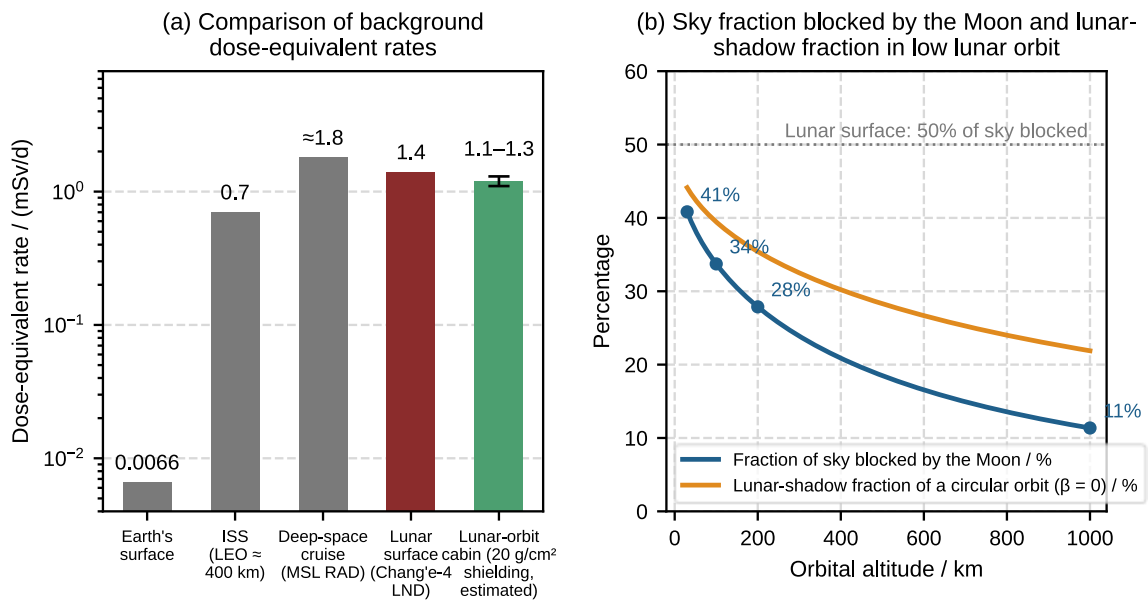
Fig. 4. (a) Comparison of background dose-equivalent rates; (b) fraction of the sky blocked by the Moon and lunar-shadow fraction in low lunar orbit (calculated in this paper; formulas in Appendix B).
