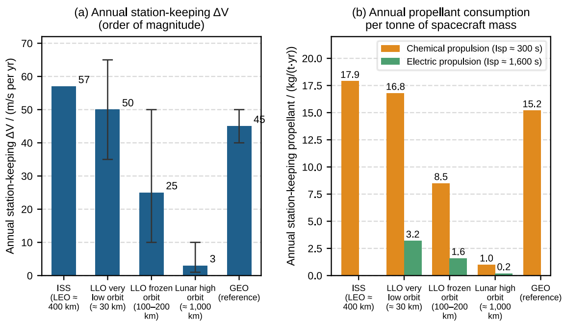
Fig. 5. Comparison of orbit-maintenance costs: (a) order of magnitude of the annual maintenance velocity increment; (b) annual propellant consumption per tonne of mass (calculated in this paper).
