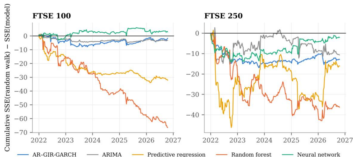
Fig. 5 Cumulative sum of squared forecast errors of the random walk minus those of each model, test period. A rising line indicates that the model is outperforming the random walk
