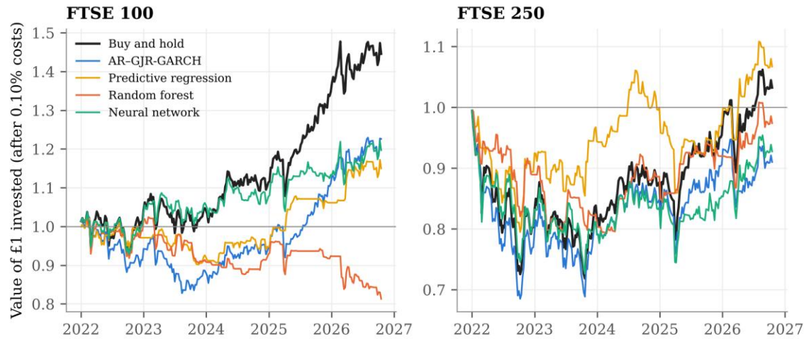
Fig. 7 Value of £1 invested in forecast-based strategies and in buy-and-hold, after 0.10% transaction costs, test period
