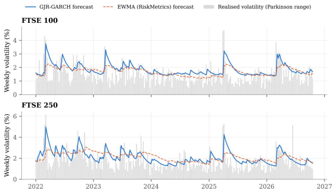
Fig. 6 Realised weekly volatility (Parkinson range estimator, grey bars) and one-week-ahead forecasts from the GJR-GARCH and EWMA models, test period
