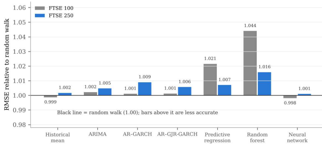
Fig. 4 Root mean squared error of weekly return forecasts relative to the random walk, test period. Values above 1 indicate a less accurate forecast than the random walk
