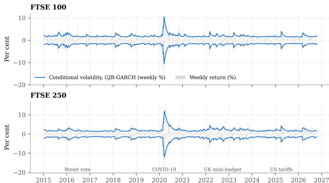
Fig. 2 Weekly returns (grey bars) and GJR-GARCH conditional volatility shown as \pm one conditional standard deviation, full sample
