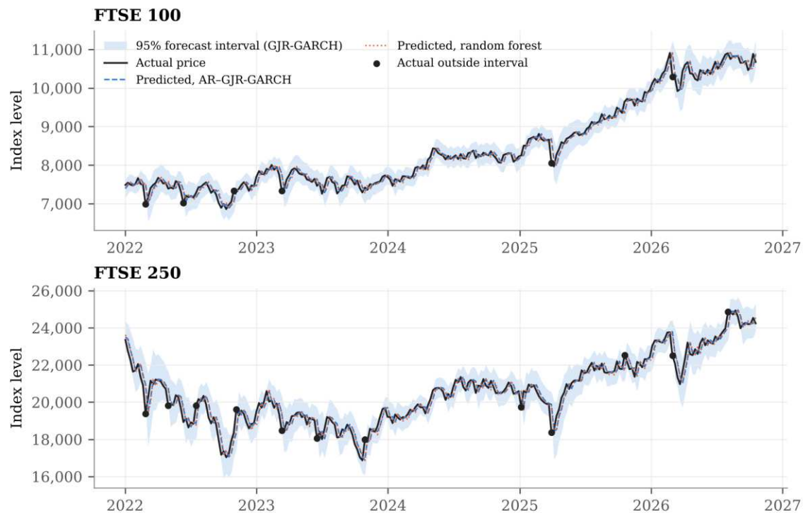
Fig. 3 Actual and predicted weekly index levels in the test period. The shaded band is the GJR-GARCH 95% forecast interval; dots mark weeks in which the actual price fell outside it
