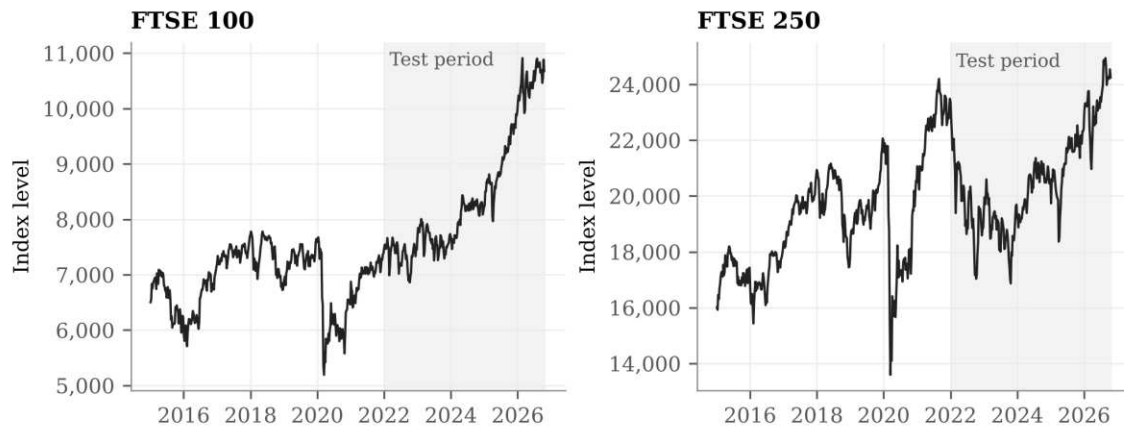
Fig. 1 Weekly closing levels of the FTSE 100 and FTSE 250, January 2015 to October 2026. The shaded area marks the out-of-sample test period
