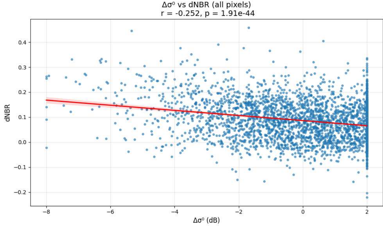
Figure 7: \Delta\sigma^0 vs dNBR correlation across all pixels
