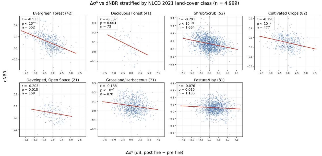
Figure 9: \Delta\sigma^0 vs dNBR Correlation Stratified by Land Cover
