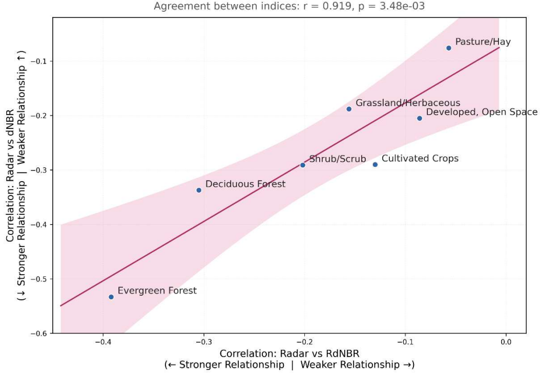
Figure 11: Correlation comparison across radar and optical analyzed data
