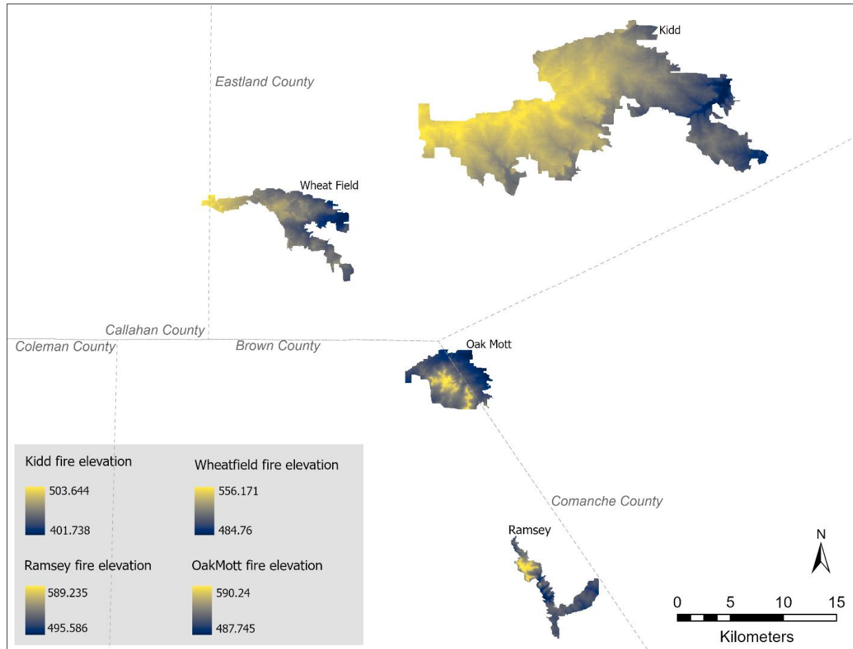
Figure 16: Elevation difference in the study area
