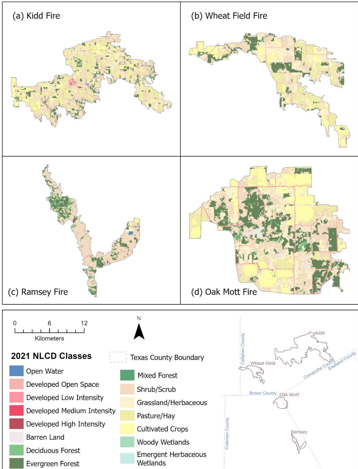
Figure 1: Study area with National Land Cover Database (NLCD) map overlay on Google Earth Engine and county perimeter
