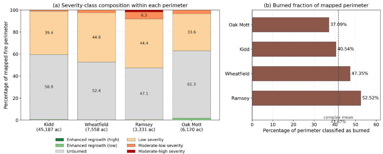
Figure 6: Quantitative comparison of burn severity among the four fires. (a) Severity-class composition as a percentage of each mapped perimeter; (b) percentage of each perimeter
