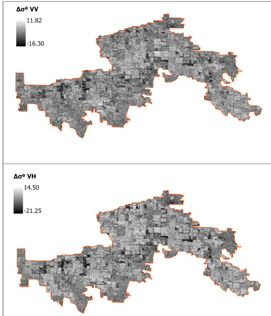
Figure 3: Radar backscatter change in the study area. Only Kidd fire is shown here for example. Next figure provides detailed understanding.
