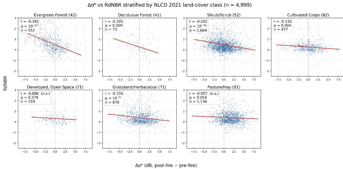
Figure 10: \Delta\sigma^0 vs RdNBR correlation stratified by land cover
