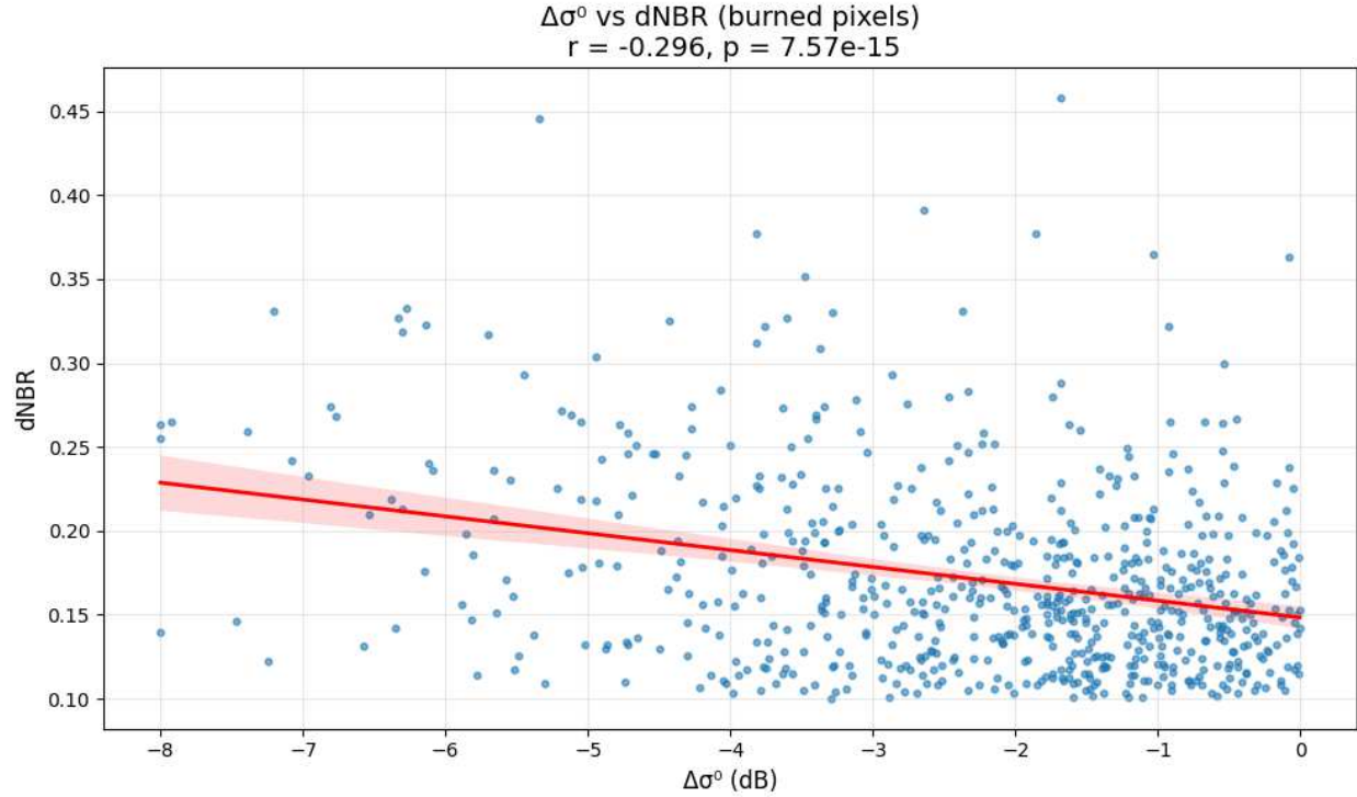
Figure 8: \Delta\sigma^0 vs dNBR correlation for burned pixels only
