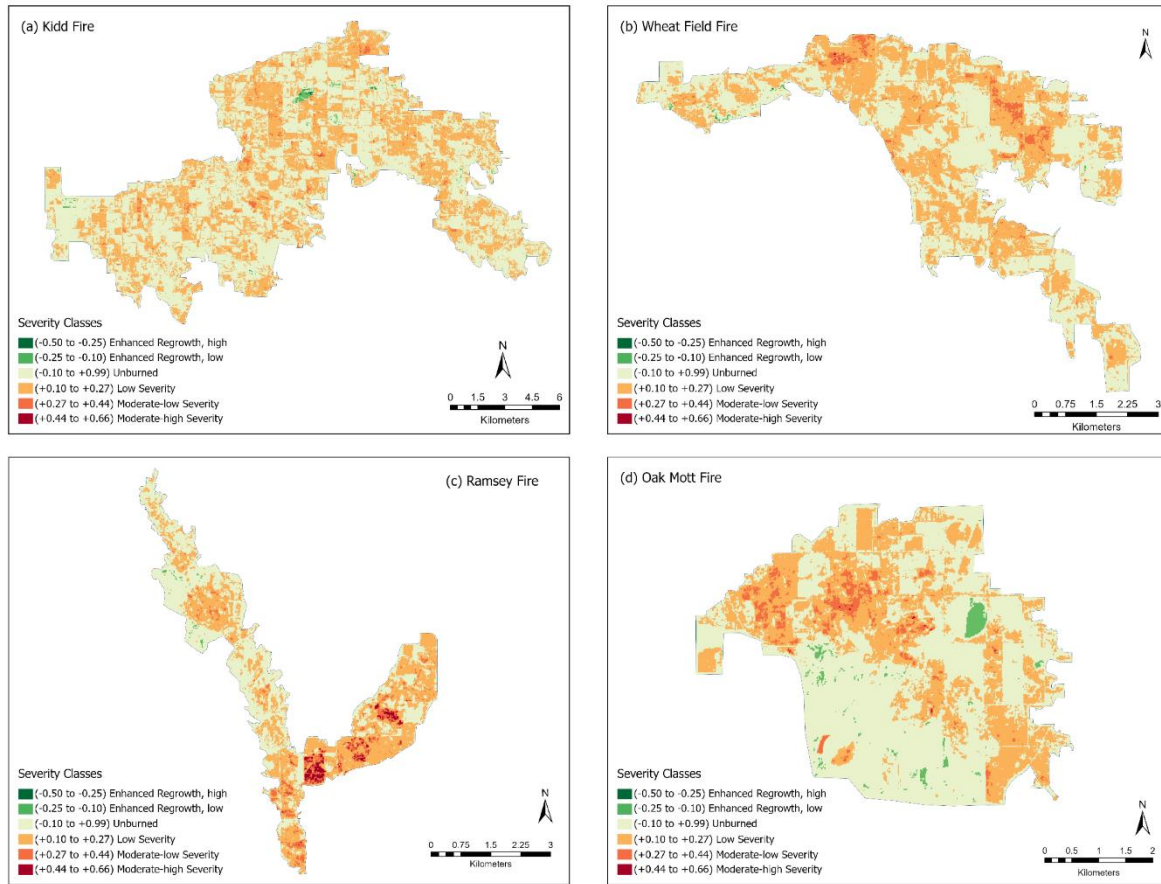
Figure 5: Sentinel-2 dNBR burn-severity classification for the four fires of the Eastland Complex: (a) Kidd, (b) Wheatfield, (c) Ramsey and (d) Oak Mott. Severity classes follow the dNBR ranges of Table 2. Panels are shown at individual scales; each carries its own scale bar.
