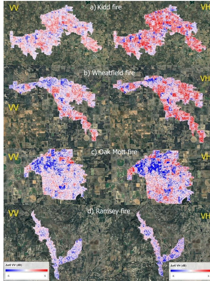
Figure 4: SAR Backscatter change spatial pattern. Backscatter values were speckle-filtered using a Lee-type adaptive filter in linear power space and differenced in decibel units, preserving the physical magnitude of change.
