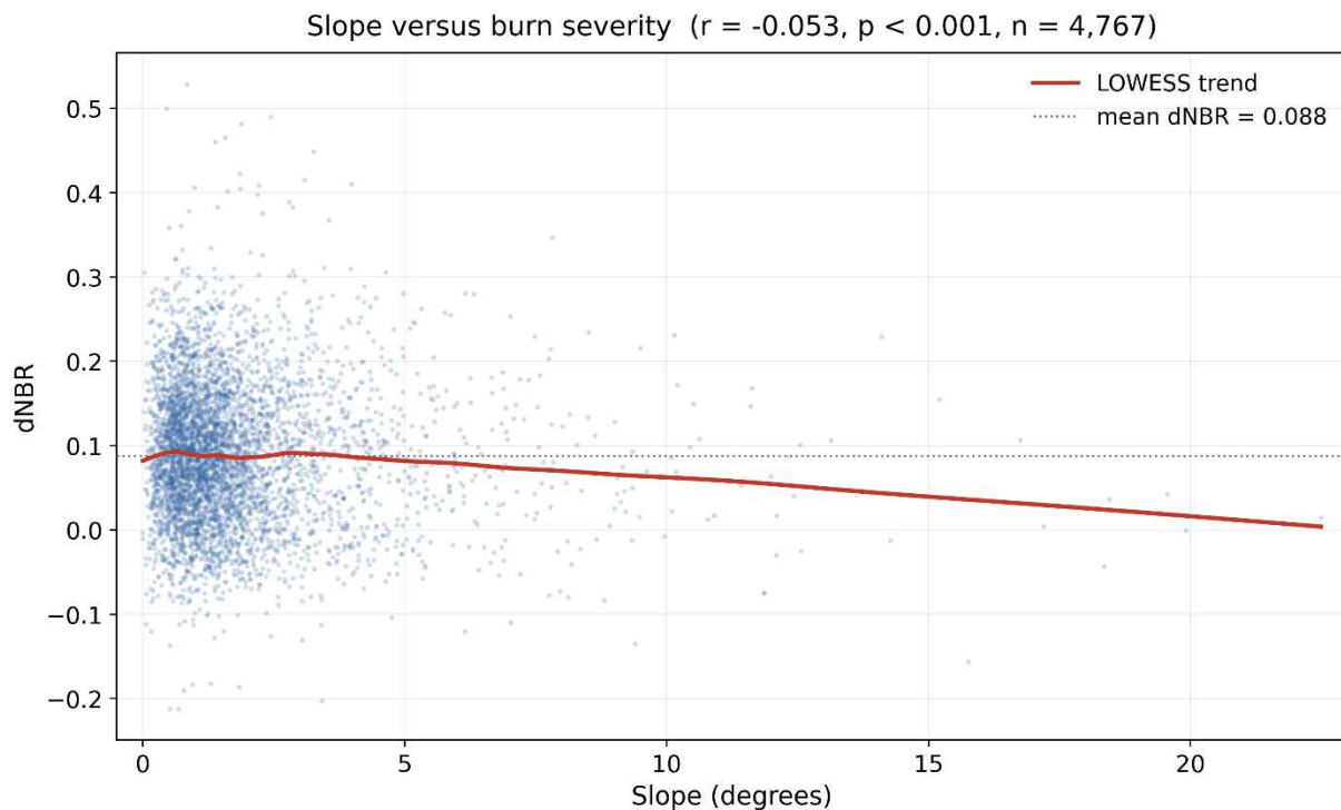
Figure 14: Locally weighted scatterplot smoothing (LOWESS) trend of slope versus dNBR
