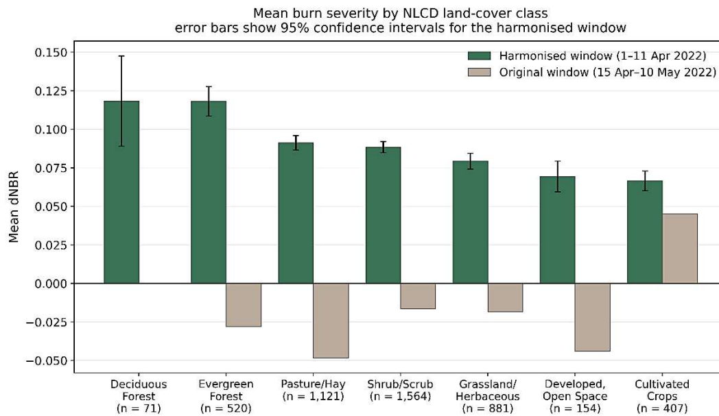
Figure 15: Mean-dNBR by NLCD class for only burned pixels
