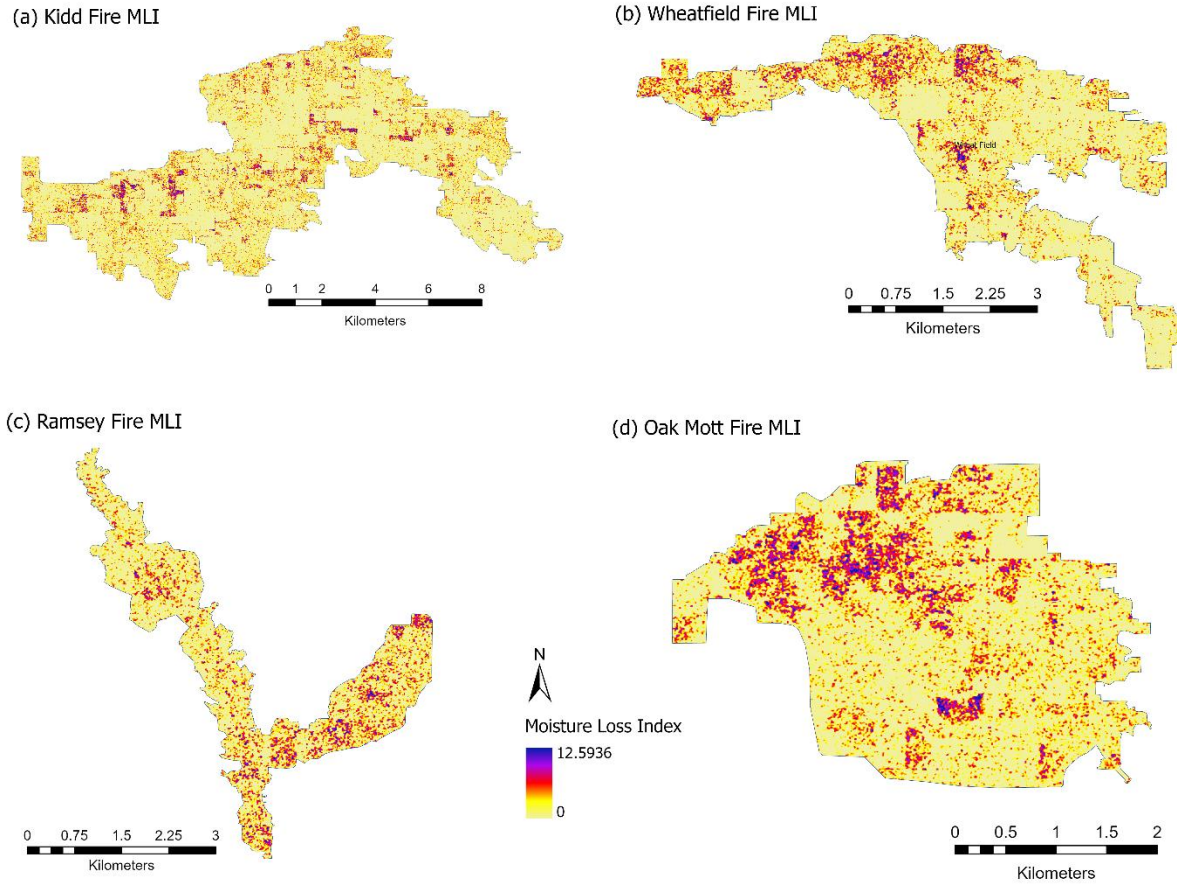
Figure 13: Moisture Loss Index (MLI) map, legend has been scaled to highest MLI for visualization
