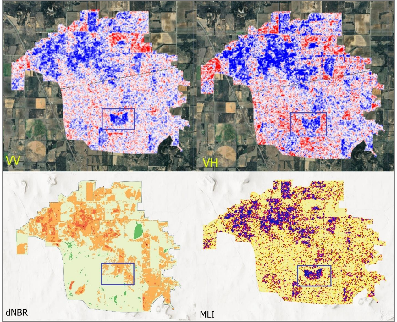
Figure 17: Comparative analysis among spatially mapped radar derived backscatter change data, moisture loss index and sentinel-2 derived burn severity map
