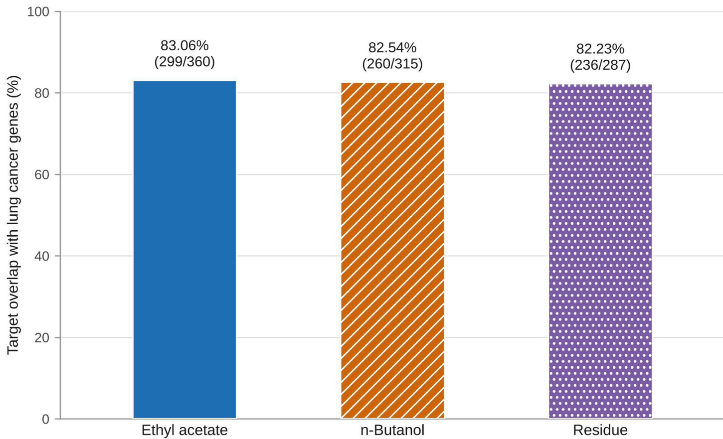
Figure 2 Percentage overlap between each solvent fraction's predicted target set and lung cancer-associated genes
