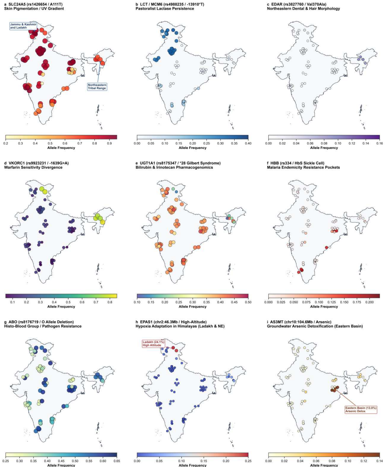
Extended Data Fig. 5 | Geographical allele frequency variations of selective sweep and pharmacogenomic loci across the Indian political map (incorporating full Jammu & Kashmir and Ladakh). Multi-panel spatial maps plotting allele frequencies across all 82 indigenous Indian populations on the official Survey of India sovereign political boundary (spanning from latitude 6.8°N at Indira Point to 37.1°N at Indira Col, Ladakh; and longitude 68.2°E to 97.4°E, enclosing all of Jammu, Kashmir, Ladakh, Aksai Chin, and Arunachal Pradesh). a , SLC24A5 rs1426654 (A111T) skin pigmentation cline showing peak frequencies in the Western Himalayas (>88% in Jammu, Kashmir, and Ladakh) and Northwestern plains,
