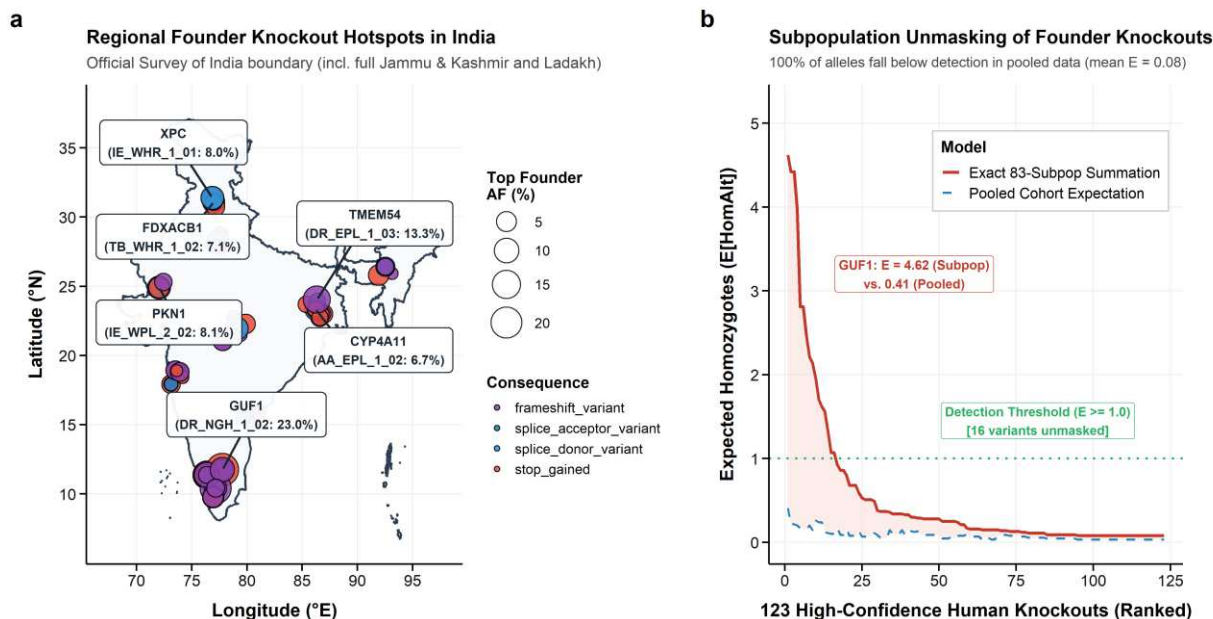
Fig. 6 | Geographic distribution of regional founder knockout hotspots and subpopulation recovery of 123 loss-of-function genes. a , Geographic bubble map plotted on the official Survey of India political boundary (incorporating the full territory of Jammu & Kashmir and Ladakh up to 37.10° N), displaying regional founder knockout hotspots across 10 agro-ecological zones and annotating top representative founder knockouts ( GUF1 23.0% in Nilgiri Hills Dravidian tribal community (DR_NGH_1_02), TMEM54 13.3% in Eastern Plateau Dravidian tribal community (DR_EPL_1_03), PKN1 8.1% in Western Plains Rajasthani non-tribal community (IE_WPL_2_02), XPC 8.0% in Western Himalayan tribal isolate (IE_WHR_1_01), FDXACB1 7.1% in Western Himalayan Tibeto-Burman tribal community of Ladakh (TB_WHR_1_02), and CYP4A11 6.7% in Eastern Plateau Austroasiatic tribal community (AA_EPL_1_02)). b , Comparison of expected homozygous alternate carrier counts under pooled national analysis ( E_{\text{pooled}} < 1.0 , mean 0.08) versus exact subpopulation summation (Total_Subpop_E_HomAlt, peaking at 4.62 in GUF1 and 4.42 in PAICS , with 16 founder alleles exceeding E_{\text{subpop}} \geq 1.0 , and top founder population expectations peaking at 4.02 in GUF1 with 14 alleles \geq 1.0 ) across all 123 empirically observed human knockout variants (Obs_HomAlt \geq 1 , totaling 144 homozygous knockout individuals; Supplementary Table S11).
